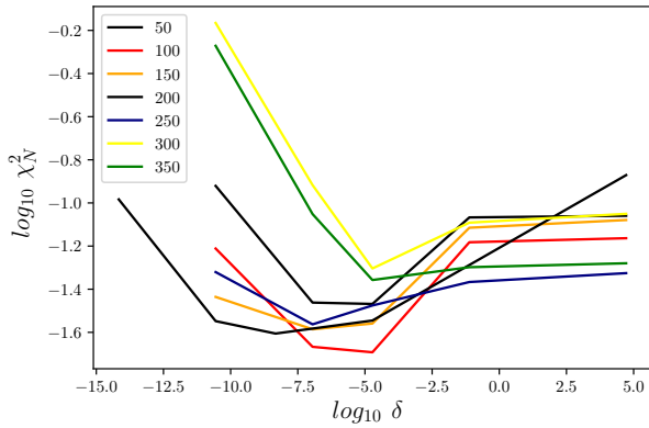
Fig. 3. \log_{10}(\chi^2_N) versus \log(\delta) for T_{\text{eff}} of a synthetic spectra having T_{\text{eff}}=7600 K, \log g=2.50 dex, v \sin i=197 km s ^{-1} , and with a S/N of 196. Each curve displays the minimization using different sets of nearest neighbor generated iteratively.
