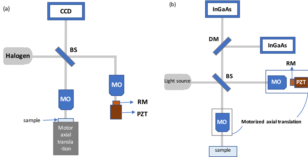
Figure 25. Schematic of (a) the ultrahigh-resolution full-field OCT setup [7] and (b) the experimental setup of FF-OCM [86]. MO, microscope objective; BS, beam-splitter cube; DM, dichroic mirror; PZT, piezoelectric actuator.
