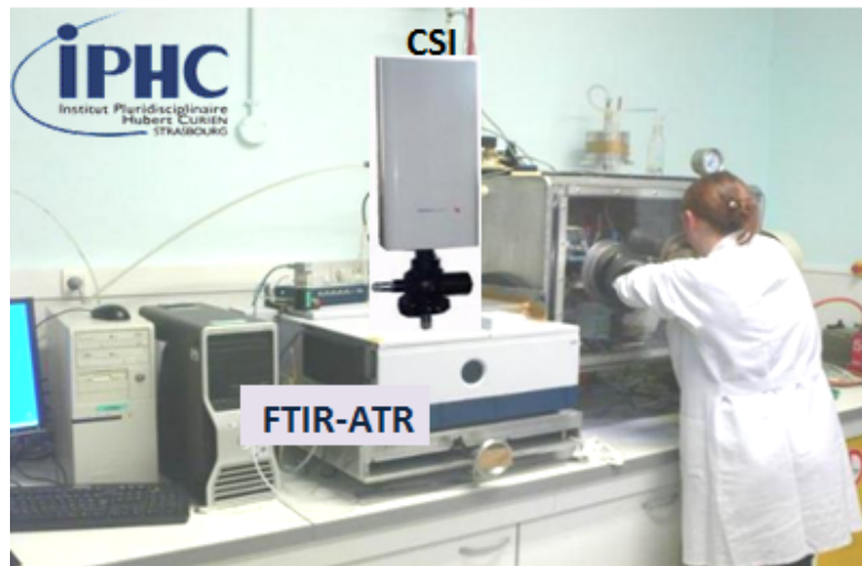
Figure 29. Illustration of combining CSI technique and ATR-FTIR.
