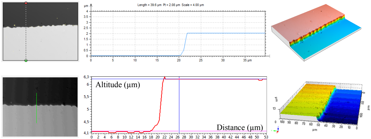
Figure 86. 2 \mu\text{m} high Al step on Si is measured by (first row) the Zygo microscope in air ( \times 50 Mirau, \text{NA}=0.55 ); and (second row) the Fogale Linnik immersion system ( \times 20 , \text{NA} = 0.5 , 0.05 \mu\text{m} step height, 13 dynamic range, \lambda_{eff} = 450 \text{ nm} , rectify, [4644]).
