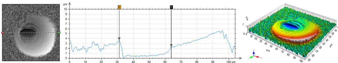
Figure 108. Etched Silicon on oval pattern measured by \times 20 immersion Linnik Fogale microscope using a 7 \mu\text{m} BTGMS microsphere on it (0.05 step height, 15.5 dynamic range, \lambda_{eff} = 450 \text{ nm} , [4675b]).
