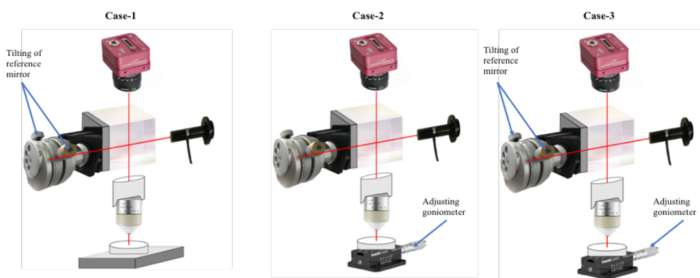
Figure 90. Description of three cases to test and observe the effect of misalignment.
