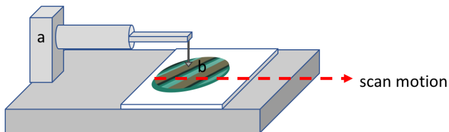
Figure 1. Schematic of stylus profiler with LVDT as the motion detector. Part a is a fixed stylus with LVDT assembly and b is a sample.
