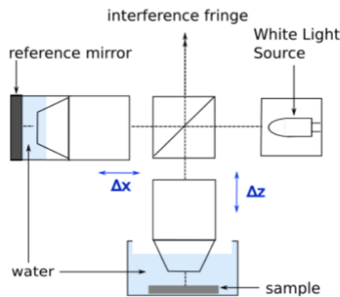
Figure 23. Configuration of a Linnik water-immersion objective.
