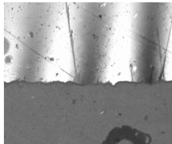
Figure 74. Fringe image of Al step on Si using white light, \times 20 immersion Linnik objectives in water (0.05 \mu\text{m} step height, 12 dynamic range, \lambda_{eff} = 640 nm, [4634-5]).
