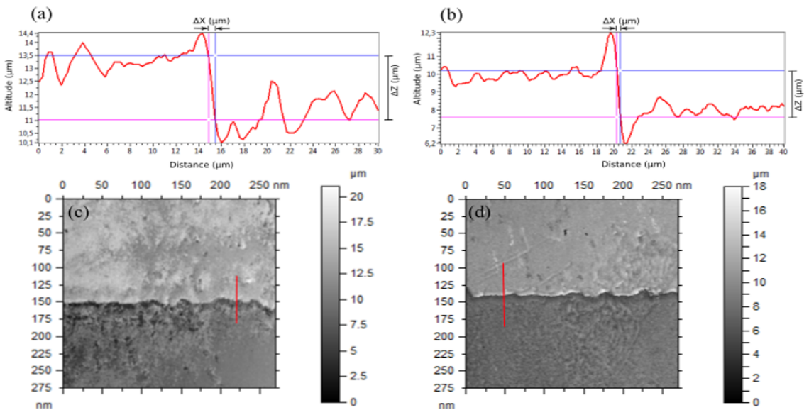
Figure 70. Comparison of line profiles of the measured height of the Al step on Si using the 40\times immersion Linnik head in air (shown in (a) and (c)) and in water (shown in (b) and (d)). The measurements of the step height ( \Delta Z ) of the sample are 2.49 \mu\text{m} (0.05 step height, 18 dynamic range, \lambda_{eff} = 640 \text{ nm} , [4585]).
