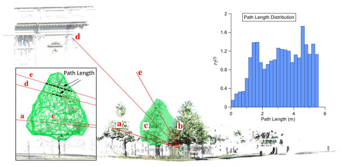
Fig. 4.8 Illustration of laser pulses, gap probability and path length calculation for the studied tree using its envelope. Approximately 43% of the studied tree (green) is visible from TLS station in the illustration. Emitted laser pulses are classified into 5 types: a - do not intersect the tree crown envelope, b – blocked by the objects in front of the tree. c – intersect within the tree crown envelope and have a return within the envelope, d – pass through the envelope and have a return behind the tree, e – pass through the envelope and have no return. Only emitted laser pulses c, d, and e are used to calculate the gap probability and path length distribution within the tree crown.
