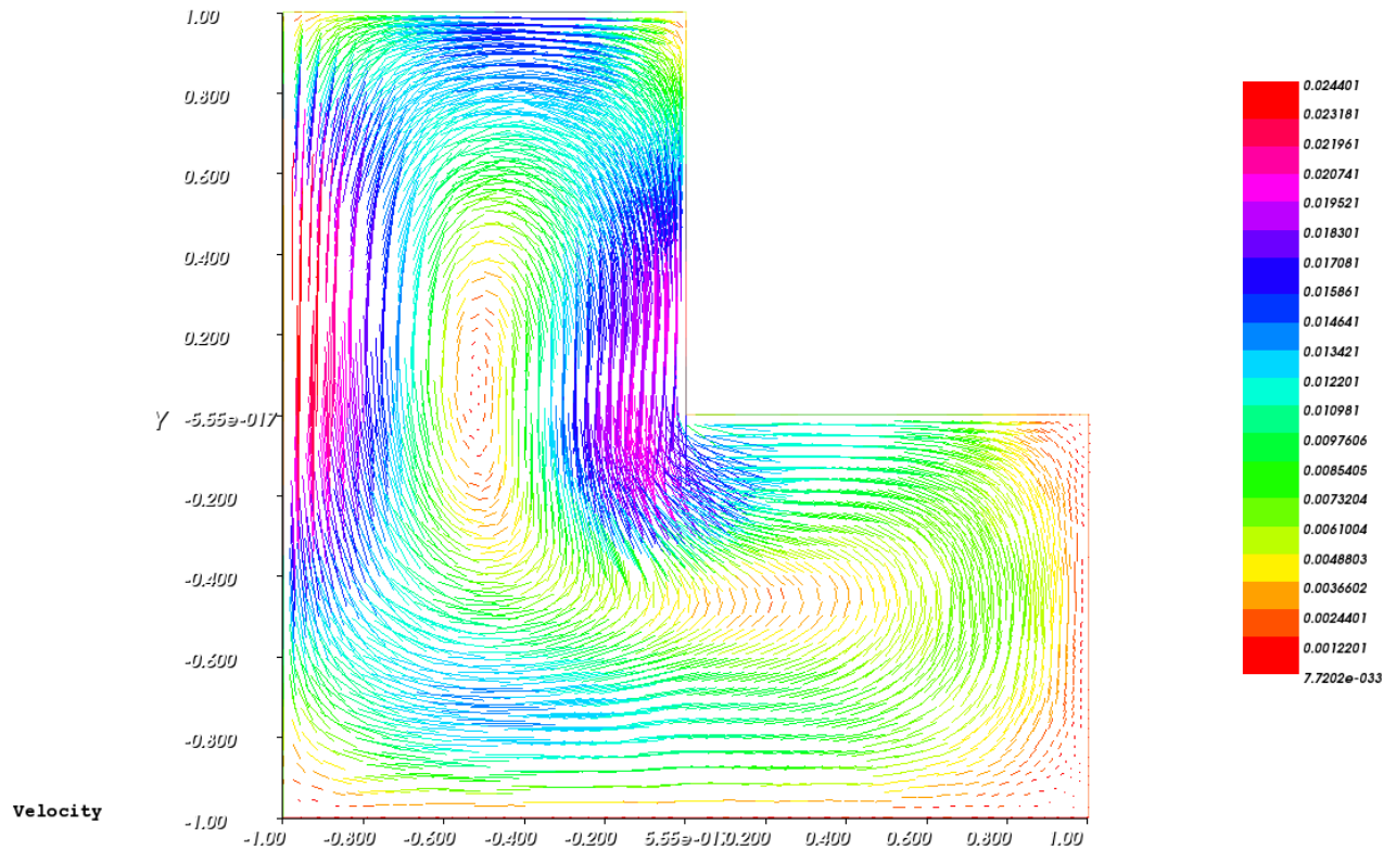
Figure 2: Contour plots of the approximated velocity components.
