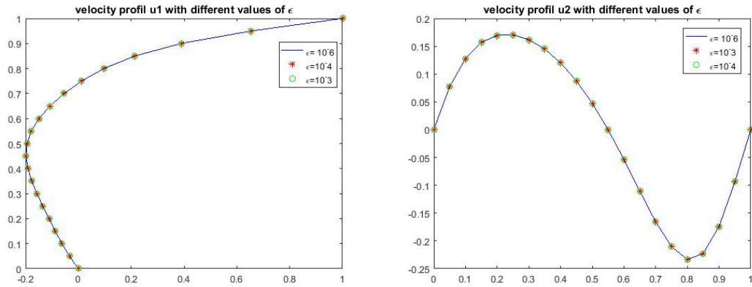
(a) x direction velocity component along the vertical centreline component. (b) y direction velocity component along the horizontal centreline component.
