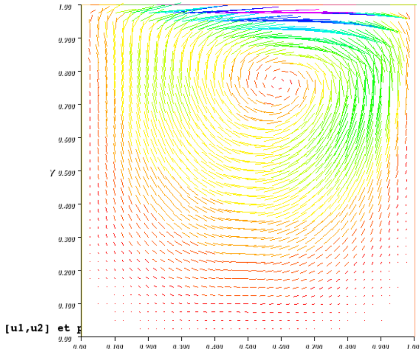
Figure 1: velocity vector in driven cavity.
