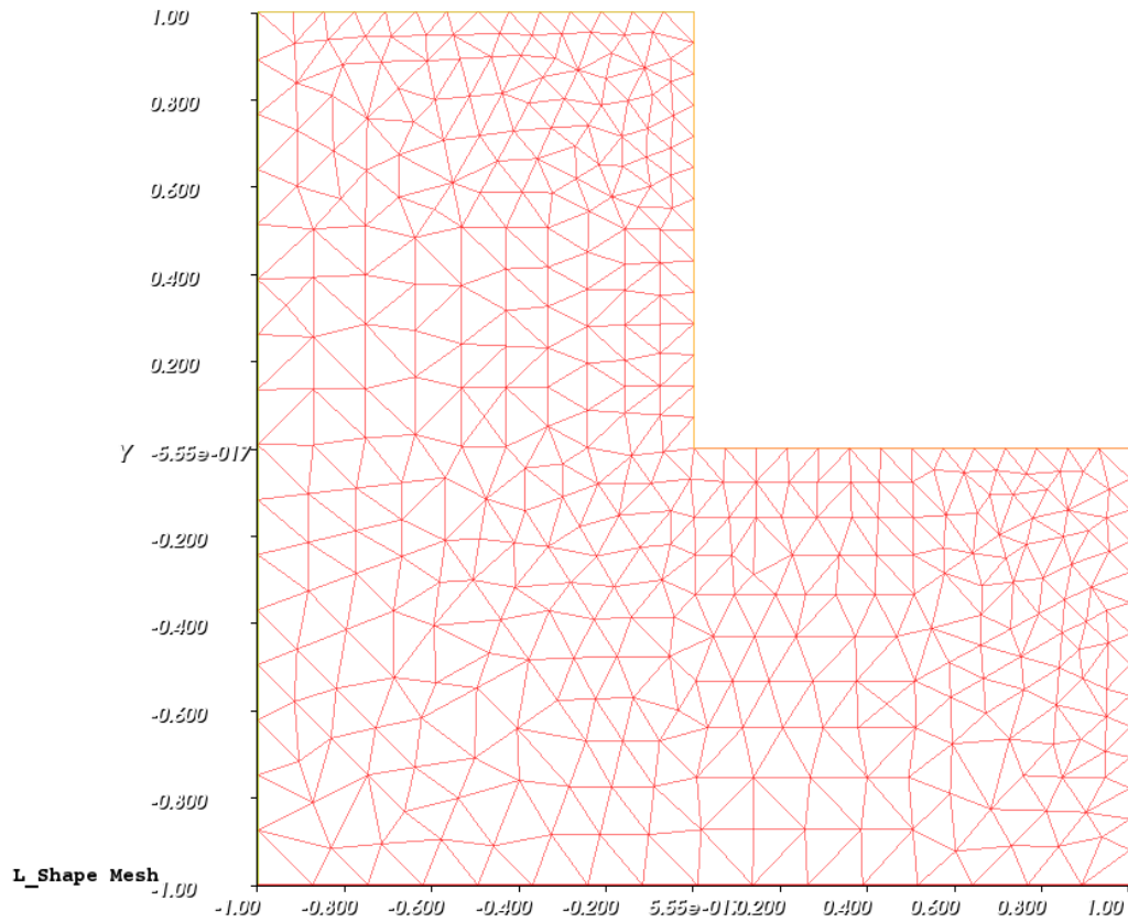
Figure 1: L shape geometry.
