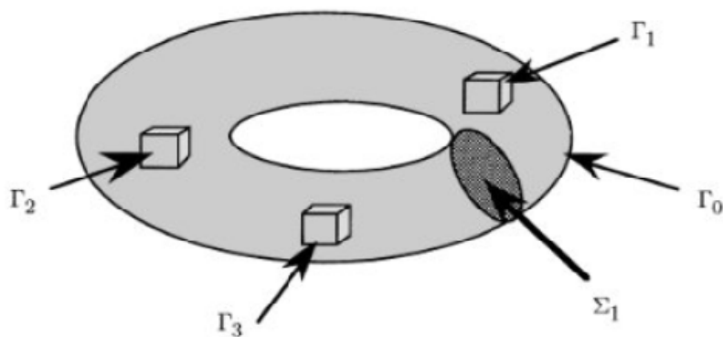
Figure 1: The domain \Omega
