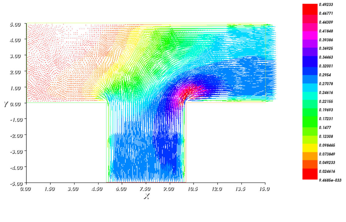
Figure 4: Velocity in a two-dimensional T-shaped bifurcation with Re = 40 and the imposed pressure on the inlet and outlet boundaries.
