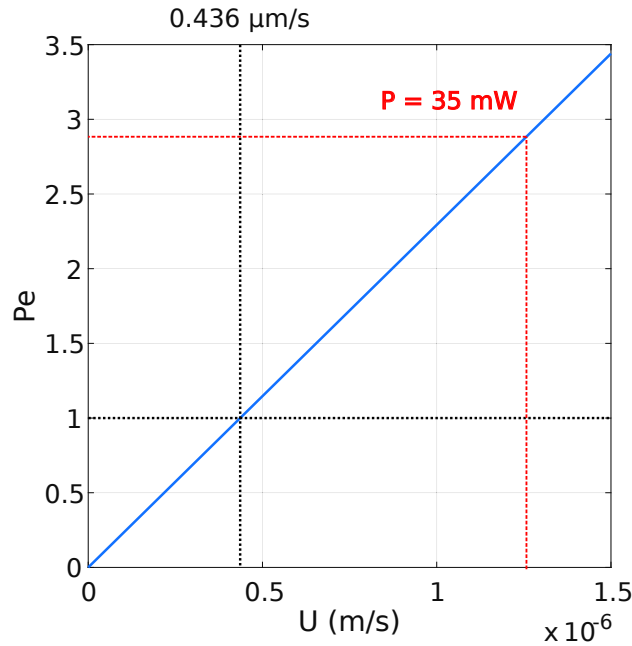
Figure 3.21 – Dependence of Peclet number on the flow velocity. When the flow velocity exceeds 0.436 \mu\text{m/s} , the advective motion starts dominating over the the diffusive motion. The red dotted line correspond to our experimental regime of induced convection with P_{\text{High}} = 35 \text{ mW}
