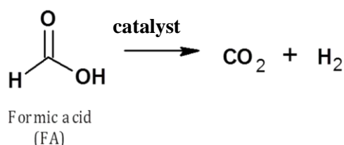
Figure 23. Reaction scheme of selective formic acid decomposition.
