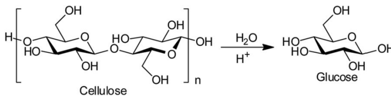
Figure 3. Scheme of acid catalyzed hydrolysis of cellulose.
