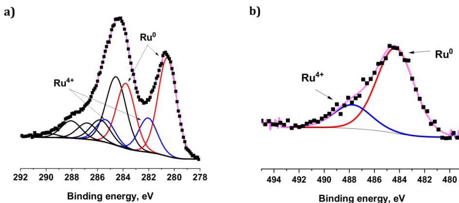
Figure 41. a) Ru 3d + C 1s ; b) Ru 3p XPS profile of the Ru(5 wt.%)/TiO 2 -P25 catalysts. No presence of any residual chlorine species was observed by XPS at the surface of TiO 2 when the chloride precursor was used (Cl 2p XPS spectra not shown).
