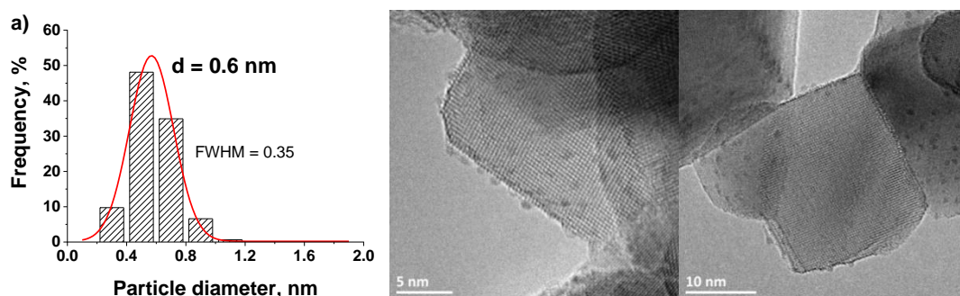
Figure 4. TEM images and the corresponding histograms of the Ru nanoparticle size distribution for 0.5%Ru_acac P25 catalyst.
