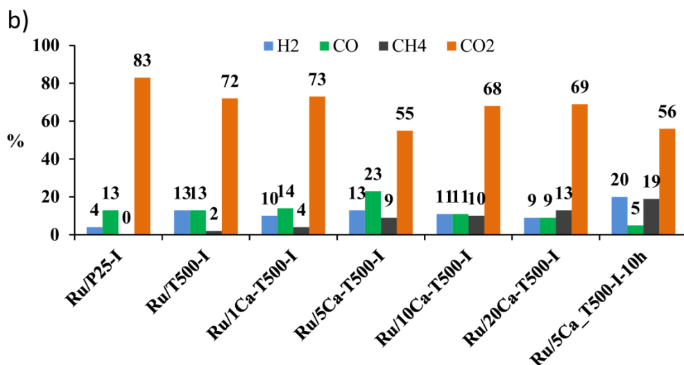
Figure 53. Catalytic activity of the Ru catalysts prepared by the impregnation method in the FALA reaction, in terms of a) LA hydrogenation, FA decomposition and GVL yield; and b) Gaseous product distribution; [1 g of LA, 0.4 ml of FA, 0.6 g of catalyst, 30 ml of H 2 O, 190 °C, 5 h].
