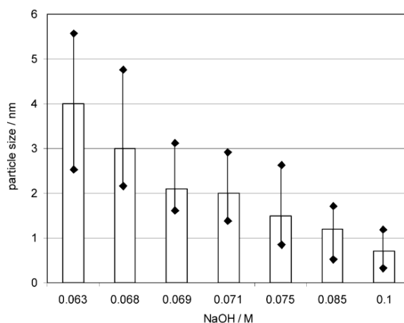
Figure 17. Average particle size dependence on the NaOH concentration in the ethylene glycol synthesis solution. 171
