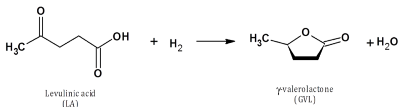
Figure 1. Reaction scheme of LA hydrogenation with internal hydrogen source.
