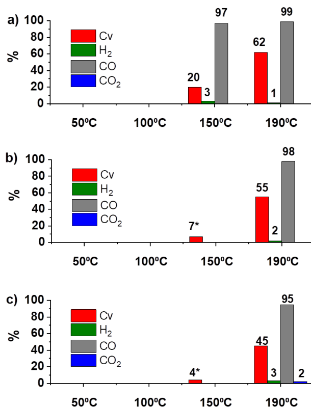
Figure 59. Catalytic activity of different TiO 2 support materials in gas phase formic acid decomposition: decomposition: a) Hombikat UV100 (320 m 2 /g); b) ST01 (310 m 2 /g); c) Aeroxide P90 (90 m 2 /g); [0.02 g of catalyst, 17000 ppm of FA, 1 h at each temperature, Ar flow 30 ml/min].
