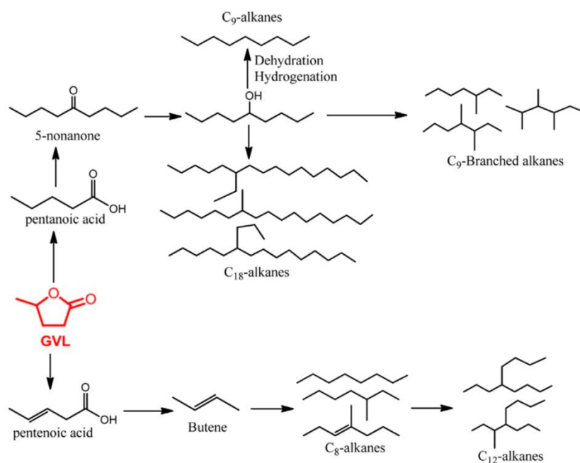
Figure 13. Routes for the transformation of GVL into liquid alkanes. 65
