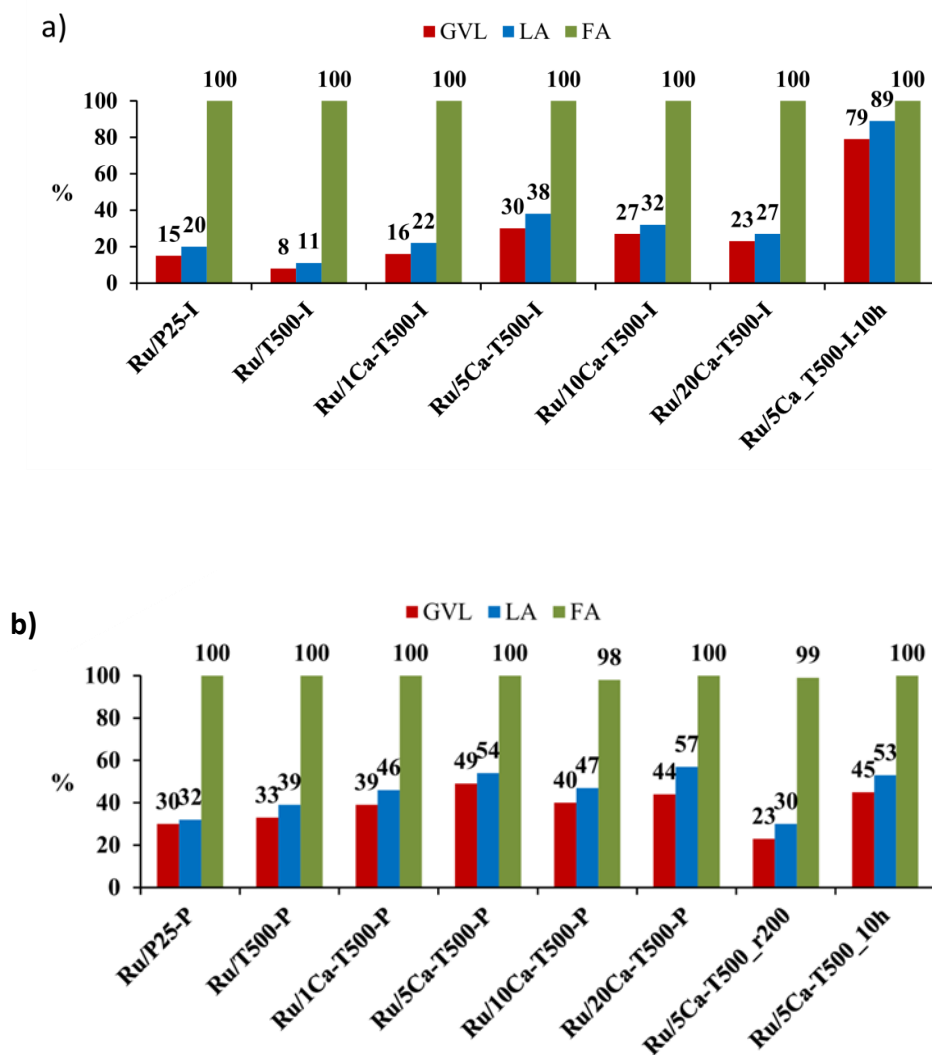
Figure 7. Catalytic activity of the Ru catalysts a) prepared by wet impregnation and b) prepared by photodeposition method in the FALA reaction.
