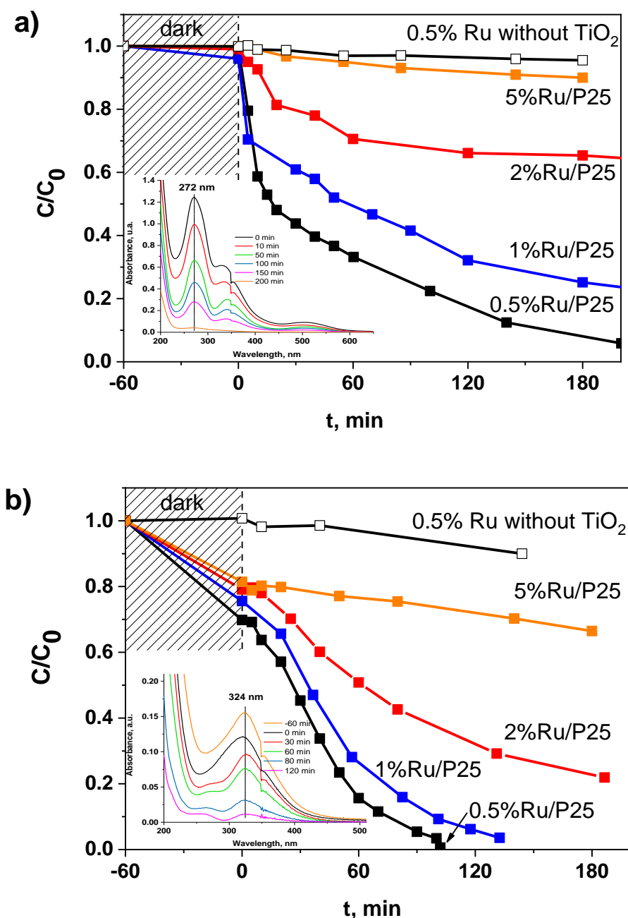
Figure 31. Disappearance of the Ru precursor in the presence of TiO 2 P25 as a function of the illumination time for a) \text{Ru}(\text{acac})_3 and b) \text{RuCl}_3 precursors, with a Ru content of 0.5, 1, 2 and 5 wt. %. Inset: Examples of UV-vis absorbance spectra evolution as a function of the illumination time during the photo-assisted synthesis.
