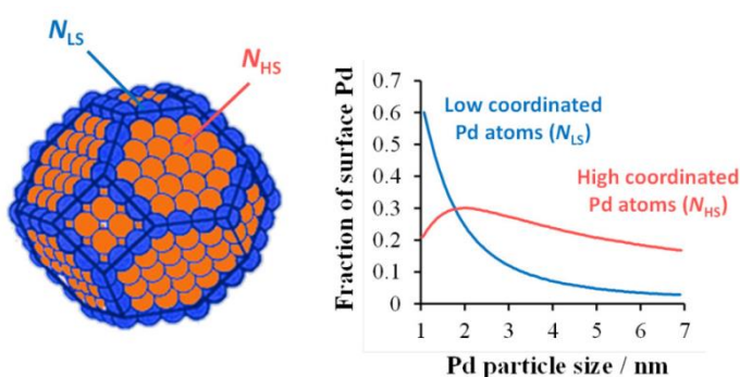
Figure 16. Schematic illustration of high-coordinated and low-coordinated atoms and their fraction of surface area. 163
