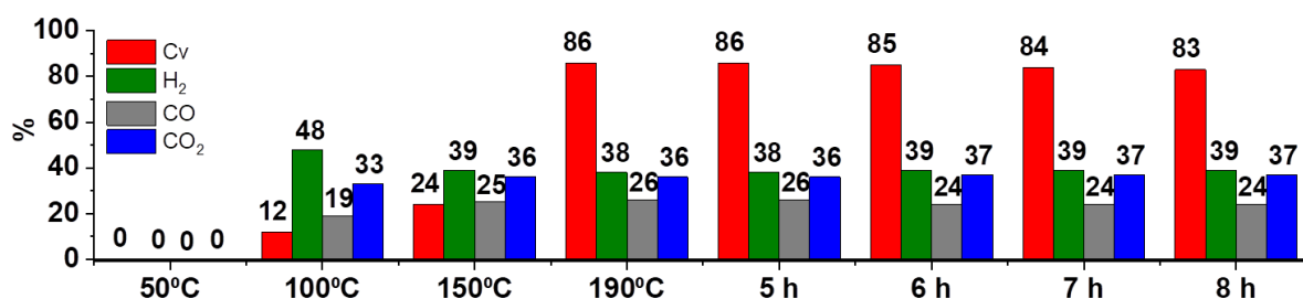
Figure 64. Catalytic activity of 5%Ru/1Ca-T500-P in the extended reaction run of gas phase formic acid decomposition; [0.02 g of catalyst treated under H 2 at 50°C for 30 min, 17000 ppm of FA, 1 h at each temperature + 4 additional hours at 190°C, Ar flow 30 ml/min].
