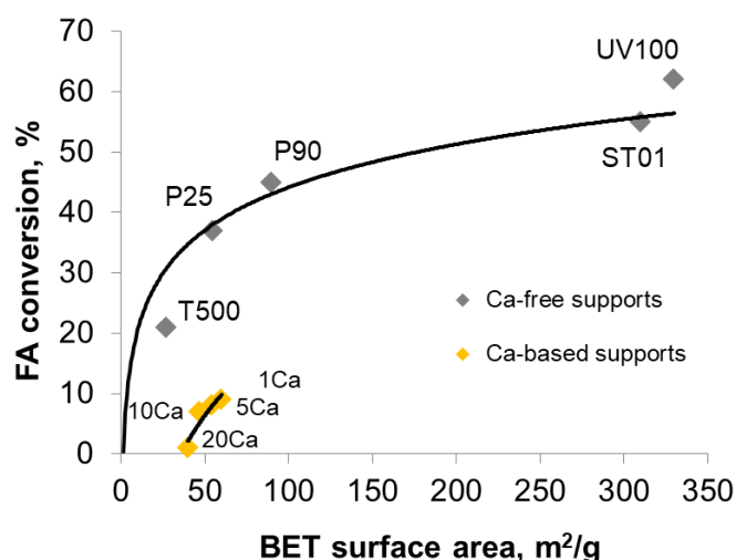
Figure 9. FA conversion obtained on the \text{TiO}_2 and the Ca-modified \text{TiO}_2 support materials in the gas phase formic acid decomposition at 190^\circ\text{C} as a function of the BET specific surface area.
