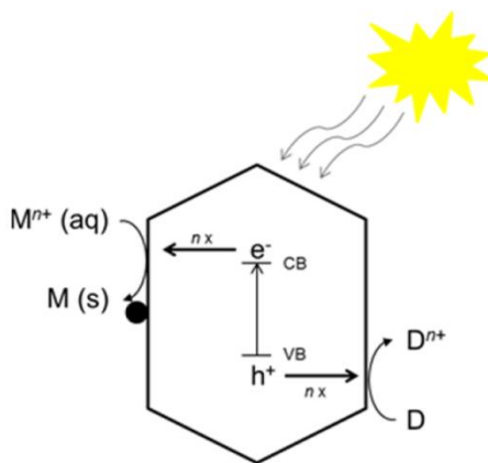
Figure 18. Schematic overview of a reductive photodeposition; VB- valence band; CB - conduction band; M -metal; D - electron donor; n - number of electrons (or holes) involved.
