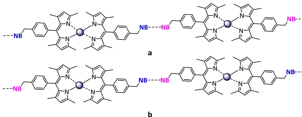
Figure 21: An example of a supramolecular network that could form via H-bonding interactions between (a) two complementary homoleptic bisdipyrin complexes or (b) a heteroleptic self-complementary bisdipyrin complex.
