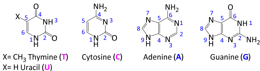
Figure 33: DNA nucleobases
