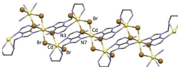
Figure 49: The X-Ray structure of the polymeric chain of [\text{Cd}_2\text{Br}_6(\text{A-Et-en})_2] . Figure taken from 86.
