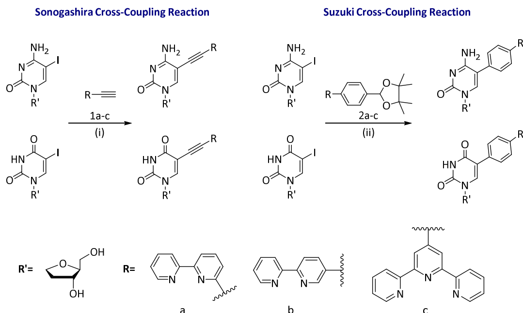
Figure 16: The synthesis of T and C based biPy and terPy . (i) Pd(OAc) 2 , TPPTS, CuI, (iPr) 2 NEt, DMF, 75°C, 2h. (ii) Pd(OAc) 2 , TPPTS, Cs 2 CO 3 , H 2 O-MeCN, 90 °C. 37
