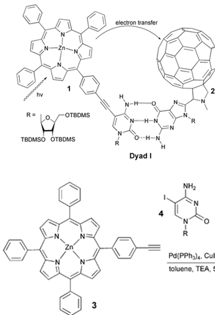
Figure 17: (Top) The self-assembly of the dyad through G-C interaction. (Bottom) The reaction Scheme of the porphyrin synthesis. Figure taken from reference 20.
