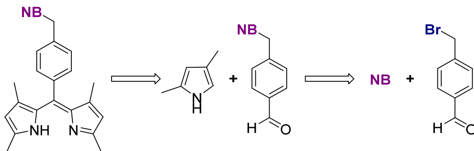
Figure 23: The retrosynthesis of the targeted tectons.
