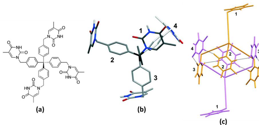
Figure 53: (a) The molecular structure of 4-tmpm. (b) The X-Ray structure of 4-tmpm showing its three-fold rotation symmetry. (c) X-Ray structure of a hydrogen bonded dimer, one molecule is in orange and the other is in light purple. Figure modified from reference 89.
