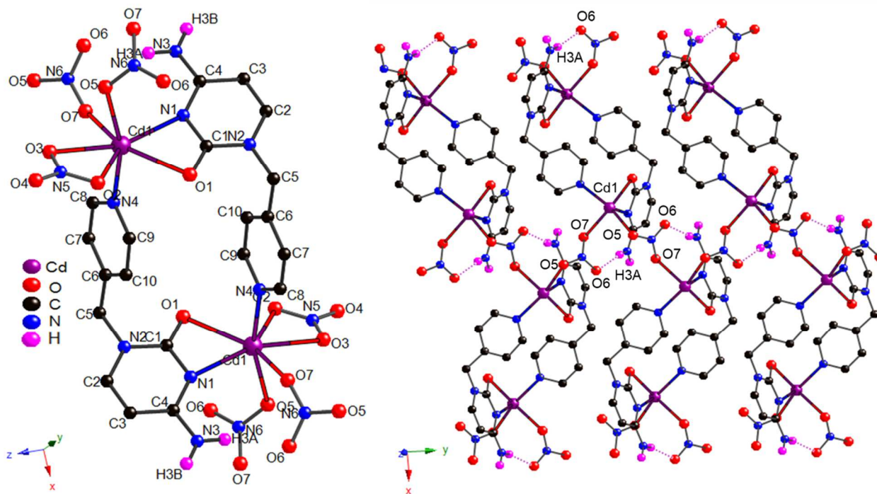
Figure 39: The crystal Structure of C-Py Cd(II) (a) Structure of the \text{Cd}_2(\text{C-Py})_2(\text{NO}_3)_4 dimer. (b) The coordination network formed through the two nitrate bridging ligands. The chelate \text{NO}_3 molecules are omitted for clarity.
