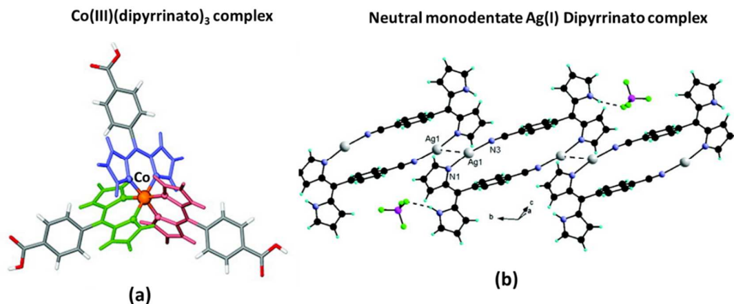
Figure 8: (a) The crystal structure of \text{Co(III)(dipyrin)}_3 complex, Figure taken from reference 23 (a). (b) The crystal structure of a neutral monodentate \text{Ag(I) dipyrinato} complex. Figure taken from reference 27.
