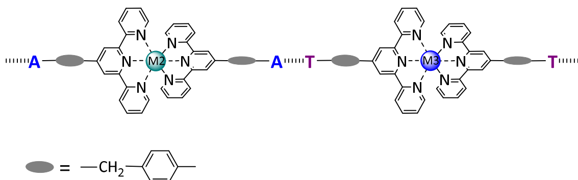
Figure 22: A schematic representation of possible assemblies of A-terPy-M 1 -terPy-T , and A-terPy-M 2 -terPy-A with T-terPy-M 3 -terPy-T .
