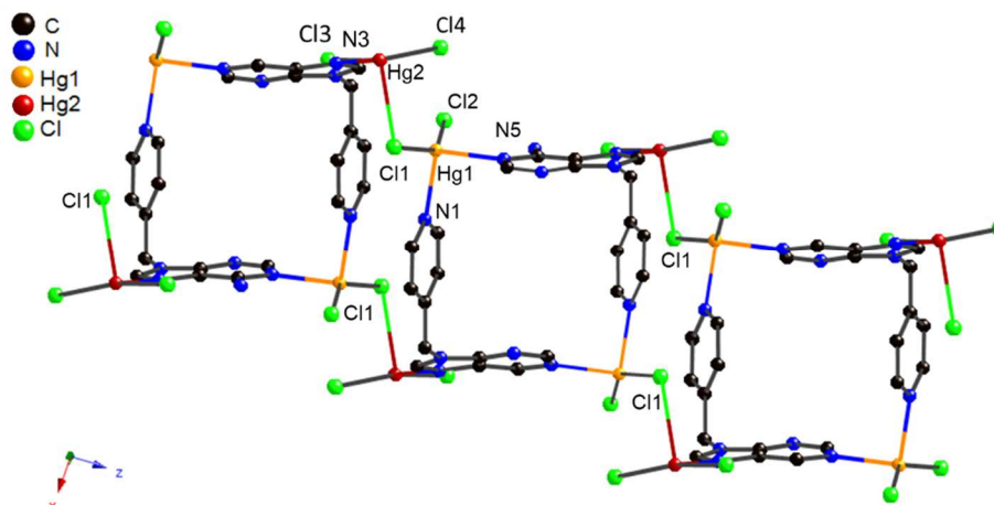
Figure 36: The crystal Structure of the 2 D helix structures linked by a Cl1 atom coordinated to Hg1 of one helix and one Hg2 of the adjacent helix.
