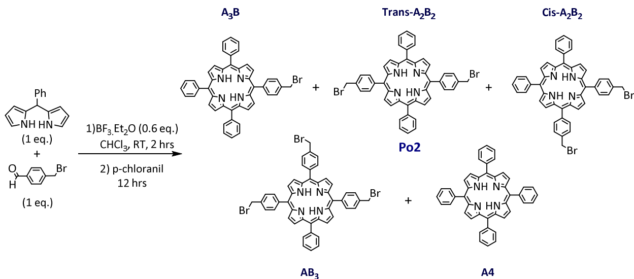
Figure 43: Synthesis of Po2 .
