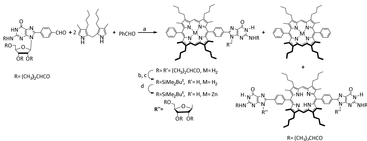
Figure 12: Synthesis of porphyrins bearing guanine for assemblies II and III, (a) (i) TFA, CH 2 Cl 2 , argon, room temperature, 4 h; (ii) NaOAc, 30 min; (iii) p-chloranil, room temperature, 6 h. (b) NH 3 /MeOH, room temperature, 36 h. (c) TBDMS-C1, imidazole, DMF, room temperature, overnight, (d) Zn(OAc) 2 , MeOH, reflux, 30 min. 16
