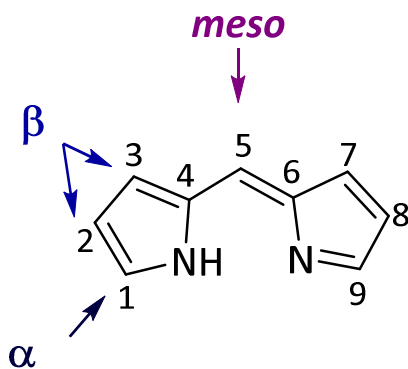
Figure 1: The structure and numbering of dipyrrins
