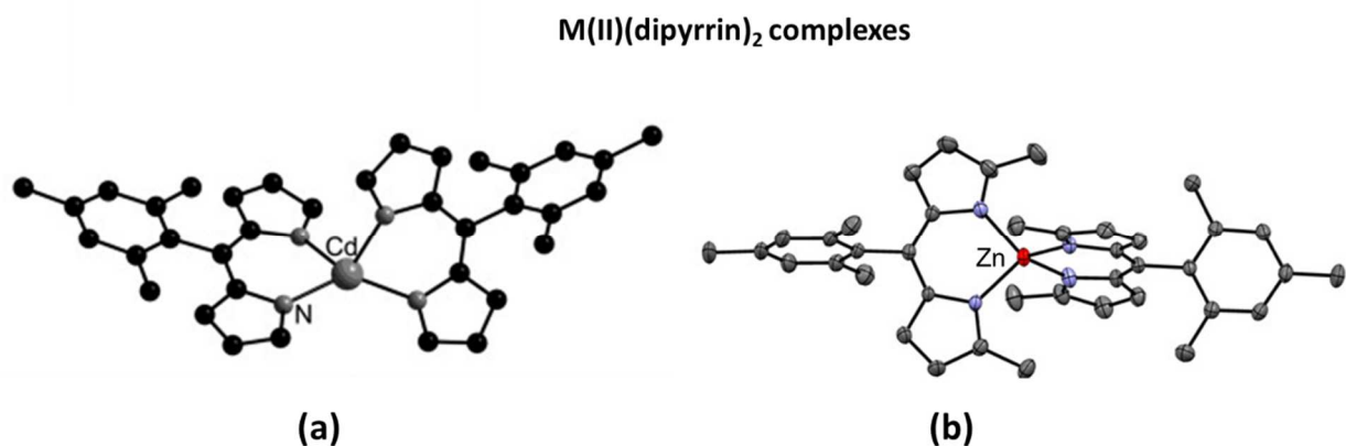
Figure 7: Examples of homoleptic dipyrinato M(\text{II}) complexes. (a) The crystal structure of \text{Cd(II)} (5\text{-mesityldipyrin})_2 . Figure modified from reference 20. (b) The crystal structure of \text{Zn(II)} (1,9\text{-dimethyl-4-mesityldipyrin})_2 . Figure modified from reference 22 (b).
