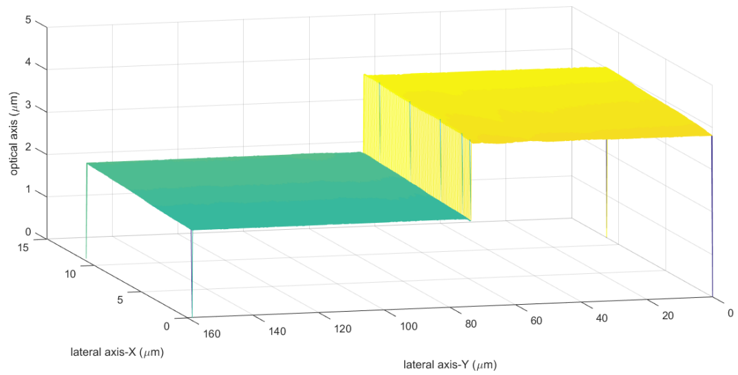
Fig. 92 Surface extracted of the Step Height Standard (SHS) obtained using 3D fringe signal processing from measurements with the new Fogale microscope ("Michelin")
