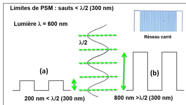
Fig. 46 The limitation of the PSM technique in height measurement
