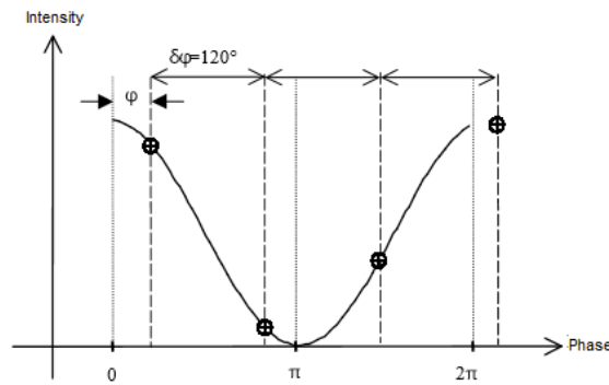
Fig. 4 Phase determination, from 4 discrete steps of 120°[47].
