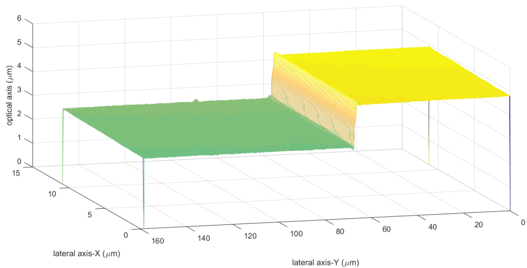
Fig. 89 Surface extracted of the Step Height Standards (SHS) obtained using 3D fringe signal processing on measurements from the modified Leitz-Linnik microscope
