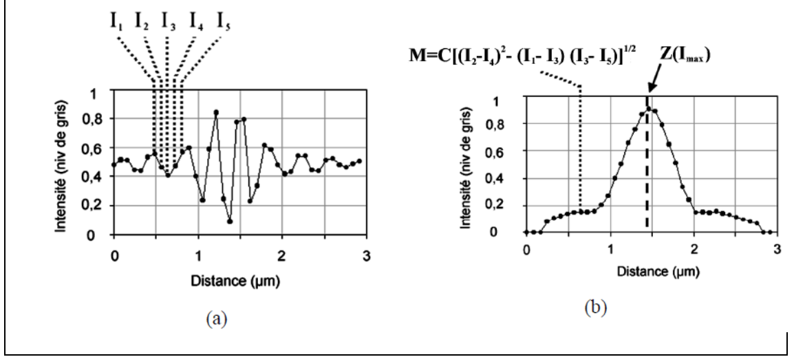
Fig. 13 FSA Algorithm
