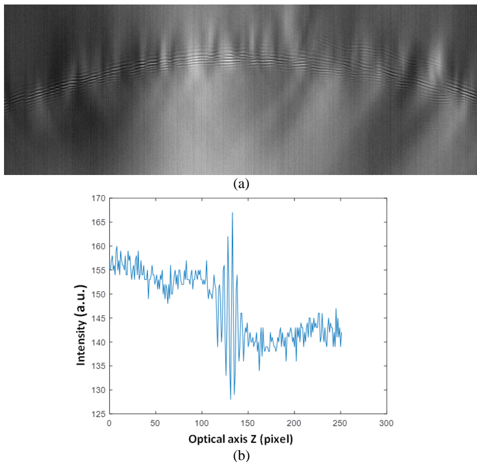
Fig. 106 (a) Fringe image of a Cable and (b) its fringe profile in 1D
