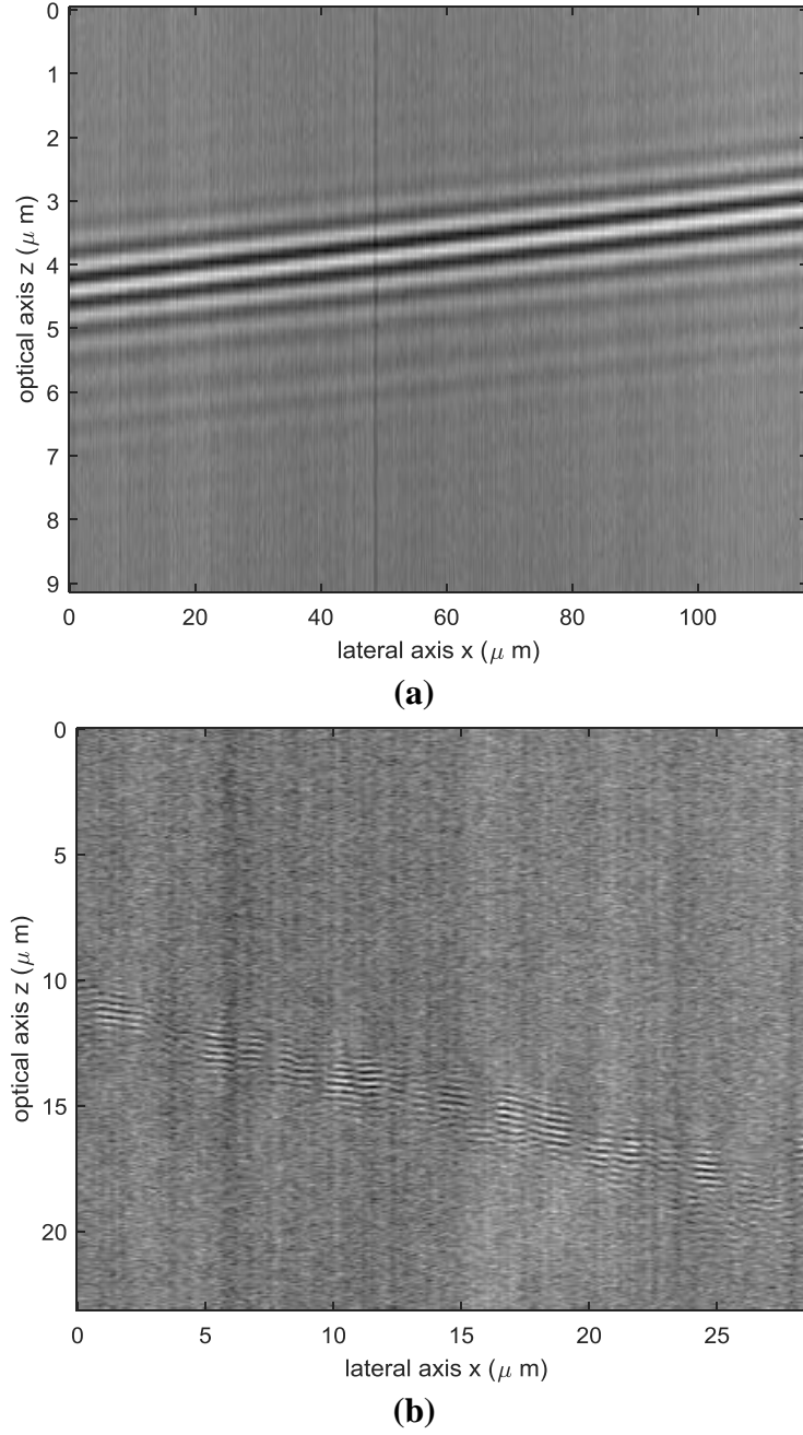
Fig. 25 XZ images showing the interferograms from (a) a Step Height Standard and (b) a rock surface [85].
