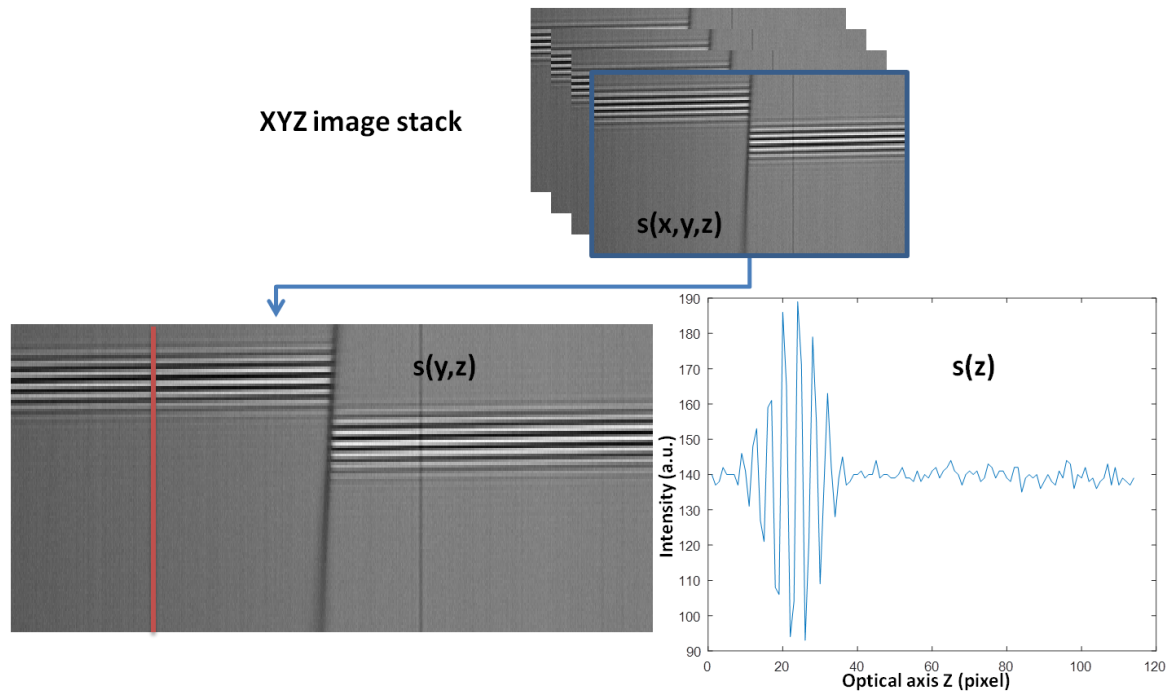
Fig. 94 Fringe signal processing of the Step Height Standard (SHS) from measurements with the "immersion" Fogale microscope
