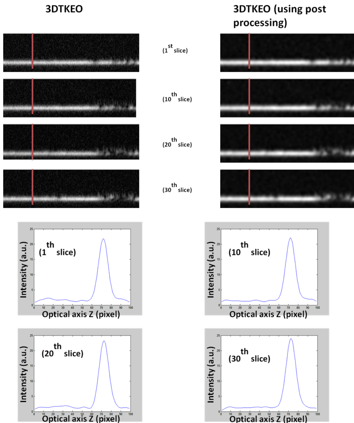
Fig. 80 Improvement results of 3D envelope detection using post-processing
