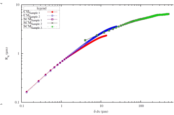
(b) RMS roughness R_q
