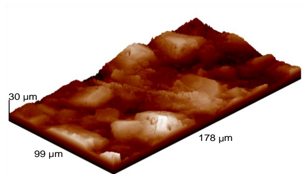
CSI measurement (165 days curing)
