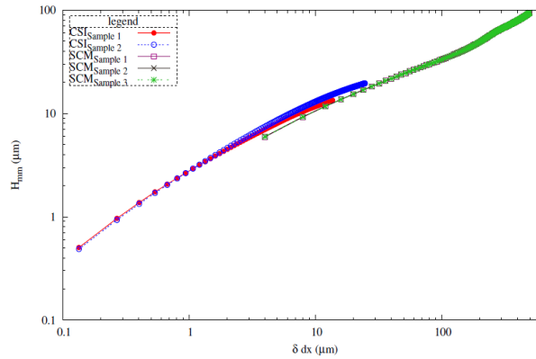
(a) Peak/valley roughness H_{mm}
