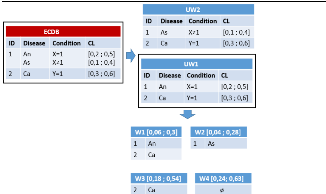
Figure 5.3: From the compact ec-table to its possible worlds
