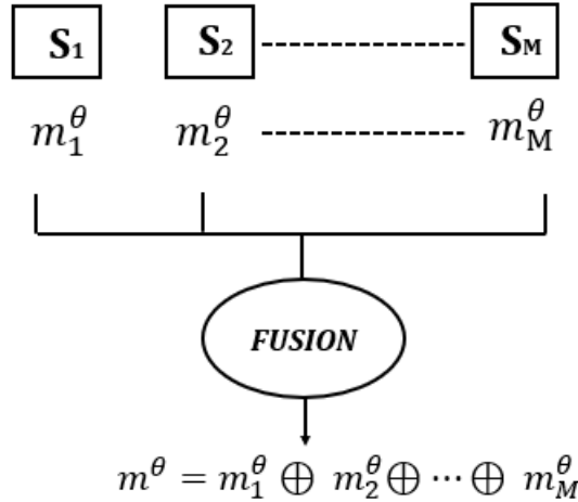
Figure 2.5: Combination of M independent sources (Dempster, 1967)
