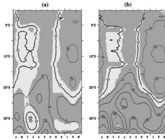
Fig. 1.18 Change (in %) of the alongshore wind component off Peru and Chile, between 0^{\circ}\text{S} and 40^{\circ}\text{S} , between the scenarios a) pre-industrial and 2\text{CO}_2 , b) pre-industrial and 4\text{CO}_2 . Adapted from Goubanova et al. (2011).
