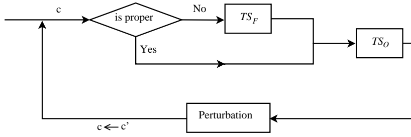
Figure 4.3: An illustration for the IDTS procedure.
