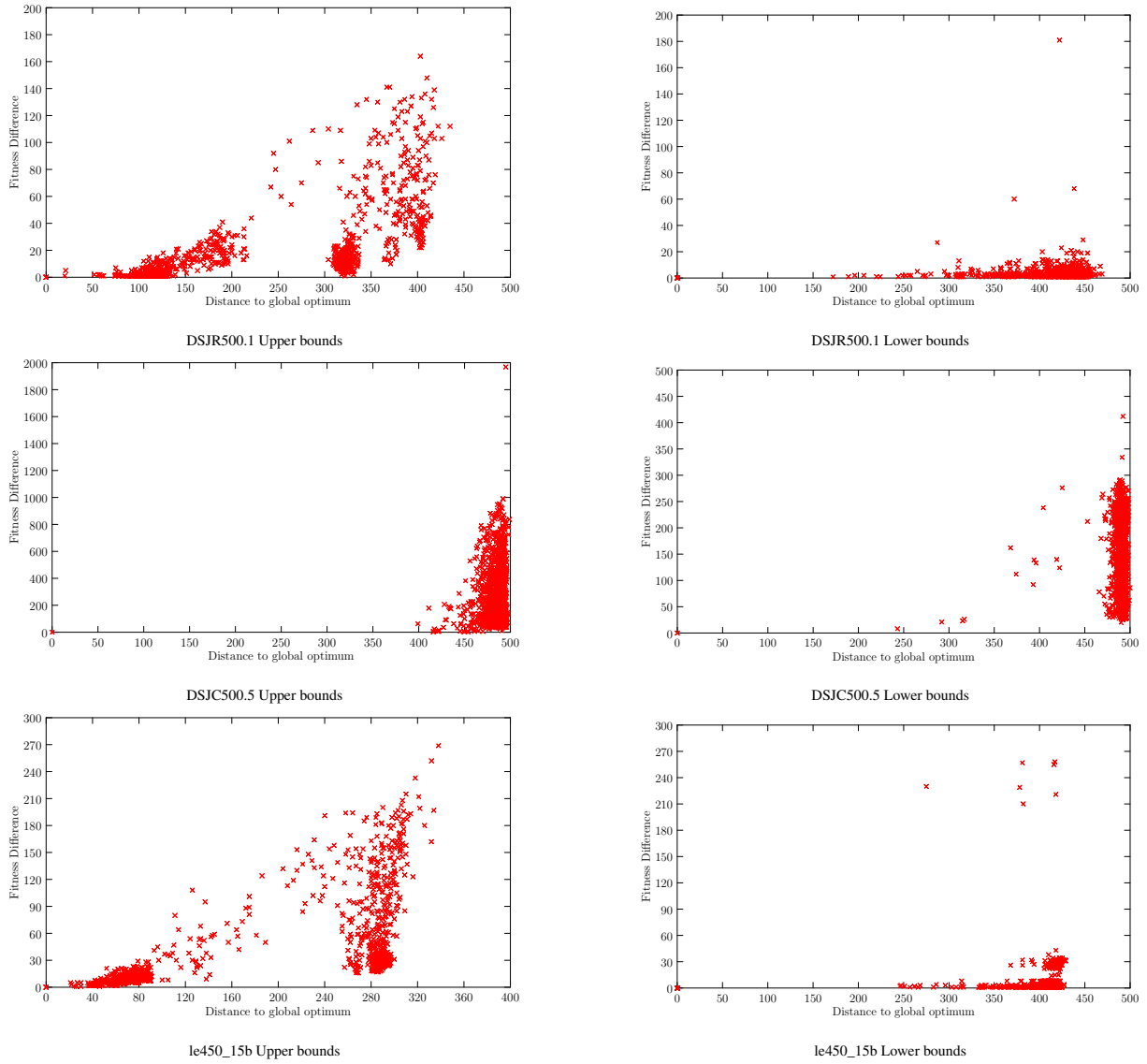
Figure 4.6: FDC plots on 4 graphs for the lower and upper bounds
