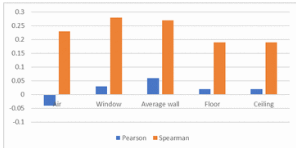
Figure 61 : Correlation between outdoor air temperature and inner temperature accuracy
