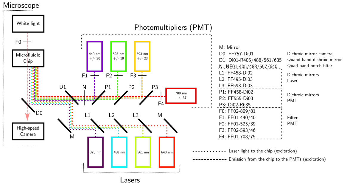
FIGURE 2.3: Microfluidic station optical setup.
