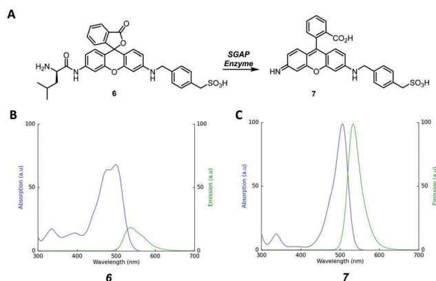
Fig. 2 Enzymatic evaluation of substrate 6 : (A) enzymatic release of sulfonlated rhodamine 7 . (B) Absorption and emission spectra of compound 6 (10 \mu M) in pH = 8.0 SGAP buffer. (C) Absorption and emission spectra of compound 7 (10 \mu M) in pH = 8.0 SGAP buffer.
