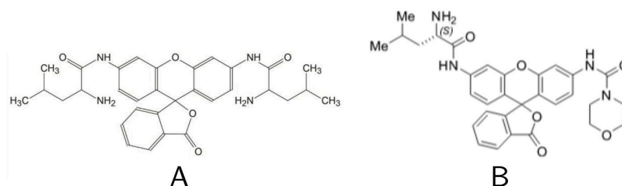
FIGURE 2.10: Structure of the two main substrates used in the SGAP experiments. A: Leu 2 Rho. B: LeuRhoMS. \lambda_{ex} = 488nm , \lambda_{em} = 535nm
