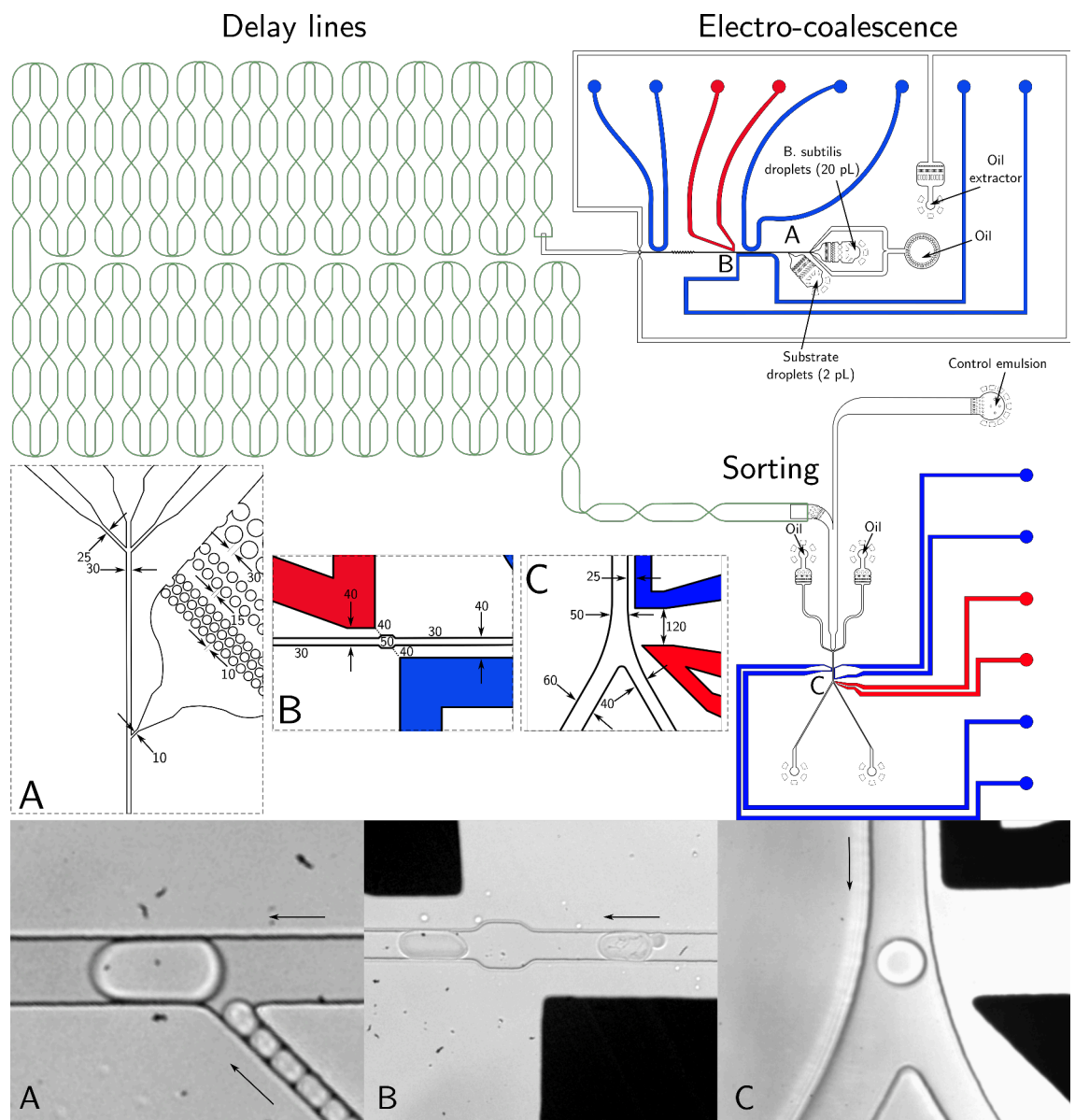
FIGURE 2.9: 2-20 pL droplet electro-coalescence device (integrated with delay lines and sorting device). All dimensions are in \mu\text{m} . Channels height is 20\ \mu\text{m} except for the delay lines where channels height is 75\ \mu\text{m} . Pressure settings: Emulsions: 600\ \text{mBar} , oil phase: 600\ \text{mBar} . The extractor is used to extract oil and increase the incubation time in the delay lines, or filled with oil and blocked with a piece of electrical wire. A Droplets are paired one to one by adjusting the pressures and B droplets are fused by applying a voltage ( 600\ \text{V} , 30\ \text{kHz} ) between the positive electrode (red) and the negative electrodes (connected to the electrical ground), using a function generator connected to a \times 1000 high voltage amplifier. C : Droplet fluorescence is measured between the two sorting electrodes (similar to 2.8).
