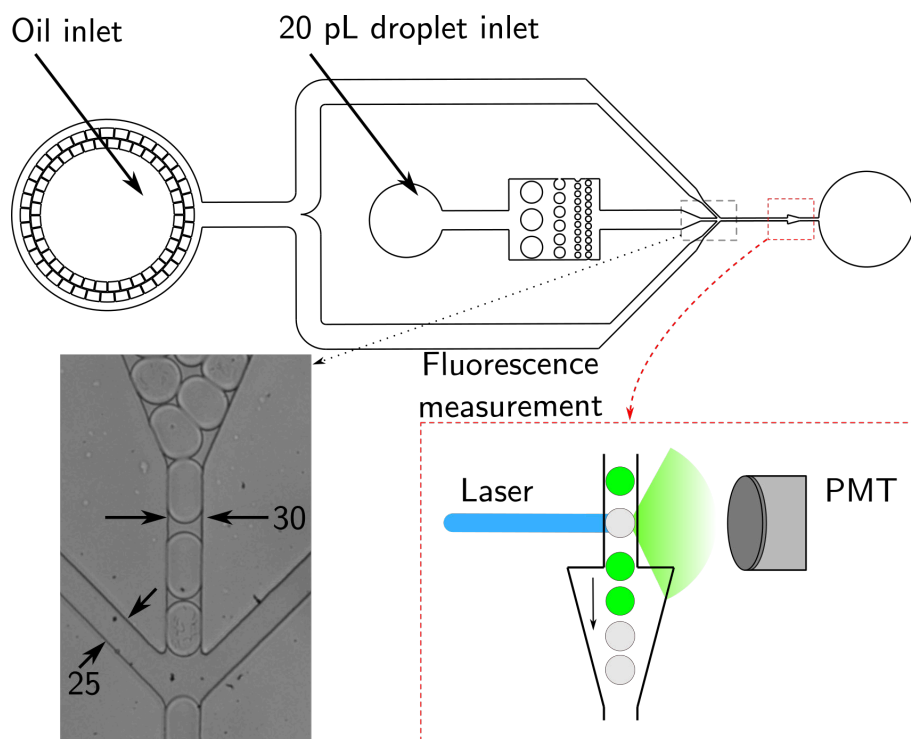
FIGURE 2.8: 20-30 droplet reinjector All dimensions are in \mu\text{m} . Channels height is 20 \mu\text{m} . Pressure settings: Emulsion: 600 mBar, oil phase: 600 mBar.
