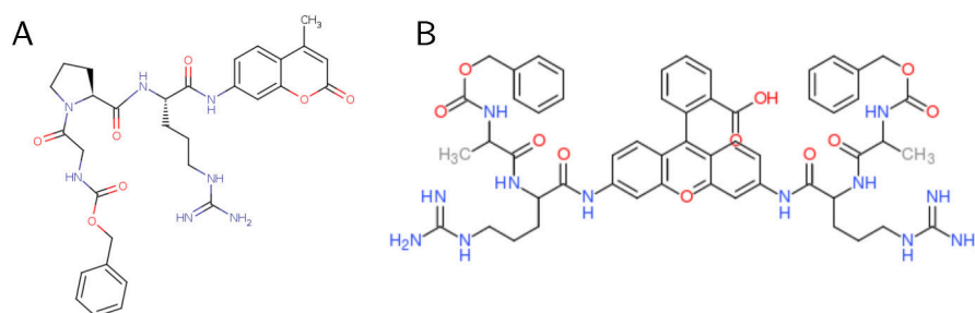
FIGURE 2.11: Structure of the two main substrates used in the trypsin experiments. A: Coumarin based trypsin substrate \lambda_{ex} = 372nm , \lambda_{em} = 445nm . B: Rhodamine 110 based trypsin substrate \lambda_{ex} = 488nm , \lambda_{em} = 535nm
