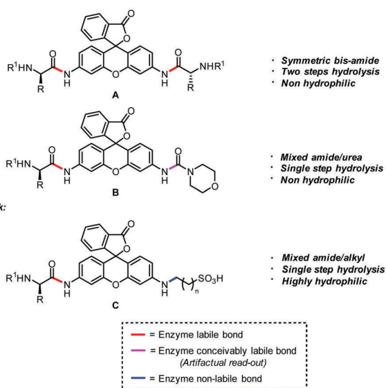
Scheme 1 Different type of fluorogenic rhodamine-based substrates developed for detection of enzymatic activity.
