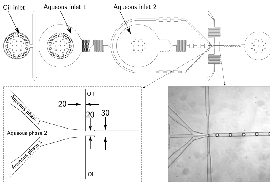
FIGURE 2.7: 20-30 pL co-flow droplet maker All dimensions are in \mu\text{m} . Channels height is 20 \mu\text{m} . Pressure settings: both aqueous phases: 1100 mBar, oil phase: 1000 mBar.
