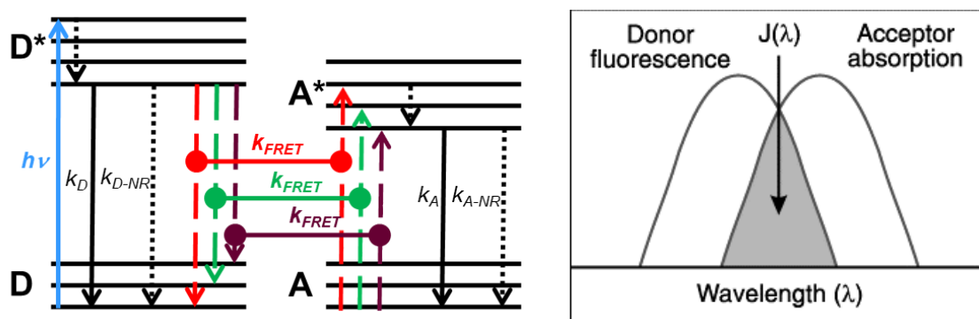
Figure 2.3. (Left) Simplified Jablonski diagram representing the energy levels of the donor (D) and acceptor (A) molecules. (Right) Spectral overlap between the donor emission and the acceptor absorption.
