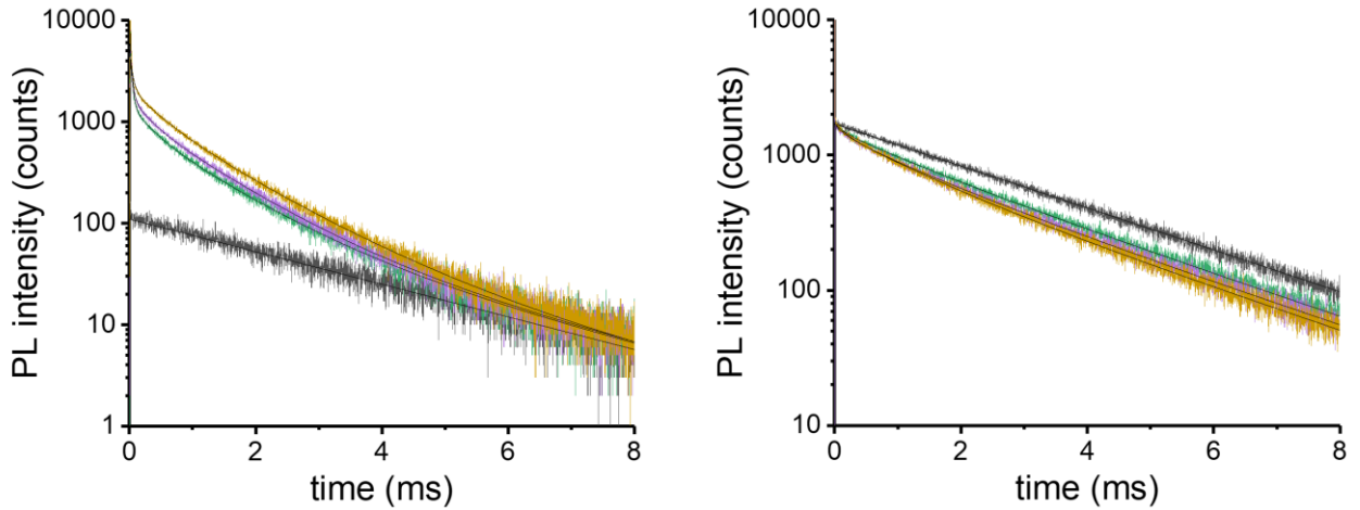
Figure 5.8. The PL decay curves of QD acceptor (left) and Tb donor (right) situated at 14 bases ssDNA distances from each other. Black: pure Tb (some Tb luminescence is also visible in the acceptor detection channel due to spectral crosstalk); green: 6 nM peptide-DNA; purple: 8.0 nM peptide-DNA; yellow: 10.0 nM peptide-DNA. Black lines represent the fit results from below.
