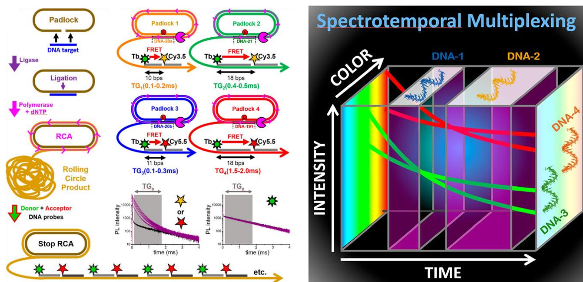
Figure 1.2. The principle of spectrotemporal quadruplexing RCA-FRET assay and PL multiplexing in three dimensions. x-axis: lifetime; y-axis: color; z-axis: intensity
