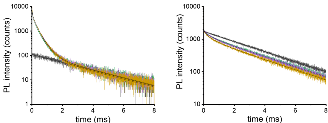
Figure 5.4. The PL decay curves of QD acceptor (left) and Tb donor (right) situated at 2 bases ssDNA distances from each other. Black: pure Tb (some Tb luminescence is also visible in the acceptor detection channel due to spectral crosstalk); green: 6 nM peptide-DNA; purple: 8.0 nM peptide-DNA; yellow: 10.0 nM peptide-DNA. Black lines represent the fit results from below.
