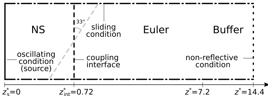
Fig. 6: sketch of the computational domain for the wave guide.
