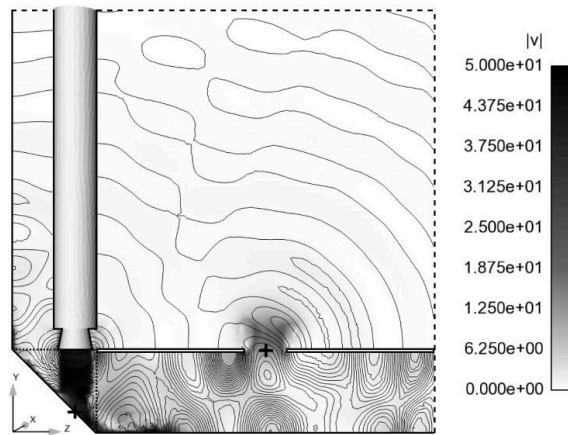
Fig. 17: snapshot of the velocity field in the LPM1 case at t = 0.07 s in the plane x = 0 , superimposed with pressure iso-lines. — : wall; - - - : non-reflective condition; ···· : coupling interface; — : pressure iso-lines; +: probe.
