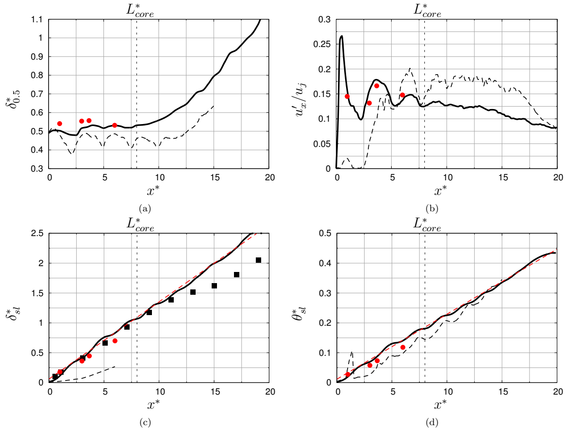
FIG. 13: free jet shear layer properties. (13a) half velocity thickness, (13b) fluctuating axial velocity along the lipline (array A), (13c) shear layer thickness, (13d) momentum thickness. ●: experimental data from MARTEL; ■: experimental data from Troutt and McLaughlin 61 ( M_j = 2.1 , Re \sim 10^6 ); —: present numerical data; ---: numerical data from Langenais 2017; 44 -.-: asymptotic spread rates d\delta_{sl}^*/dx^* = 0.13 and d\theta_{sl}^*/dx^* = 0.022 .
