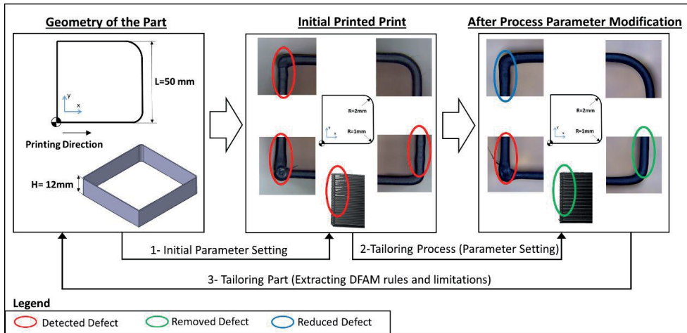
Figure 42. Printing result before and after process parameter modification ( Publication IV )
