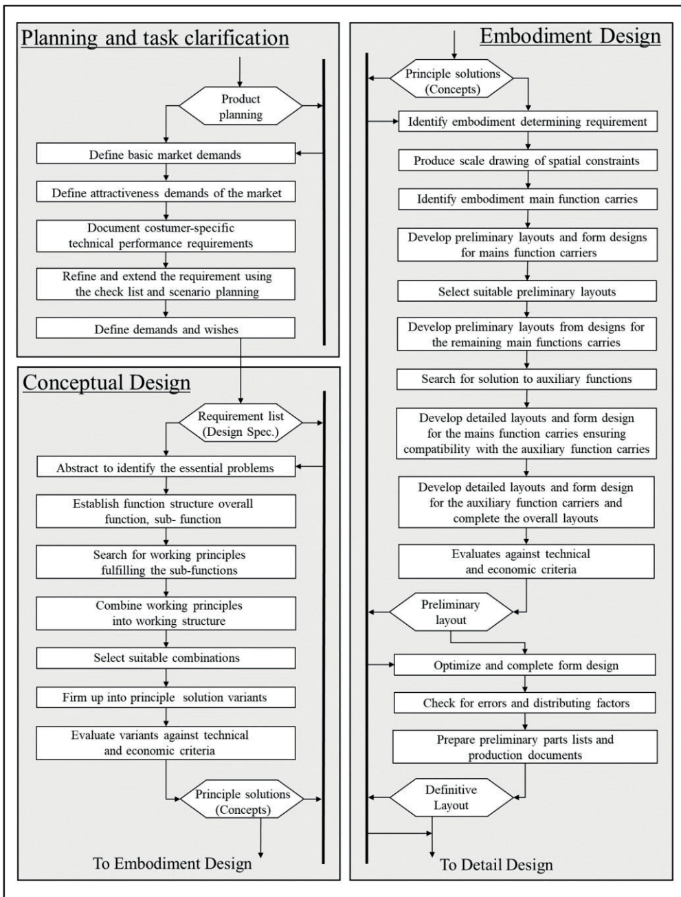
Figure 5. Steps required in setting up requirement lists, conceptual design, embodiment design, rearranged from (Pahl et al., 2007)
