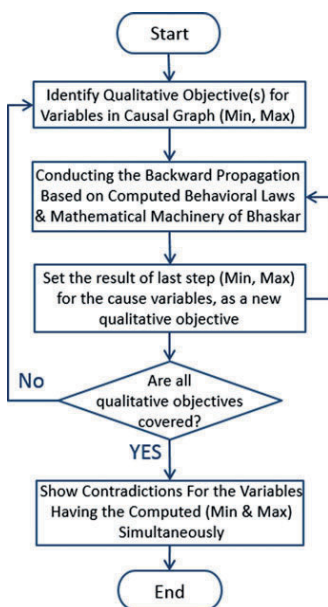
Fig. 18. Contradiction detection algorithm.
