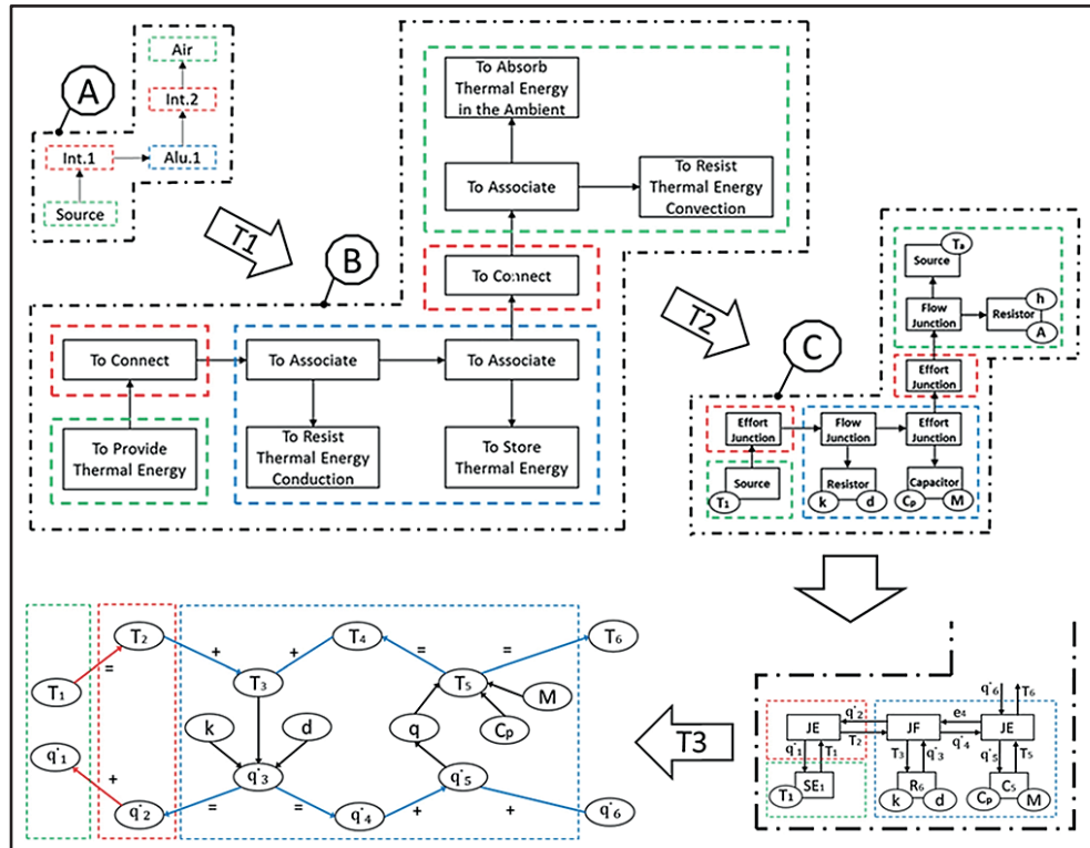
Figure 38. A) Systematic transformation between interface analysis, B) functional model, C) generic functional representation, and extracting causal graph for thermal heat exchange in FFF liquefier ( Publication IV )
