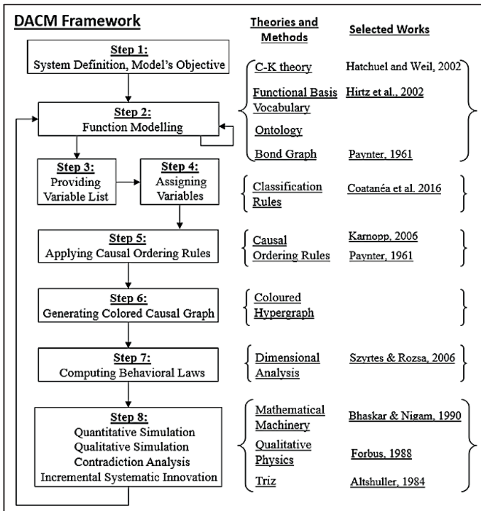
Figure 15. Modeling steps in DACM framework (Publication III)
