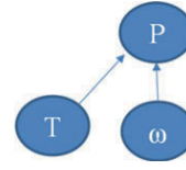
Fig. 14. Causal graph.
