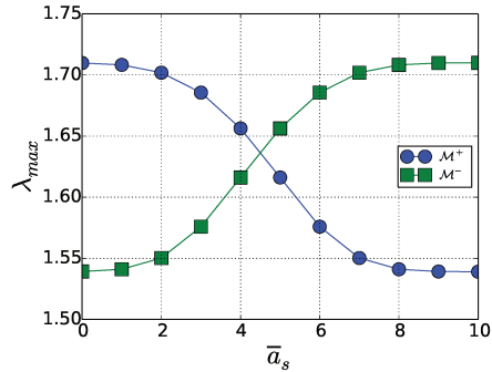
Figure 4.5: Dependence of greater eigenvalues of matrices \mathcal{M}^+ (blue circles) and \mathcal{M}^- (green squares) respectively on \bar{a}_s for N = 10 , r_{div} = 0.9 , r_d = r_s = 0.1 . Hence (1 - r_d)(1 + r_{div})(1 - r_s) = 1.539 and (1 - r_d)(1 + r_{div}) = 1.71 .
