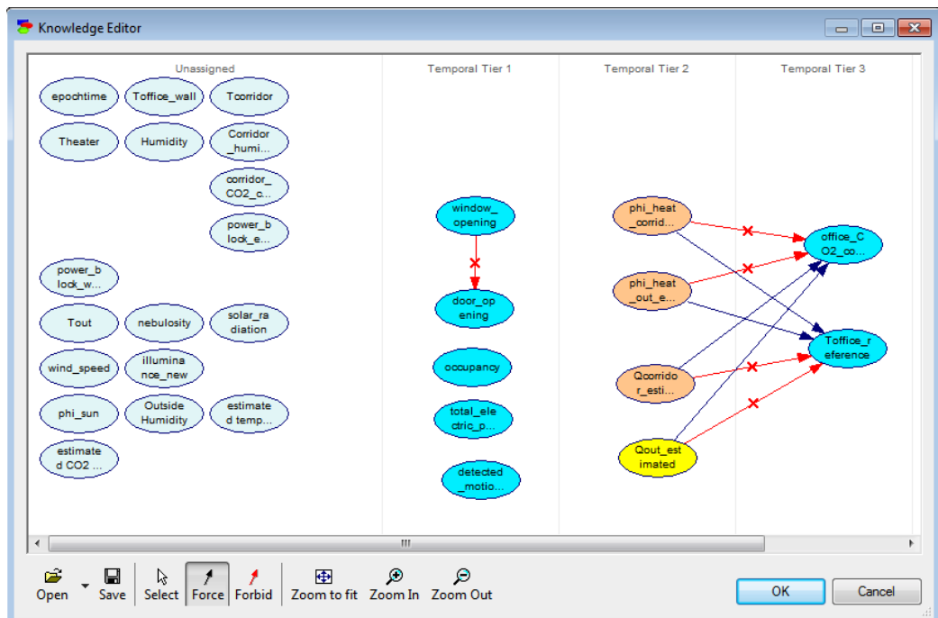
Figure 4.15: Model fragment in the form of potential causalities (figure is realized using the BayesFusion program)
