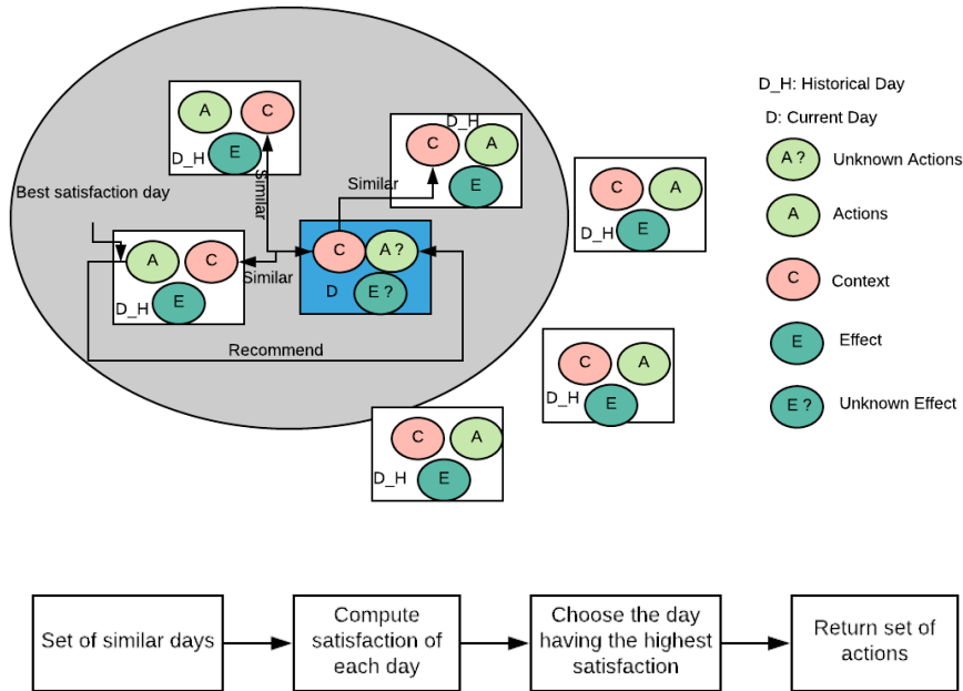
Figure 5.5: Obtain the best set of actions
