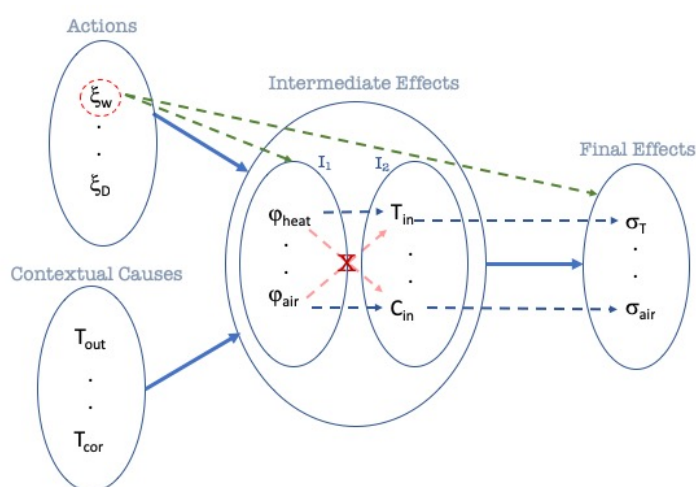
Figure 4.12: The representation of the potential and forbidden causalities
