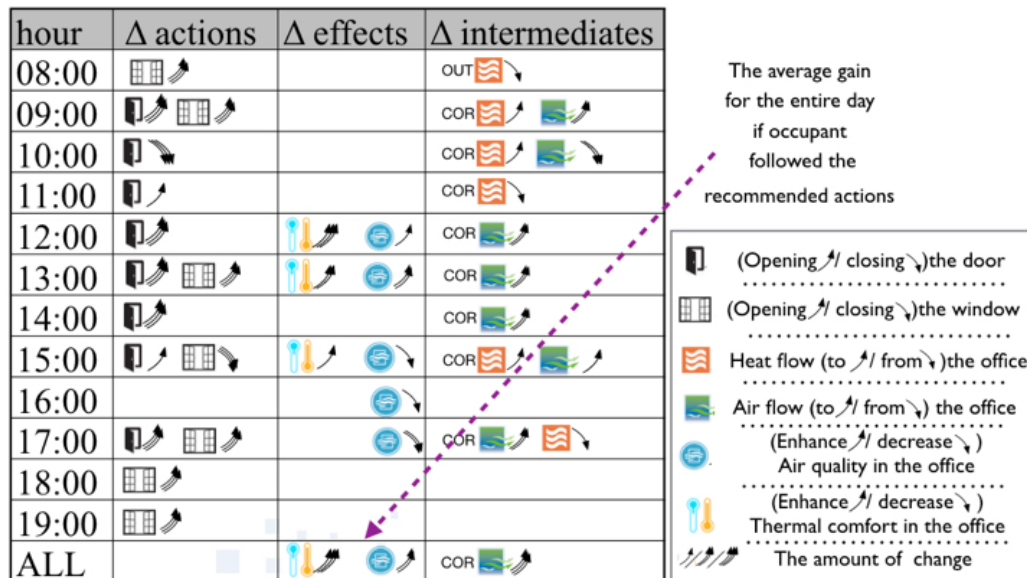
Figure 4.9: Differential explanations through difference between the historical scenario and a Pareto-optimal scenario for 05-May-2015
