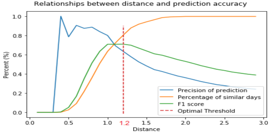
Figure 5.11: Result of threshold Context distance T_C approach
