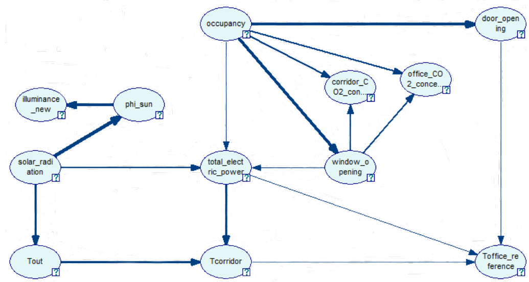
Figure 5.15: Bayesian network for similar days
