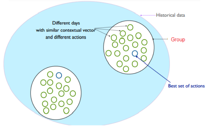
Figure 5.2: Concept of proposed solution
