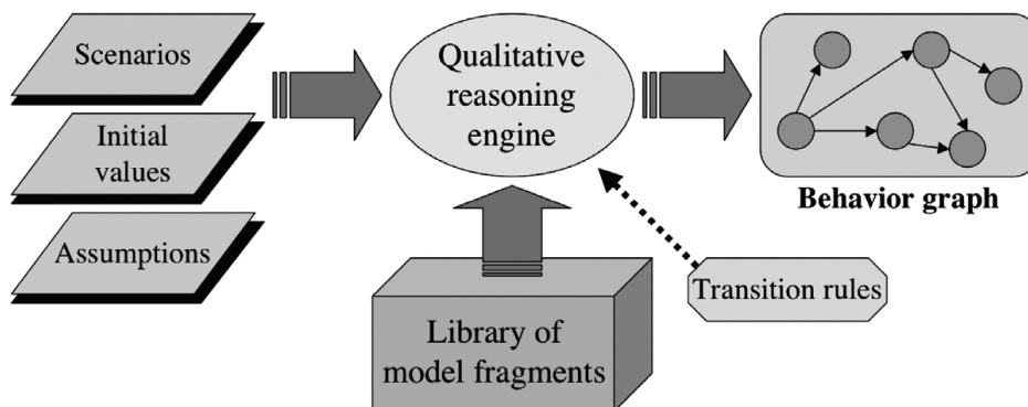
Figure 3.2: Basic architecture of the qualitative reasoning engine [15]
