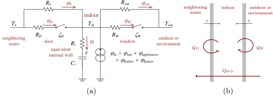
Figure 4.2: Building simulation models: (a) thermal model [106], (b) aeraulic model [74]
