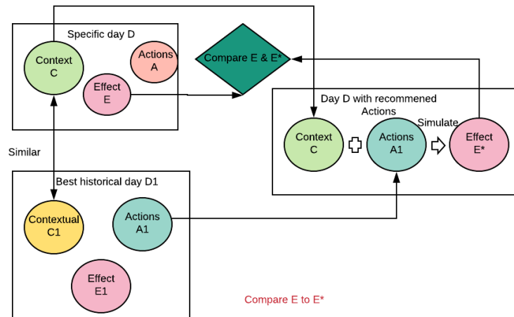
Figure 5.10: The concept of recommended actions validation
