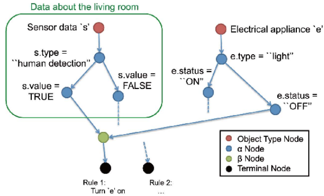
Figure 2.3: An example of a rule-based system [59]
