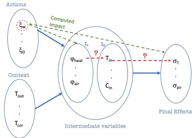
Figure 4.11: Undetected causality between intermediate variables and effects
