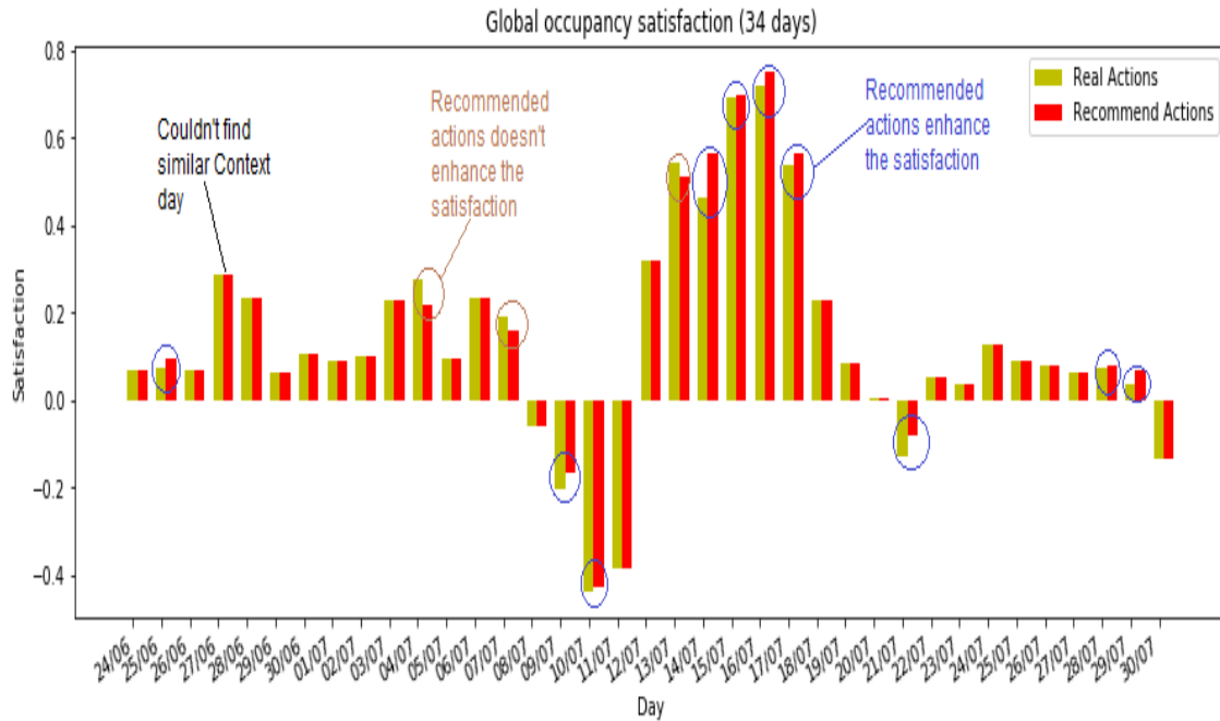
Figure 5.12: Results of recommended actions to enhance global satisfaction (When no similar context day is not found the same actions of the test day are used for simulation)
