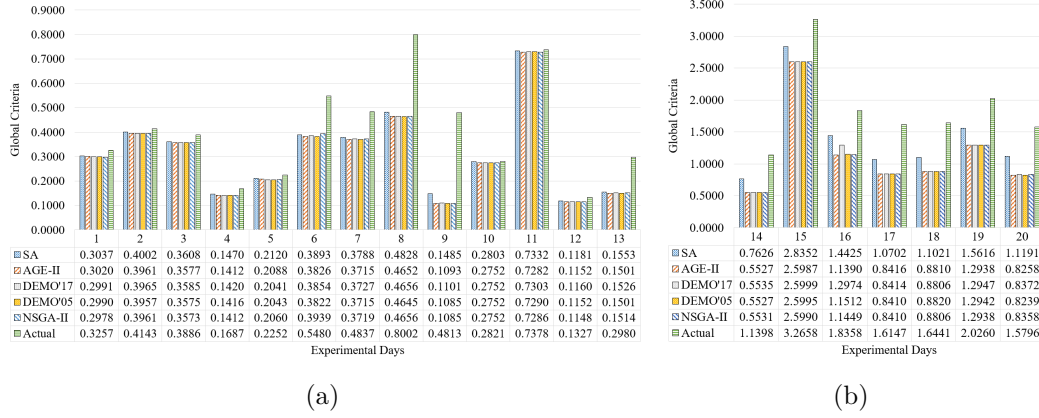
Figure 9.1: Comparing the performance of optimizers when global criteria with respect to actual schedule of occupant's actions is (a) less than or equal to 1, (b) greater than 1
