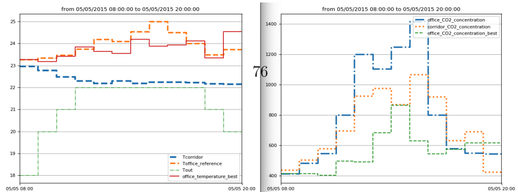
Figure 4.7: Outside, corridor, inside, best (with recommended actions) temperature (left) and corridor, inside, recommended air quality (right)
