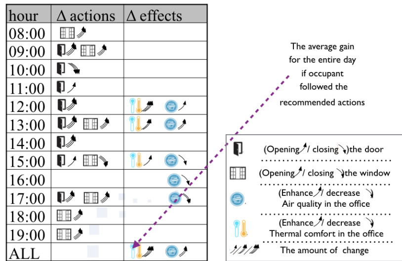
Figure 5.14: Descriptive differential explanations
