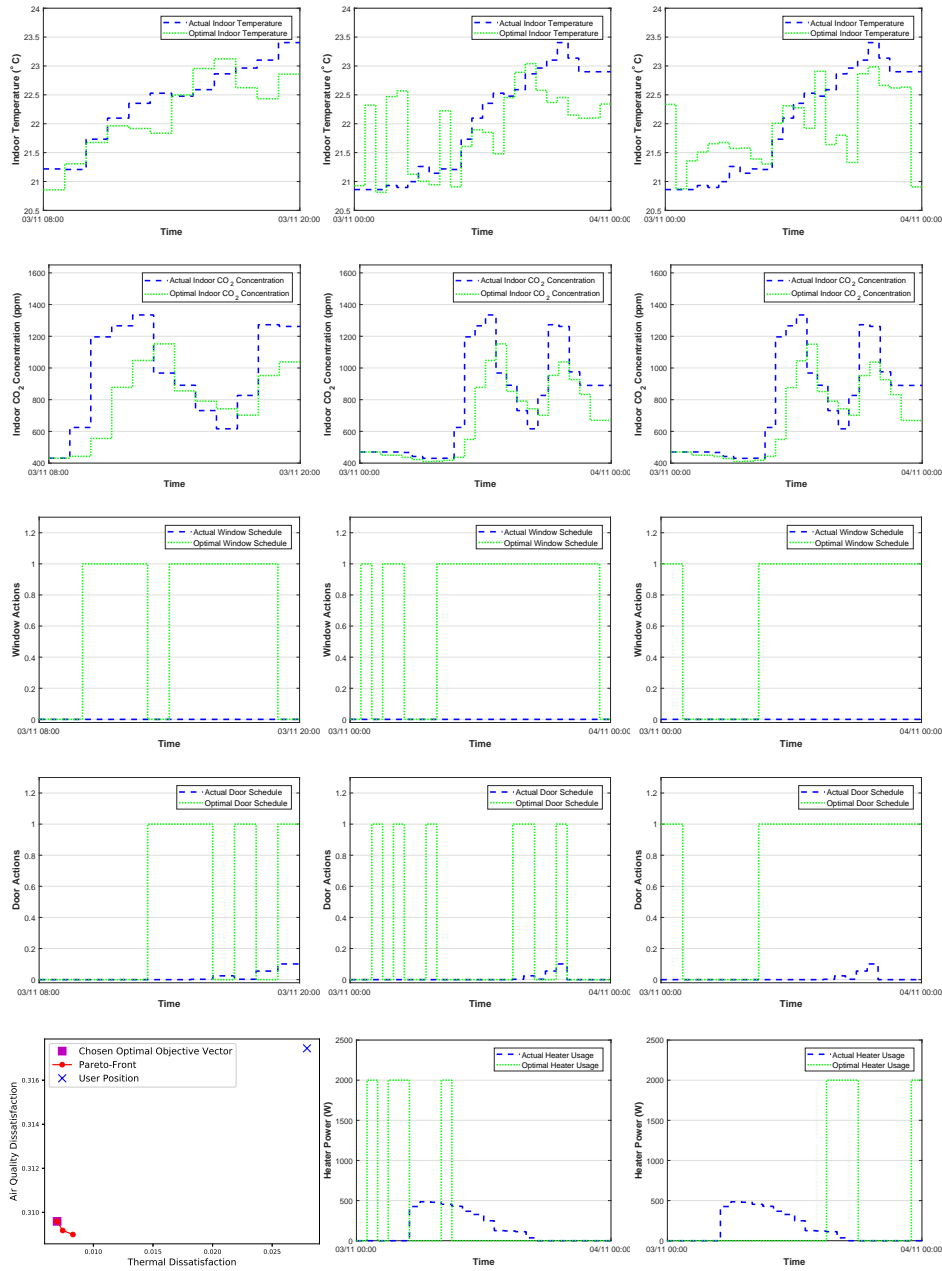
Figure 9.2: Indoor physical parameters along optimal actions for 2-objective problem with \sigma_{temp} and \sigma_{air} (first column); for 3-objective problem with \sigma_{temp} , \sigma_{air} and \sigma_{cost} (second column); and for 4-objective problem with \sigma_{temp} , \sigma_{air} , \sigma_{cost} and \delta_{WD} (third column)
