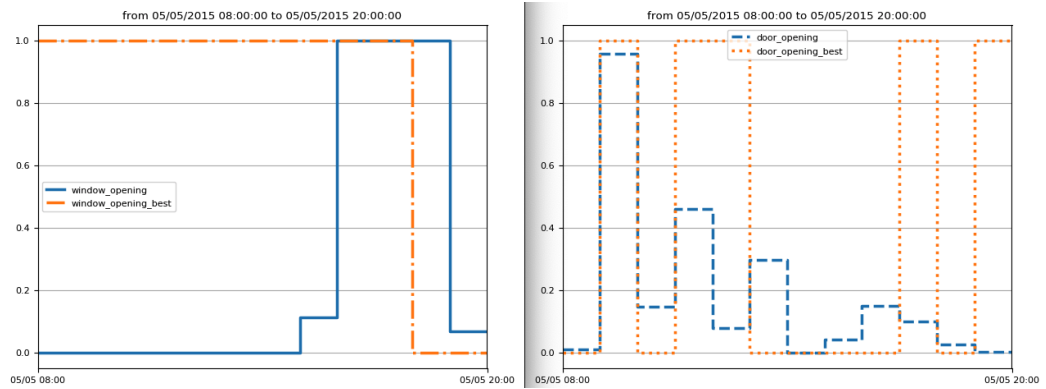
Figure 4.4: window (left) / door(right) opening (measured and recommended)
