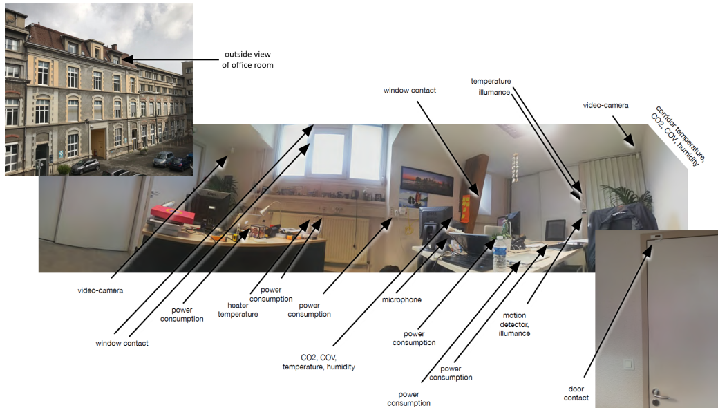
Figure 4.1: Office at Grenoble Institute of Technology fitted with 27 sensors
