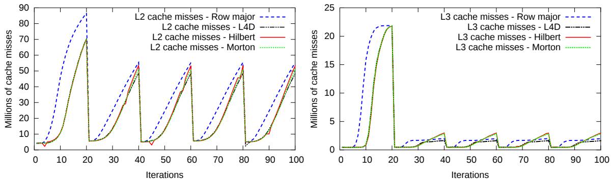
Figure 4.7 – Millions of cache misses per iteration for the cache level 2 during the update- velocities and accumulate loops. Test case in Table 4.3. Figure 4.8 – Millions of cache misses per iteration for the cache level 3 during the update- velocities and accumulate loops. Test case in Table 4.3.
