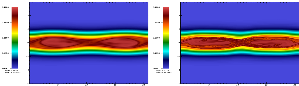
Figure 7.16 – x - vx cut (electrons distribution) for A = 0.01 , BSL \Delta t = 0.1 on 64 \times 256 grid, at time T = 150 , 1d1v test case in (7.9) and (7.10) at time T = 150 , 1d1v test case in (7.9) and (7.10)
