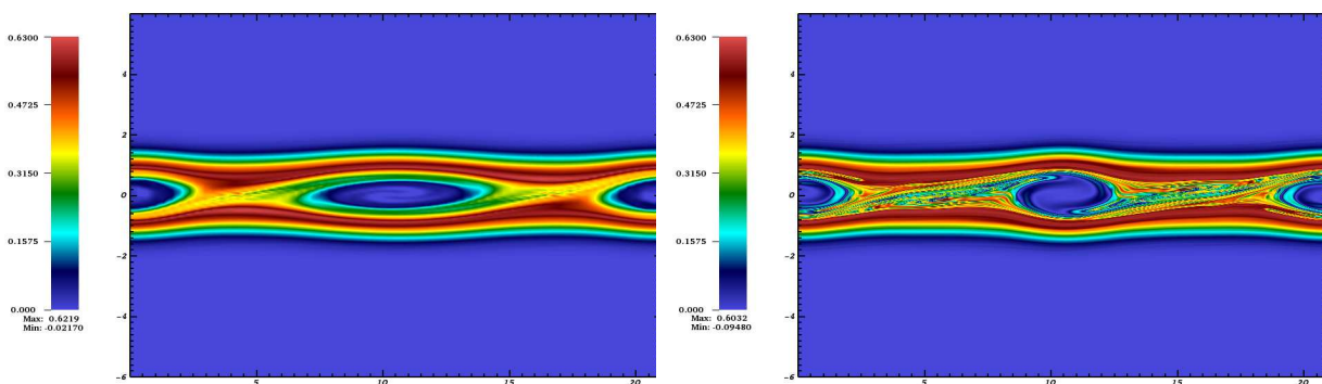
Figure 7.18 – x - vx cut (ions distribution) for A = 0.01 , BSL on 64 \times 256 grid, at time T = 150 , 1d1v test case in (7.9) and (7.10) at time T = 150 , 1d1v test case in (7.9) and (7.10)
