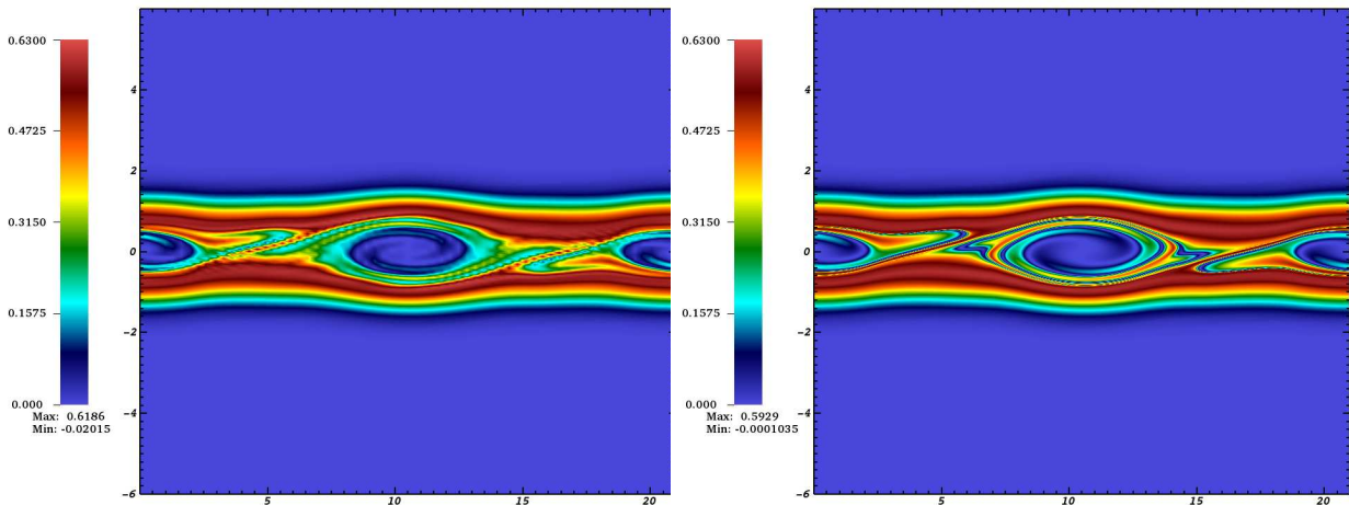
Figure 7.20 – x - vx cut (ions distribution) for Figure 7.21 – x - vx cut (ions distribution) for A = 0.01 , BSL \Delta t = 0.1 on 64 \times 256 grid, at A = 0.01 , BSL \Delta t = 0.1 on 512 \times 2048 grid, at time T = 80 , 1d1v test case in (7.9) and (7.10) time T = 80 , 1d1v test case in (7.9) and (7.10)
