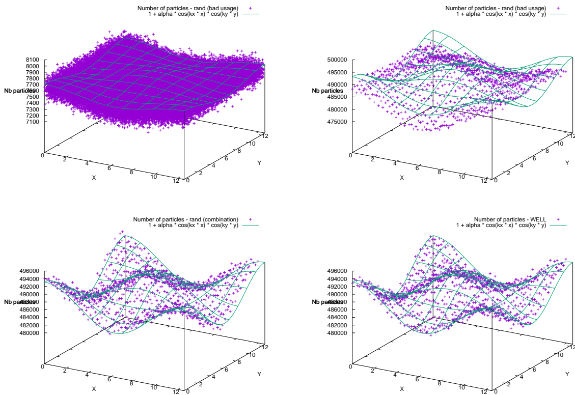
Figure 2.6 – Sampling 500 million particles following (1 + 0.01 \cdot \cos(x/2) \cdot \cos(y/2)) . Top left: 32-bits rand(), 256 \times 256 grid. Top right: 32-bits rand(), 32 \times 32 grid. Bottom left: two 32-bits rand() combined, 32 \times 32 grid. Bottom right: WELL, 32 \times 32 grid.
