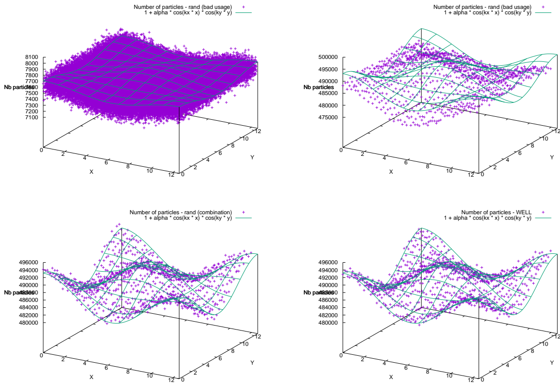
Figure 2.6 – Sampling 500 million particles following (1 + 0.01 \cdot \cos(x/2) \cdot \cos(y/2)) . Top left: 32-bits rand(), 256 \times 256 grid. Top right: 32-bits rand(), 32 \times 32 grid. Bottom left: two 32-bits rand() combined, 32 \times 32 grid. Bottom right: WELL, 32 \times 32 grid.
