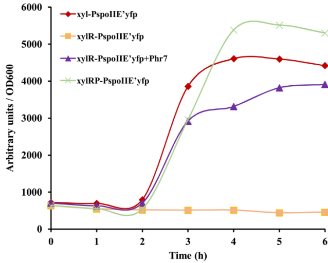
Fig. 4 Rap8 prevents expression of Spo0A-regulated genes. Kinetics of spoIIE expression.
