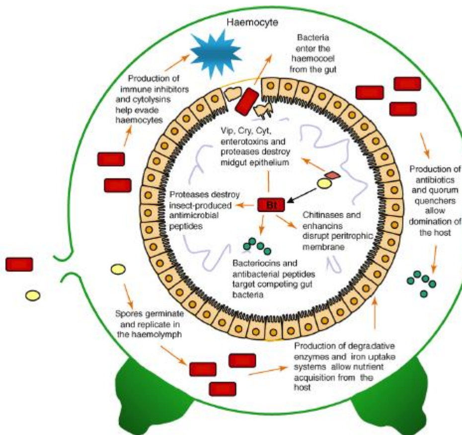
Figure 3. Interactions between B. thuringiensis and its host. The schema shows the lumen of midgut to the peritrophic matrix (blue line), midgut epithelial cells, the haemocoel and the cuticle (green line). Red rectangle represent vegetative cells, cream ovals the spores and pink diamonds the crystals. Some compartments, barriers and immune innate response faced to B. thuringiensis are represented (Raymond et al. , 2010).
