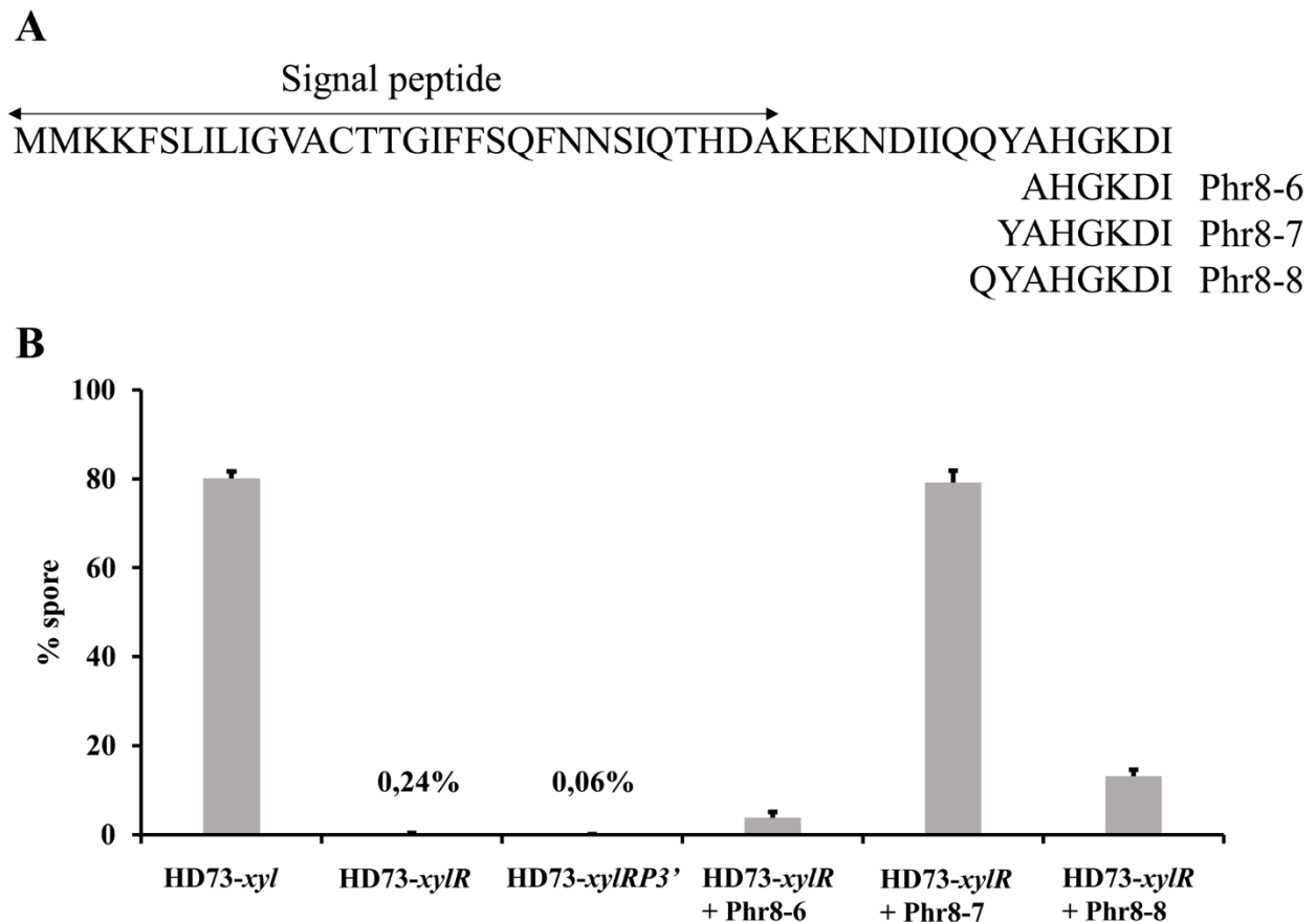
Fig. 3 Characterization of the signaling peptide Phr. (A) Amino acid sequence of the Phr8 peptide and of the synthetic peptides used for complementation experiments. The double arrow indicates the N-terminal putative signal peptide sequence. The potential cleavage site was predicted with the SignalP 4.1 program ( http://www.cbs.dtu.dk/services/SignalP ). (B) Sporulation efficiency of the HD73 control (HD73- xyl ) strain and expressing Rap8 (HD73- xylR ), Rap8-Phr8 truncated for 6 last C-terminal amino acids (HD73- xylRP3' ) strains. The strain expressing Rap8 (HD73- xylR ) was complemented with the synthetic peptides Phr8-6, Phr8-7 and Phr8-8 added independently 1 hour after the onset of the stationary phase at 50 \mu M final concentrations. The viable cells and heat-resistant spores were counted after 2 days in HCT medium at 30°C. Error bars: Standard Error of the Mean (SEM).
