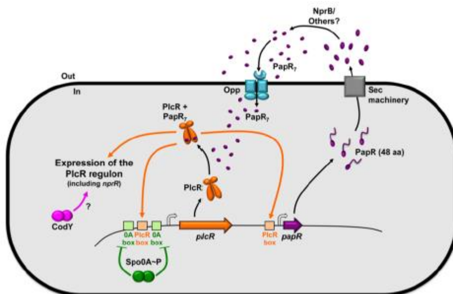
Figure 24. Schematic representation of the QS system of B. cereus group, PlcR/PapR.
