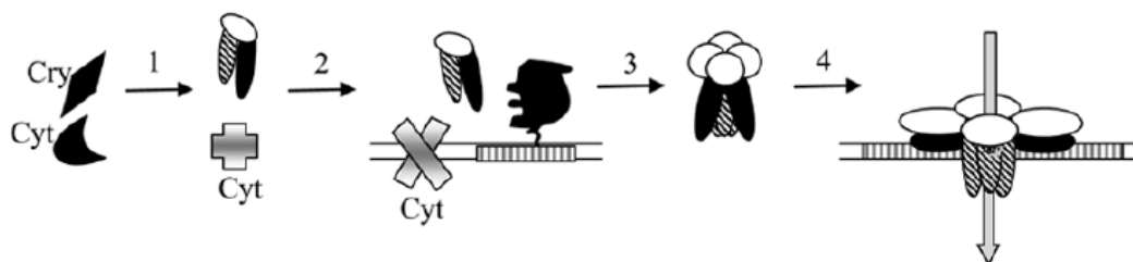
Figure 7. Mode of action of Cyt toxins in synergy with Cry toxins. Both proteins are solubilized and their active form is released (1). Cyt toxin inserts into the membrane and Cry toxin binds to membrane receptors, ALP or Cyt toxin (2). Cry toxins form oligomers (3). Oligomers are inserted into membrane resulting in pore formation (4) (Bravo, Gill and Soberón, 2007).
