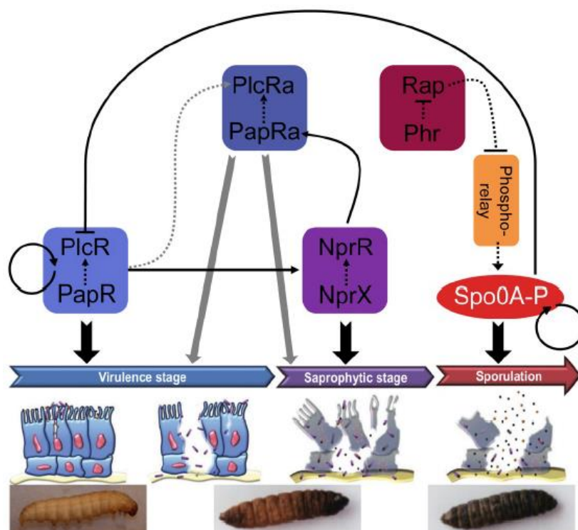
Figure 27. Sequential activation of the QS systems of B. thuringiensis pathogenic lifecycle in the insect. Solid lines: transcriptional effect; dotted lines: peptide- or protein-protein interaction; grey lines: putative effect. Arrows and blunt lines: positive or negative effect, respectively. The bottom
