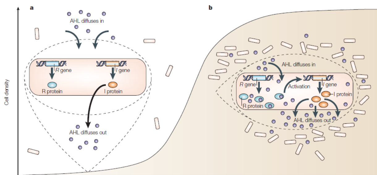
Figure 19. Mode of action of R/I QS systems. The R genes encode a transcriptional regulator and the I genes encode an AHL synthase. The AHL are synthesized, exported and accumulate in the extracellular medium. When density is high and a threshold of AHL molecules is reached, The R proteins bind to their cognate AHL forming a complex that controls the transcription of target genes. The amplification of the AHL signal is obtained by a positive feedback, resulting from the activation of I gene transcription by the complex R protein/AHL (Lazdunski, Ventre and Sturgis, 2004).
