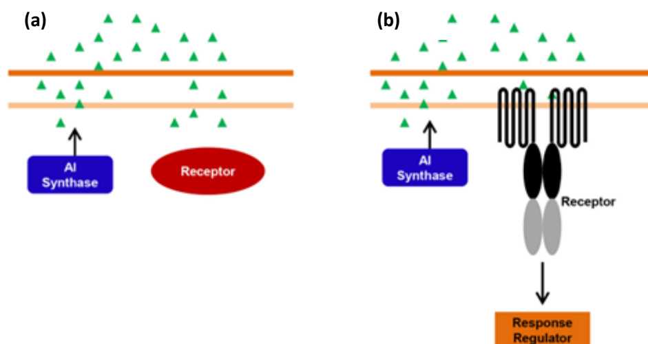
Figure 18. Quorum sensing systems in Gram-negative bacteria. One-component system (a), the autoinducers are produced and released into the extracellular medium, then they are imported back into the cytoplasm, where they are detected by QS specific sensors acting as transcriptional regulator. Two-component system (b) involves a transmembrane receptor that controls the activity of the response regulator (Hawver, Jung and Ng, 2016).
