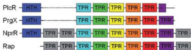
Figure 22. Schematic representation of the structure of RNPP proteins. HTH DNA binding domain, located in the N-terminal are represented in blue. The others colored boxes represent the TPR domains (six to nine) (Perchat et al. , 2011).
