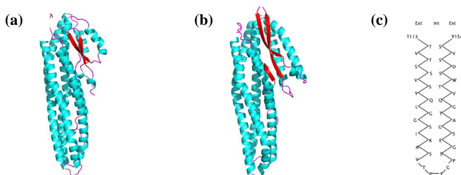
Figure 10. The structure of Hbl-B with \alpha -helices colored cyan, \beta -strands colored red and loops colored magenta (a), NheA (b) colored as in Hbl-B. Schematic representation of CytK Schematic representation of CytK. The exterior (Ext) and interior (Int) (c) (Lund, De Buyser and Granum, 2000; Ganash et al. , 2013).
