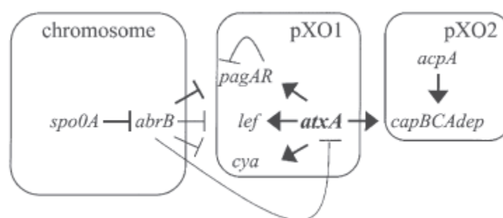
Figure 4. Virulence gene regulation of B. anthracis involving chromosomal, pXO1 and pXO2 genes. The pXO1 plasmid gene, atxA regulates positively the three anthrax toxins genes, pagA , lef , and cya , while pXO2, acpA gene regulates positively genes involved in capsule biosynthesis. Genes involved in toxins and capsule production are expressed in exponential phase. The expression of atxA , is repressed by the transitory regulator AbrB inhibiting the toxin expression before exponential phase. When cell density is higher Spo0A inhibit AbrB, allow toxin expression. Black arrows represent a positive effect and black blunt lines represent a negative effect.
