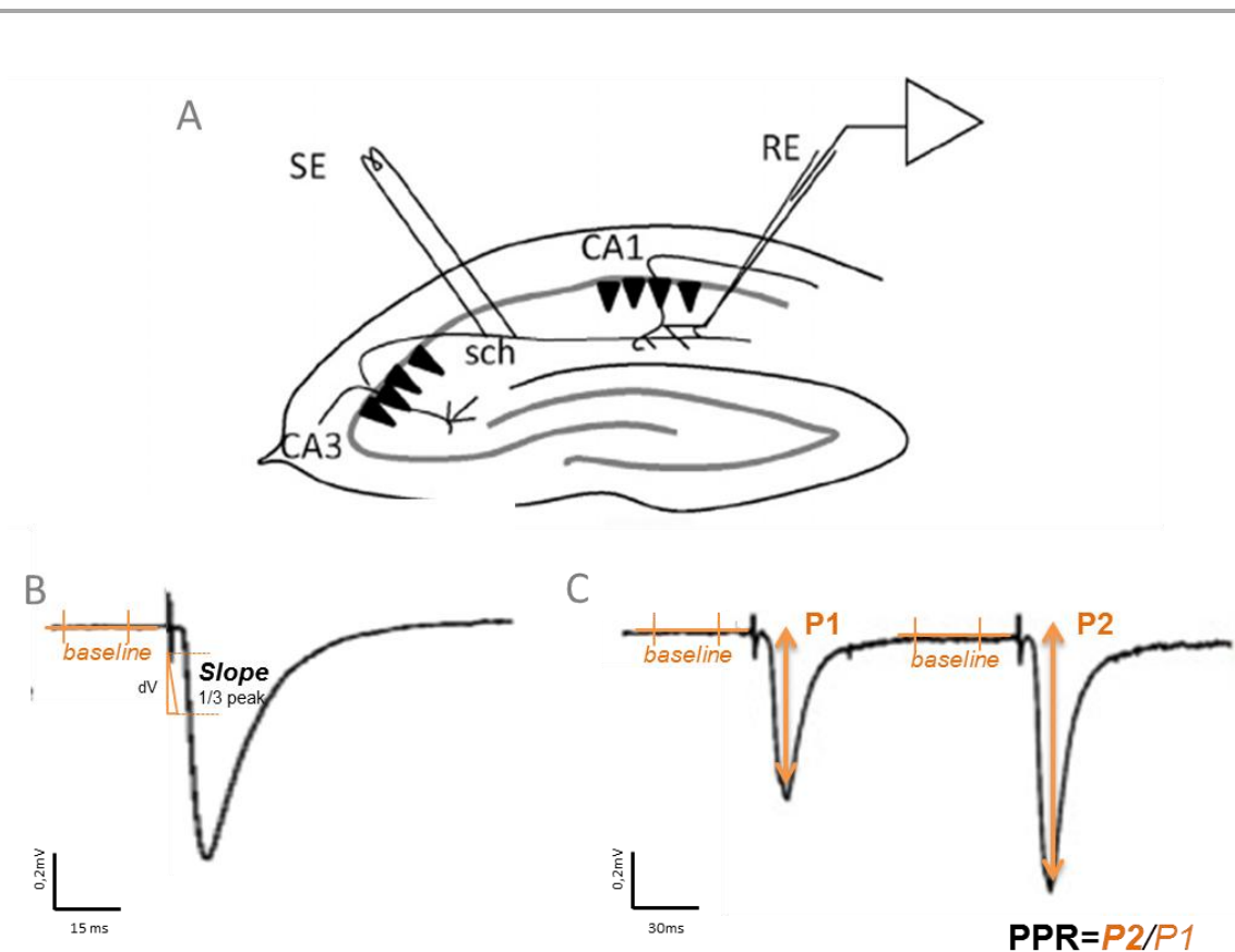
FIGURE 13. FIELD EXCITATORY POST-SYNAPTIC POTENTIALS IN THE HIPPOCAMPUS.
