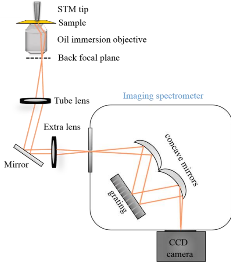
Figure 15. Schematic illustration of the experimental setup for obtaining angularly resolved spectral images.
