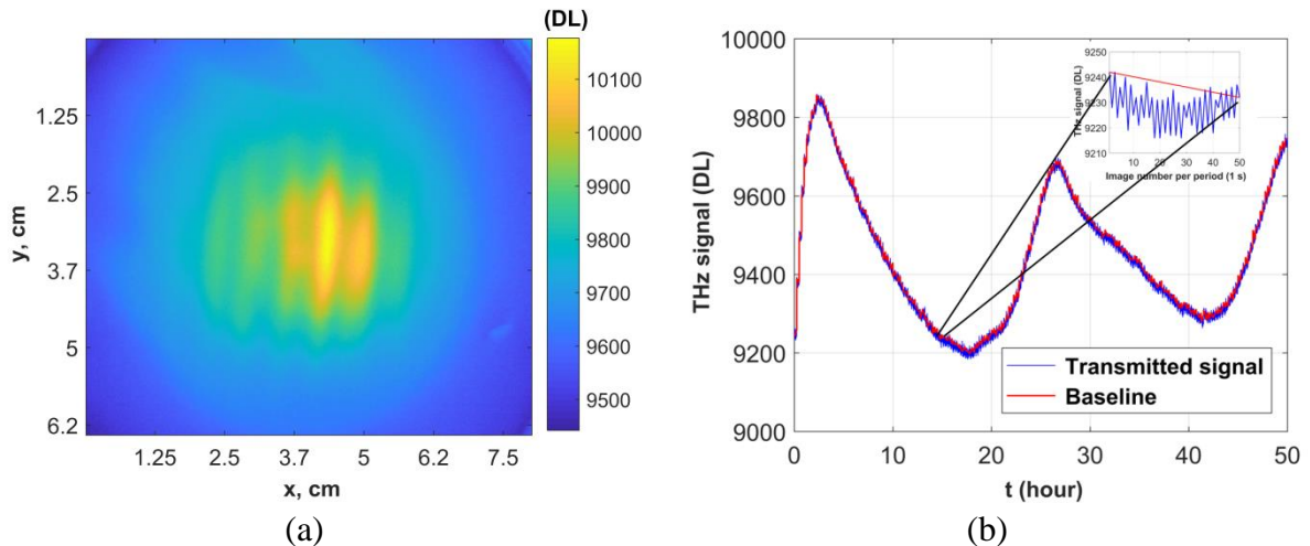
Figure 3-13: (a) Raw image of the wood sample in the near-field configuration and (b) the influence of the environment temperature on the measurement during 50 hours.
