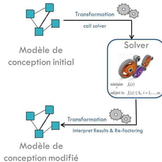
FIGURE 5.10 – Application du patron DPMP
