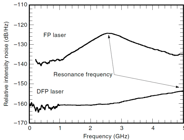
Figure 1- 16 : Spectra of relative intensity noise of a DFB and a FP laser [33].
