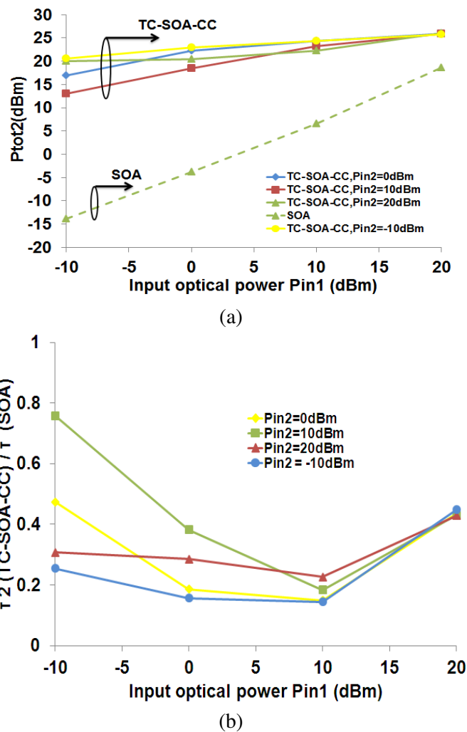
Figure 4- 27 : (a) P_{tot,2} and P_{out,SOA} as function of input optical power P_{in,1} for several values of P_{in,2} , (b) the ratio of \tau_{e2}(\text{TC-SOA-CC-IM})/\tau_e(\text{SOA-IM}) as function of P_{in,1} for several values of P_{in,2} .
