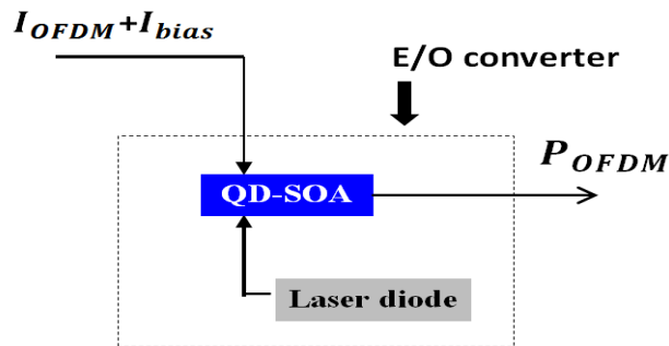
Figure 4- 7 : QD-SOA E/O converter configuration
