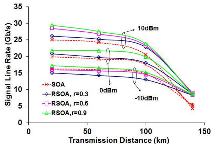
Figure 4- 6 : System capacity versus Transmission distance for SOA and RSOA
