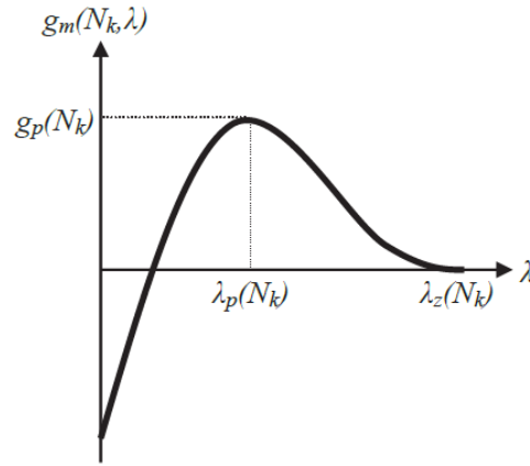
Figure 2- 3 : Plot defining the shape of the material gain g_m(N_k, \lambda) [29].
