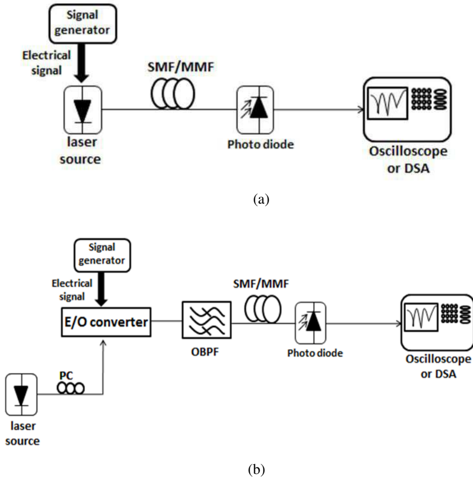
Figure 1- 13: IMDD setup, (a) direct modulation (b) external modulation, OBPF: optical band pass filter, DSA: digital signal analyzer, E/O: electrical to optical converter, PC: polarization controller.
