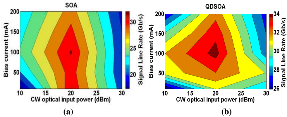
Figure 4- 11 : Contour plot of signal line rate as a function of CW optical input power and bias current after transmitting through a 60km SMF IMDD transmission system. (a) SOA-IM, (b) QD-SOA-IM.
