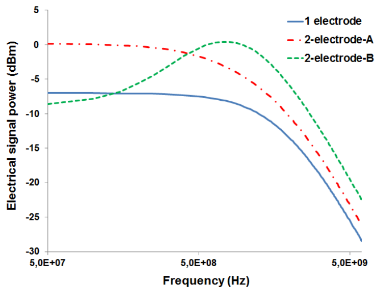
Figure 3- 29: Electrical bandwidth for the three RSOA configurations.
