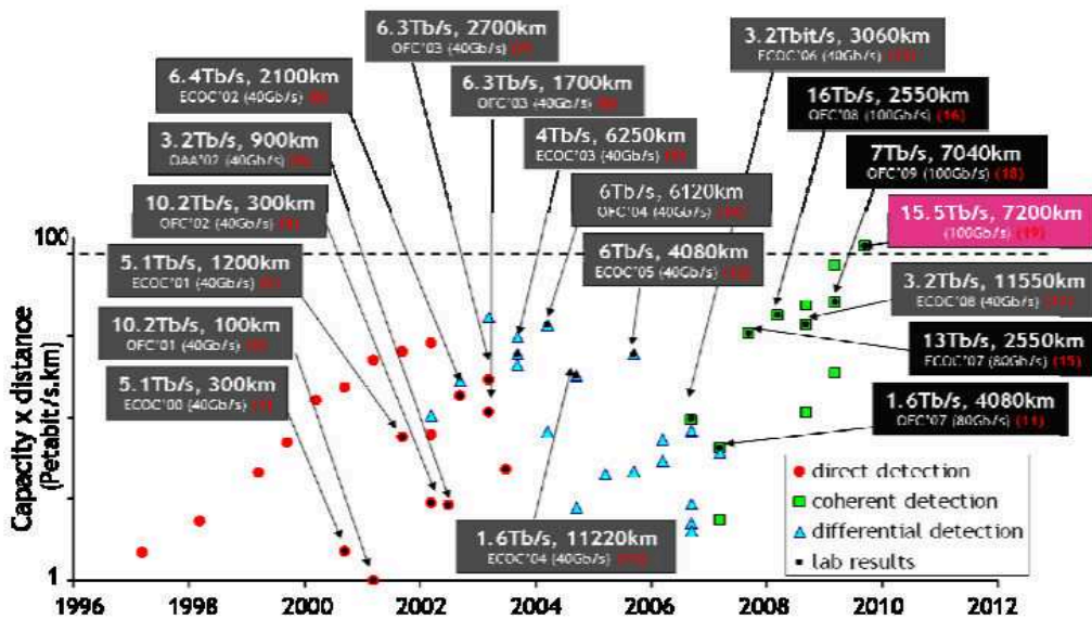
Figure 1- 3 : Capacity x distance product over the last 16 years [from Alcatel-Lucent Bell Labs].
