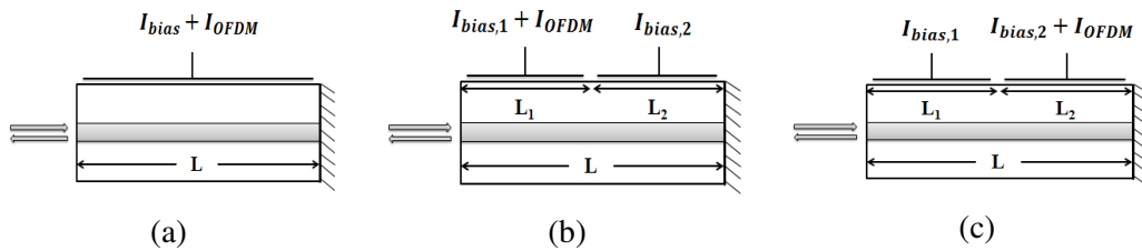
Figure 3- 28: Three studied RSOA configurations, (a) one electrode, (b) two electrodes with modulating the input section, (c) two electrodes with modulating the mirror section.
