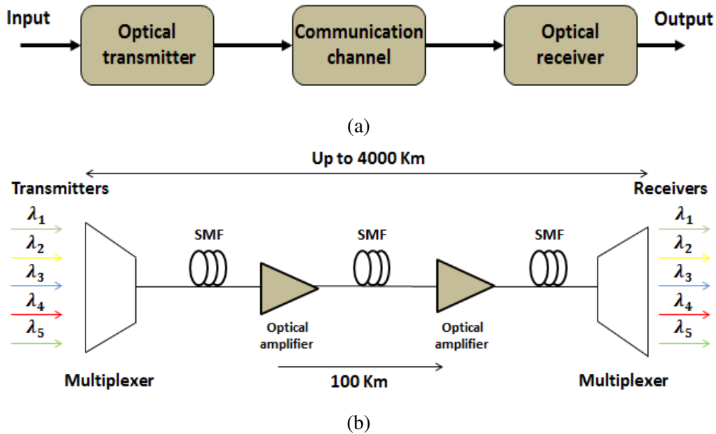
Figure 1- 4 : Schematic diagram (a) a system of optical fiber communication and (b) WDM systems.
