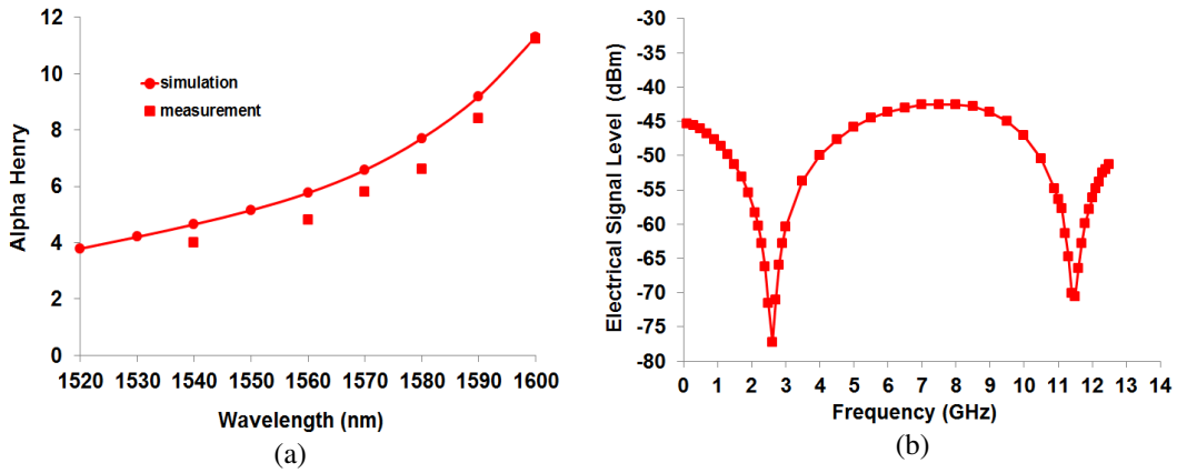
Figure 2- 16 : (a) Measurements and simulations of phase amplitude coupling factor ( \alpha_H ) versus wavelength for a bias current of 80 mA and a pump probe optical input power of -7 dBm, pump signal wavelength is 1550 nm (b) Measured frequency response of a 56 km SMF for the same conditions as in (a). The probe signal wavelength is 1560 nm.
