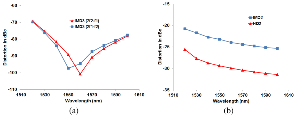
Figure 2- 20: Distortion simulation dBc values for (a) IMD3 signals (b) IMD2 and HD2, as function of wavelength for a 7 mA input AC current, Input power to the RSOA is -20 dBm, bias current is 65 mA.
