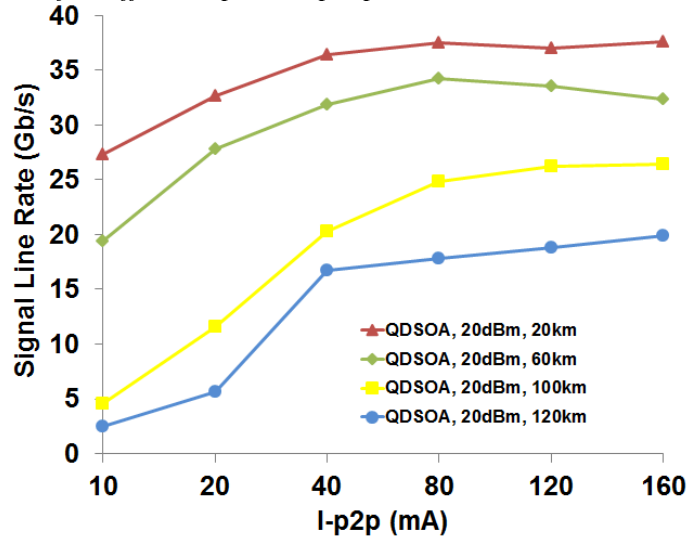
Figure 4- 14 : Signal line rate as a function of driving current PTP for different transmission distances.
