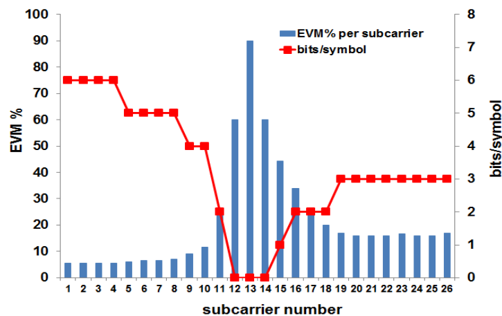
Figure 3- 27: EVM and in its corresponding bit/symbol by using AMOOFDM for each subcarrier for a transmitted signal over a 100 Km SMF.
