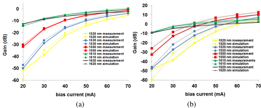
Figure 2- 5 : RSOA gain versus its bias current for different wavelength values for (a) 3.3 dBm optical input power and (b) -10 dBm optical input power.
