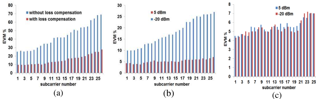
Figure 3- 16 : Numerical calculation of the EVM versus subcarrier number for a 2GHz OFDM-16 QAM signal for the cases of (a) compensating the losses in which photodetector input power is 0 dBm, and without compensating the losses, input power to the RSOA is -20 dBm. (b) For two optical input powers to the RSOA, input power to the photodetector is kept at 0 dBm and with ASE noise, and (c) same as (b) but without ASE noise.
