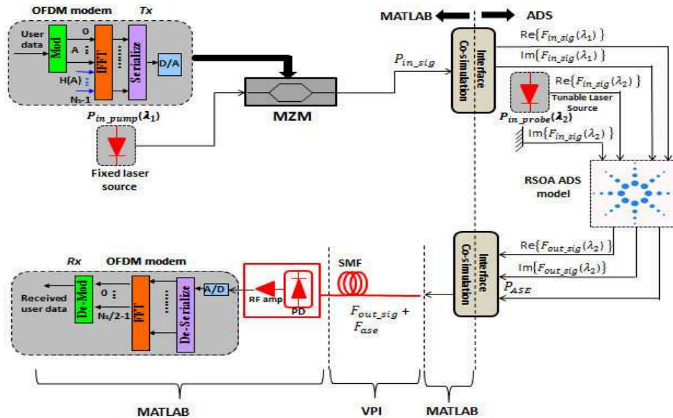
Figure 3- 33 : IM-OFDM wavelength conversion co-simulation platform using RSOA.
