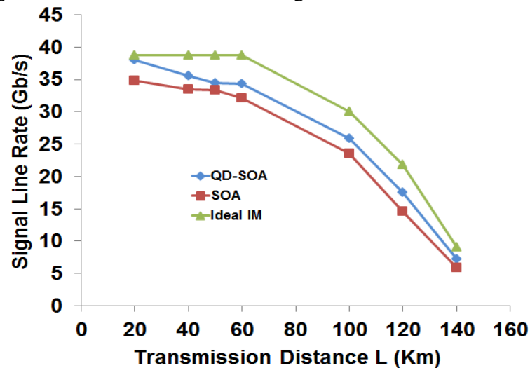
Figure 4- 15 : Maximum achievable signal transmission capacity versus reach performance of AMOOFDM signals for various intensity modulators. The optical input power is fixed at 20dBm.
