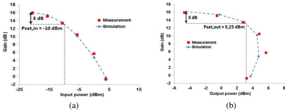
Figure 2- 10 : Numerical and experimental results of the saturation power as function of (a) the input power and (b) the output power of the RSOA. The RSOA bias current is 70 mA and the input wavelength is 1560 nm.
