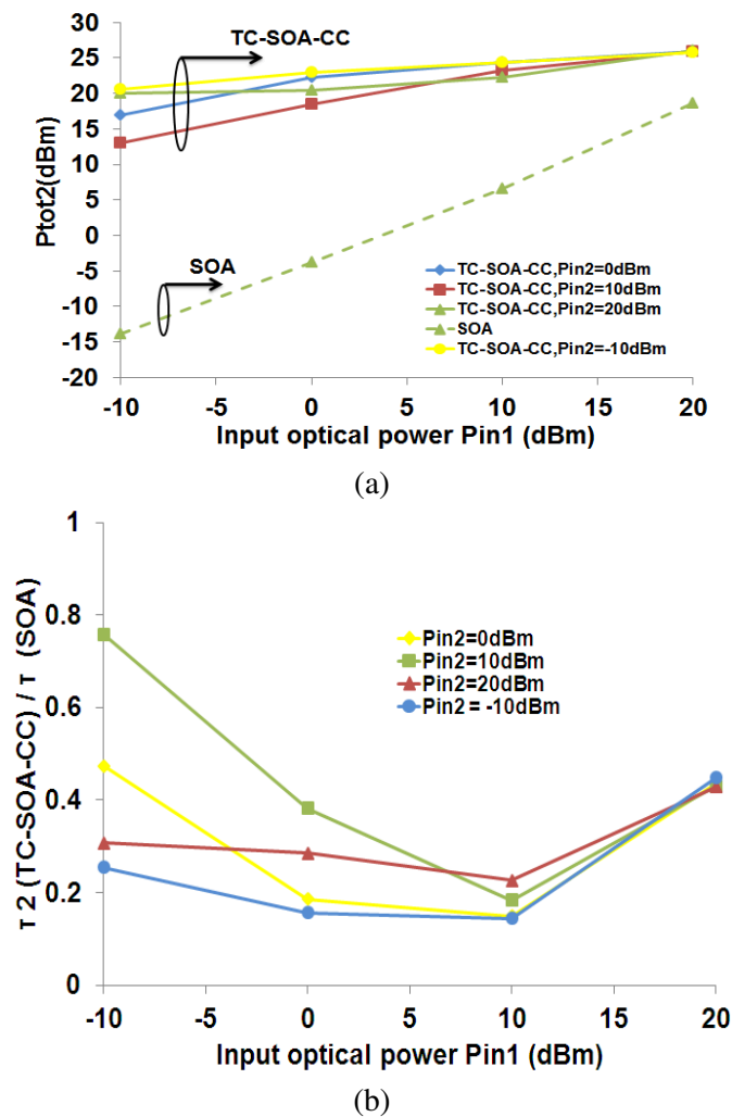
Figure 4- 27 : (a) P_{tot,2} and P_{out,SOA} as function of input optical power P_{in,1} for several values of P_{in,2} , (b) the ratio of \tau_{e2}(\text{TC-SOA-CC-IM})/\tau_e(\text{SOA-IM}) as function of P_{in,1} for several values of P_{in,2} .
