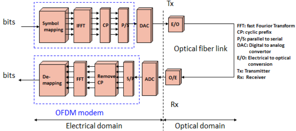
Figure a: Optical OFDM IM-DD transmission system.
