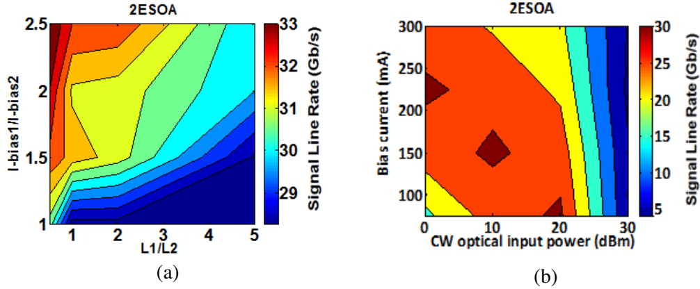
Figure 4- 21 : Contour plot of signal line rate for 2E-SOA-IM of a 60km SMF IMDD transmission system.
