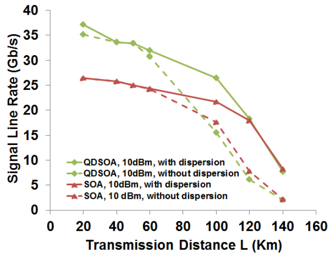
Figure 4- 18 : Signal line rate versus reach performance for cases of including and excluding chromatic dispersion. The optical input power is fixed at 10dBm.
