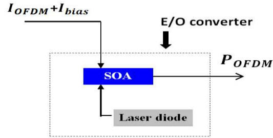
Figure 4- 3 : SOA E/O converter configuration
