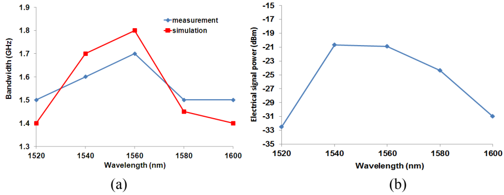
Figure 2- 15 : (a) Electrical bandwidth for RSOA in a pump probe configuration.(b) Electrical magnitude power of the probe signal at 100 MHz
