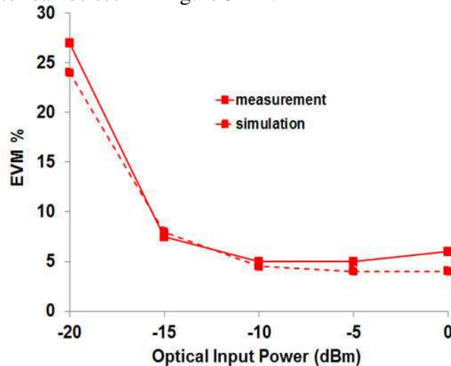
Figure 3- 12 : EVM vs optical OFDM -16 QAM 500 MHz input signal to the photodiode in an optical back to back configuration with a MZM
