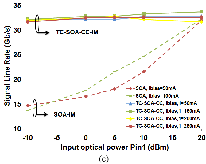
Figure 4- 29 : Signal line rate of TC-SOA-CC-IM and SOA-IM as a function of the input optical power P_{in,1} . (a) P_{in,2}=0dBm , (b) P_{in,2}=10dBm , (c) P_{in,2}=20dBm .
