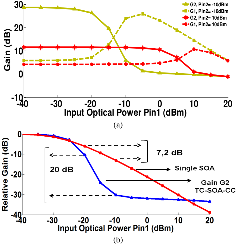
Figure 4- 25 : (a) Gains G_1 and G_2 versus the input optical power P_{in,1} with I_{bias,1} = I_{bias,2} = 280mA , (b) Relative gain G_2 versus the input optical power P_{in,1} for TC-SOA-CC and for a single SOA with I_{bias,1} = I_{bias,2} = 280mA
