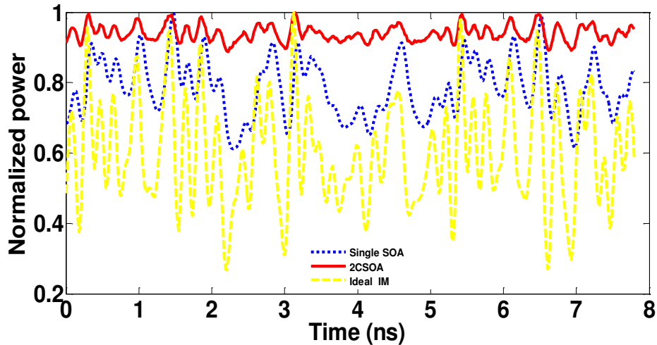
Figure 4- 31 : Normalized AMOOFDM signal waveforms generated by a TC-SOA-CC-IM, single SOA-IM and ideal-IM
