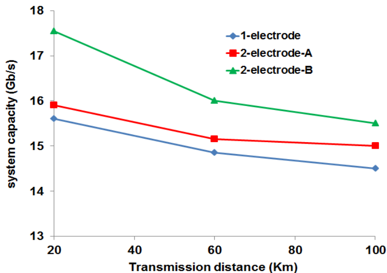
Figure 3- 31: System capacity versus transmission distance for the three RSOA configurations.
