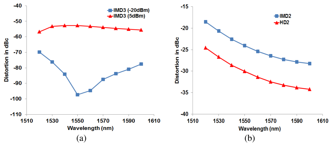
Figure 2- 21: Distortion simulation dBc values for (a) IMD3 signals (b) IMD2 and HD2, as function of wavelength for a 7 mA input AC current, Input power to the RSOA is 5 dBm, bias current is 65 mA.(for case (a) we have two input powers).
