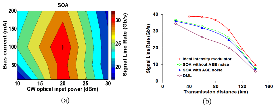
Figure 4- 4 : (a) SOA performance versus bias current and optical input power (b) transmission capacity versus distance for Ideal IM, SOA, and DFB laser configurations.
