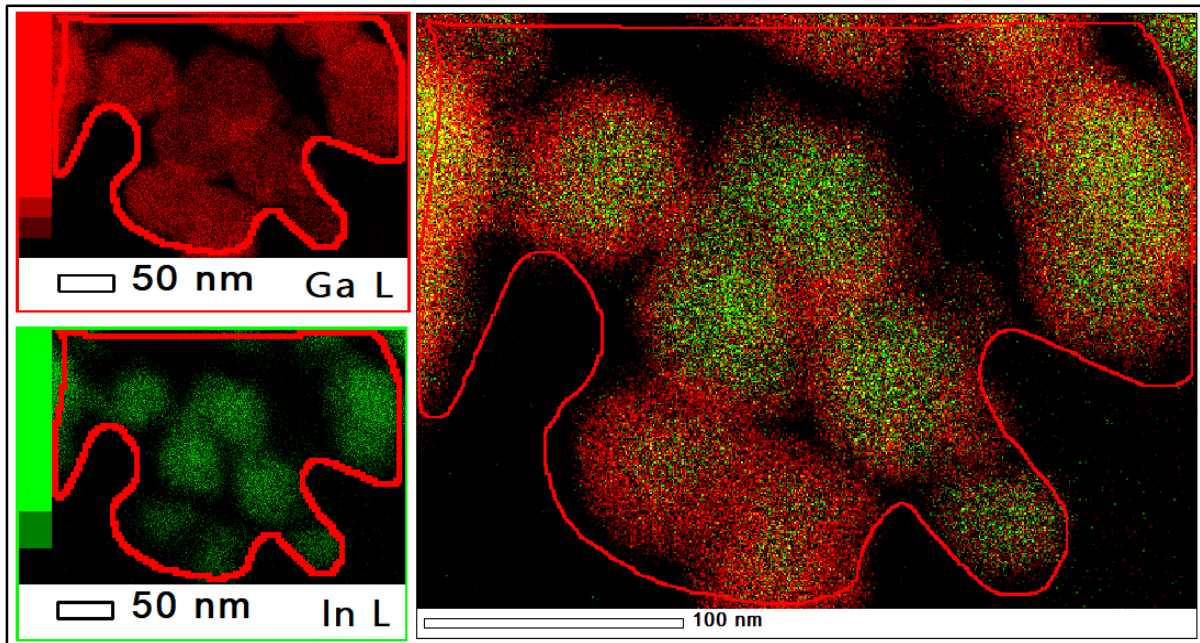
Figure 3.9. Elemental mapping of Ga_{0.84}In_{0.16}N solid solution nanomaterial synthesized through continuous flow millireactor in supercritical toluene, this particular image corresponds to region depicted in STEM image of Figure 3.7.b.
