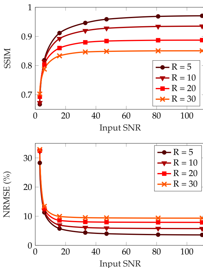
FIGURE 2.5: For a constant image size N = 1024 , evolution of A) SSIM scores and B) NRMSE scores as a function of input SNR, for different acceleration factors of 5, 10, 20 and 30, in the case of analytical images reconstructed from iid-undersampled data. For both metrics, as the input SNR increases, the image quality improves and approaches its limit. A stationary regime is reached for high input SNR, where SSIM and NRMSE scores are approximately equal to their maximum and minimum values respectively for a given acceleration factor.
