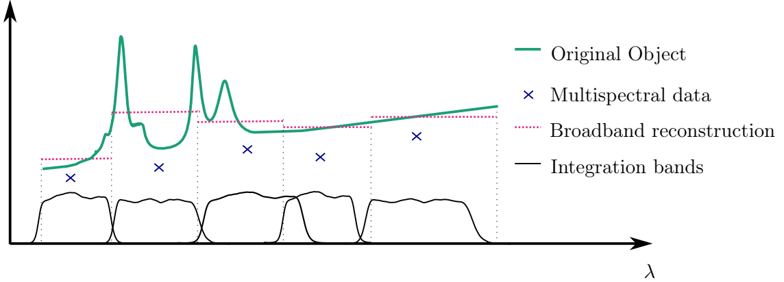
Figure 4.1: Inaccuracy of the broadband reconstruction method illustrated on five low-resolution multispectral data. The spectral distribution of the original object of interest is illustrated for a single spatial position over the wavelength range.
