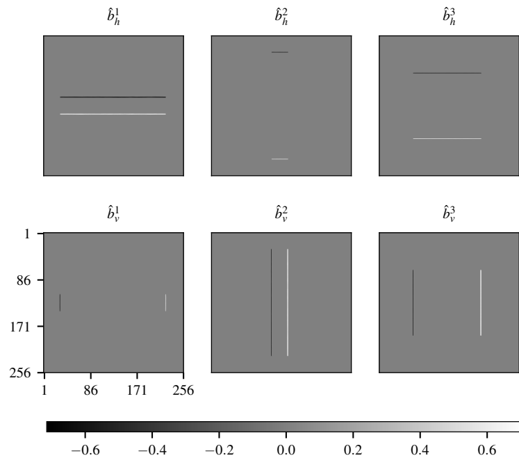
Figure 5.20: Estimated auxiliary variables for the object Synthetic 1 after 50 iterations with a threshold parameter s = 0.03 and a 30 dB multispectral data.
