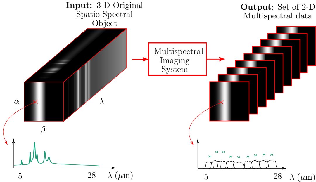
Figure 1.1: Illustration of the input and output for a multispectral imaging system such as the imager MIRI of the JWST [Bouchet et al. 2015]. The input is a 2\text{D}+\lambda continuous object having spatial and spectral distributions and the output a set of 2\text{D} low-resolution multispectral data degraded by the instrument response.
