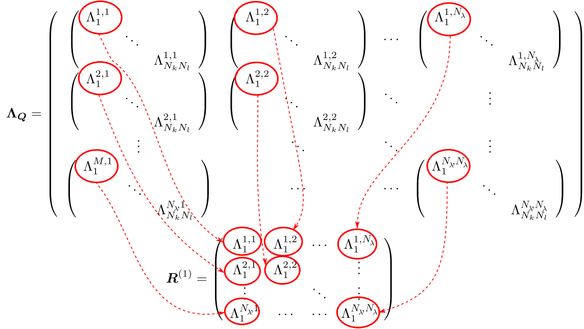
Figure 4.3: Illustration of the extraction procedure of \mathbf{R}^{(1)} for the inversion of a non-diagonal bloc-diagonal matrix \mathbf{\Lambda}_Q .
