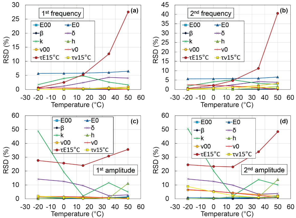
Figure 4.3. RSD in function of temperature for each of the ten constants of the 2S2P1D model for the longitudinal mode of the cylinder: (a) 1 st resonance frequency; (b) 2 nd resonance frequency; (c) 1 st resonance amplitude; (d) 2 nd resonance amplitude.
