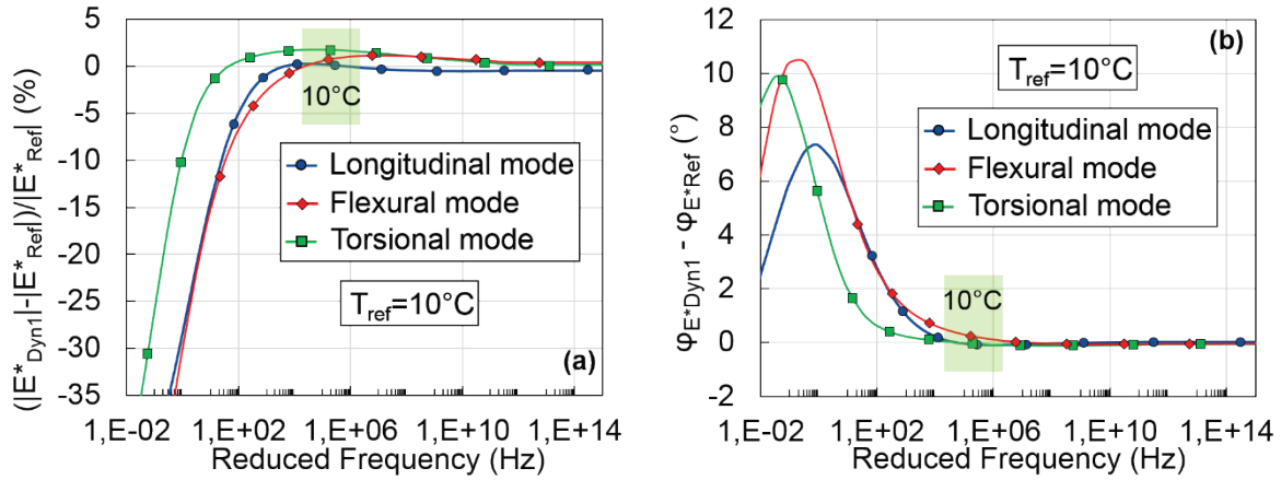
Figure 4.8. Master curve at 10°C of: (a) the relative difference between the norm of the complex modulus determined with method I ( |E_{DynI}^*| ) and of the reference LVE material ( |E_{Ref}^*| ); (b) the difference between the phase angle of the complex modulus determined with method I ( \varphi_{E_{DynI}^*} ) and of the reference LVE material ( \varphi_{E_{Ref}^*} ). Results for three studied modes of vibrations.
