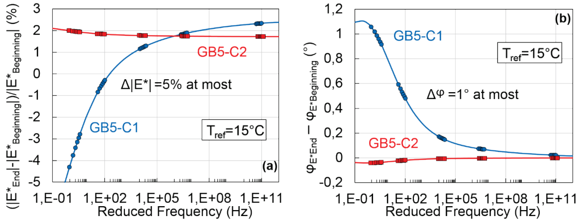
Figure 5.12 (a) Relative difference in % at 15^\circ\text{C} between the norm of the complex modulus evaluated from dynamic tests at the end ( |E^*_{End}| ) and at the beginning ( |E^*_{Beginning}| ) of the FSDyn project for the two GB5 cylinders; (b) Difference in ° at 15^\circ\text{C} between the phase angle of the complex modulus evaluated from dynamic tests at the end ( \phi_{E^*_{End}} ) and at the beginning ( \phi_{E^*_{Beginning}} ) of the FSDyn project for the two GB5 cylinders.
