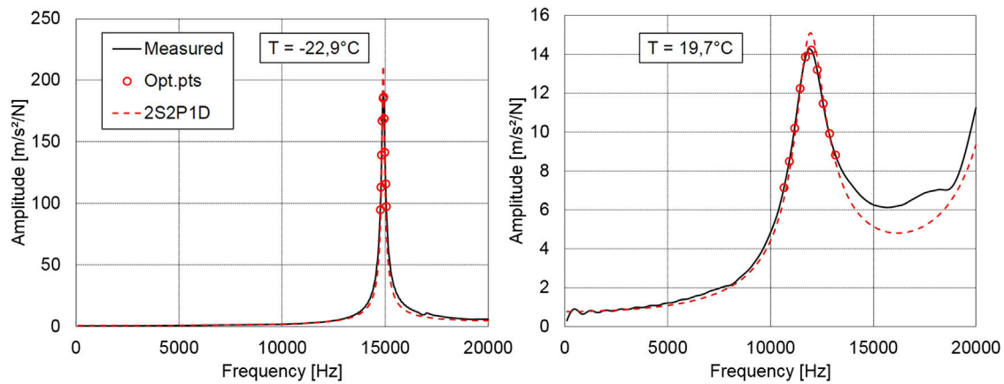
Fig. 9. Measured and optimized FRFs for specimen 4. (left) at -22.9^{\circ}\text{C} ; (right) at 19.7^{\circ}\text{C} .
