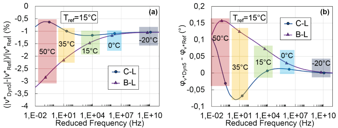
Figure 4.29. Master curve at 15°C of: (a) the relative difference between the norm of the complex Poisson's ratio determined with method V ( |v^*_{Dyn5}| ) and of the reference LVE material ( |v^*_{Ref}| ); (b) the difference between the phase angle of the complex Poisson's ratio determined with method V ( \phi_{v^*_{Dyn5}} ) and of the reference LVE material ( \phi_{v^*_{Ref}} ). Results for the two studied configurations.
