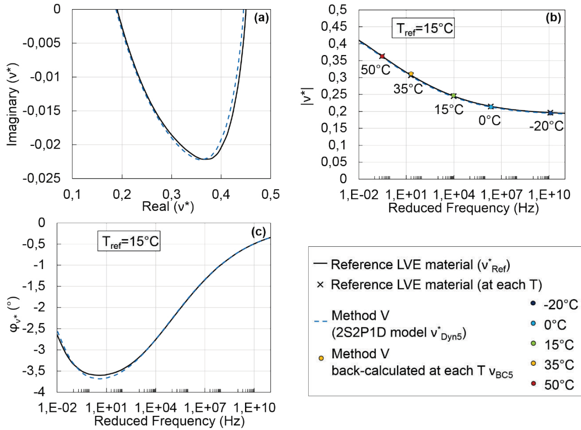
Figure 4.28. Comparison of the values of the complex Poisson's ratio determined with methods V (real values v_{BC5} and v^*_{Dyn5} ) with the values of the complex Poisson's ratio of the reference LVE material ( v^*_{Ref} ). (a) Cole-Cole plot; (b) and (c) master curves of the norm and of the phase angle of the complex modulus at 15°C. Results for the longitudinal mode of the cylinder.
