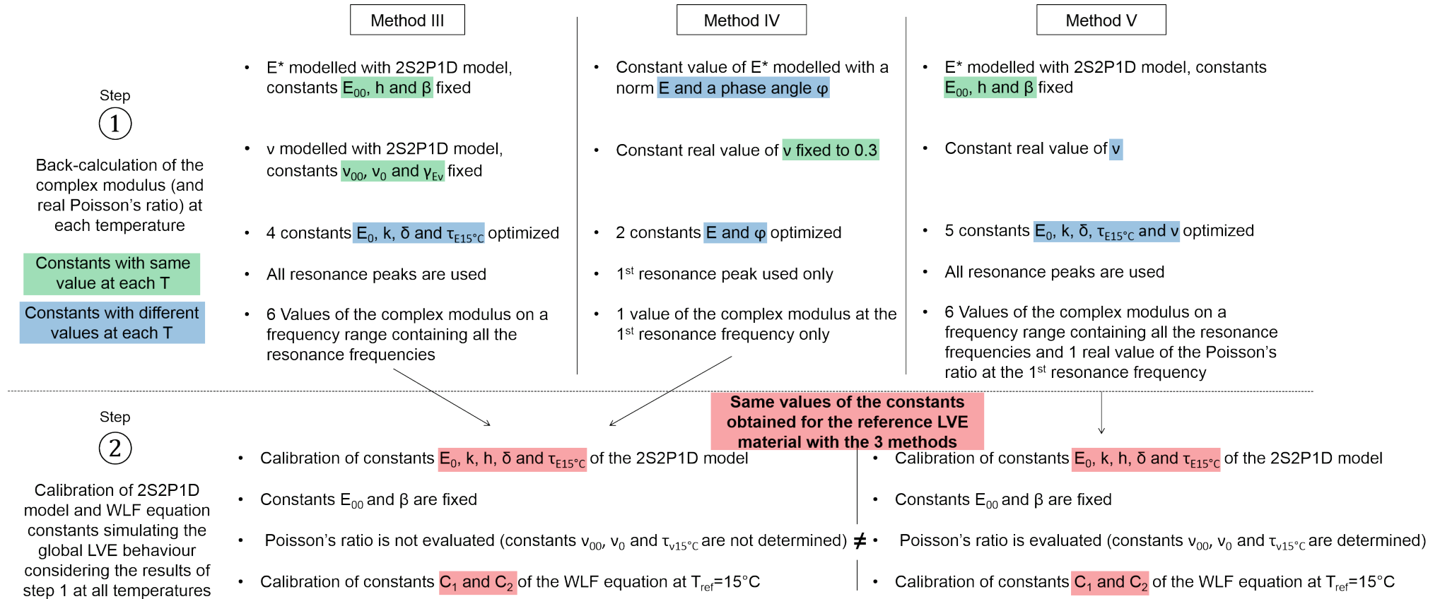
Figure 4.30. Comparison of methods III, IV and V. Values of constants noted as fixed are set to the values of the reference LVE material or to values determined from other tests.
