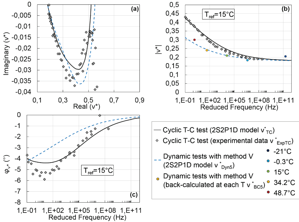
Figure 5.26 Comparison of the values of the complex Poisson's ratio determined from dynamic tests with method V (real values v_{BC5} and v_{Dyn5} ) with the values of the complex Poisson's ratio determined from cyclic test ( v_{ExpTC} and v_{TC} ). (a) Cole-Cole plot; (b) and (c) master curves of the norm and of the phase angle of the complex Poisson's ratio at 15°C. Results for specimen WF-8.
