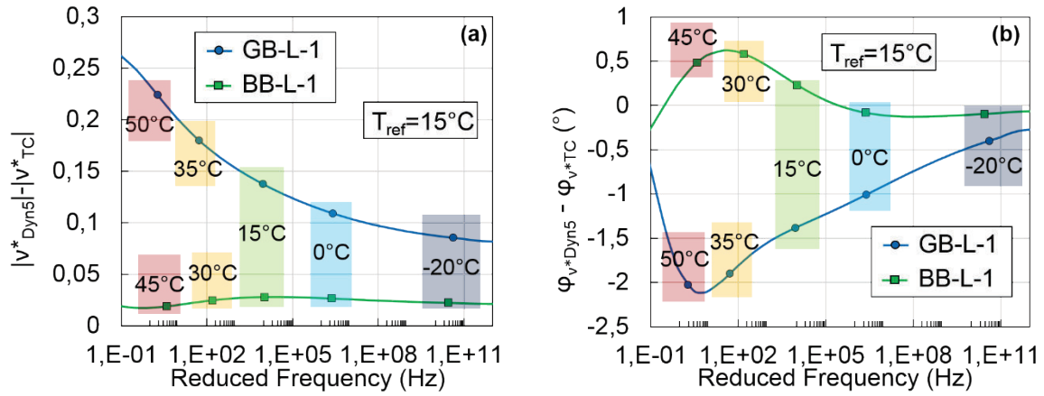
Figure 5.33 Master curve at 15°C of: (a) the relative difference between the norm of the complex Poisson's ratio determined from dynamic tests with method V ( |v_{Dyn5}^*| ) and from cyclic tests ( |v_{TC}^*| ); (b) the difference between the phase angle of the complex Poisson's ratio determined from dynamic tests with method V ( \varphi_{v^*Dyn5} ) and from cyclic tests ( \varphi_{v^*TC} ). Results for the GB-L-1 and BB-L-1 cylinders tested in the MAP experimental campaign.
