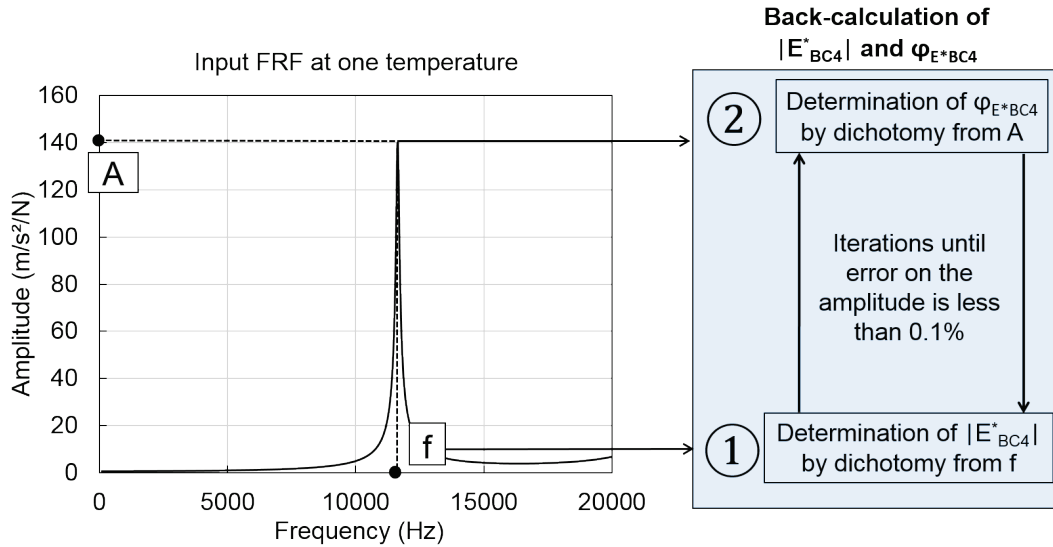
Figure 4.20. Principle of the back-calculation of the norm ( |E^*_{BC4}| ) and phase angle ( \phi_{E^*_{BC4}} ) of the complex modulus at each temperature from the first resonance frequency in the first step of method IV.
