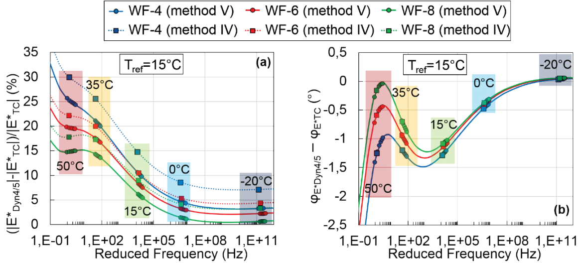
Figure 5.25 Master curve at 15^\circ\text{C} of: (a) the relative difference between the norm of the complex modulus determined from dynamic tests with method IV/V ( |E^*_{Dyn4/5}| ) and from cyclic tests ( |E^*_{TC}| ); (b) the difference between the phase angle of the complex modulus determined from dynamic tests with method IV/V ( \varphi_{E^*_{Dyn4/5}} ) and from cyclic tests ( \varphi_{E^*_{TC}} ). Results for the WF specimens tested in the MHRAPC experimental campaign.
