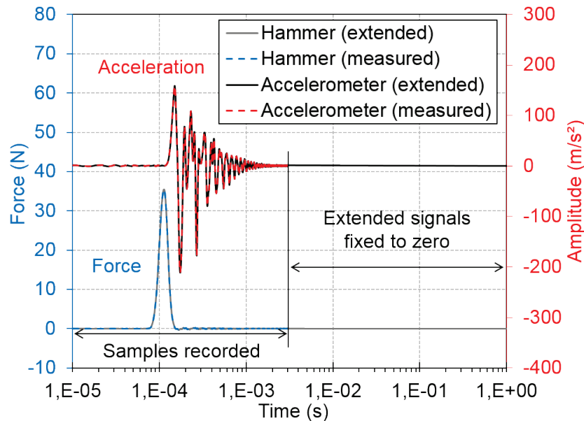
Figure 3.12. Example of measured and extended signals of the impact hammer and accelerometer in time domain.
