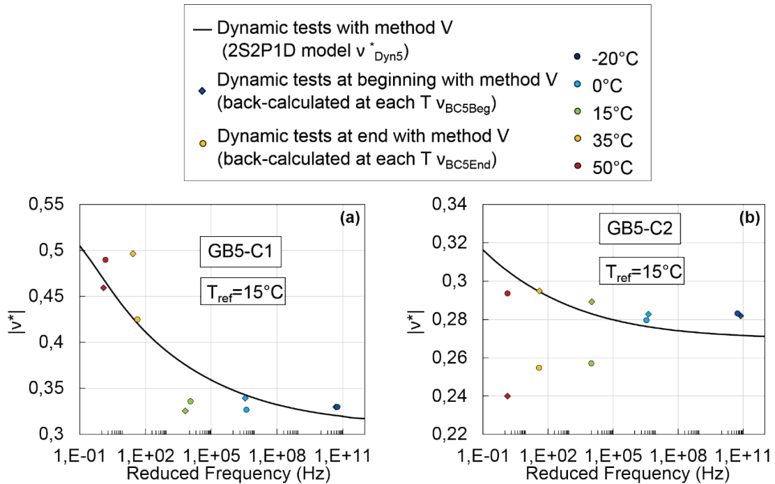
Figure 5.13 (a) Master curves at 15^\circ\text{C} of the real values of the Poisson's ratio back-calculated at each temperature from dynamic tests with method V at the beginning ( v_{BC5Beg} ) and at the end (noted v_{BC5End} ) of the FSDyn project. The master curves of the norm of the complex Poisson's ratio determined from dynamic tests with method V ( v^*_{Dyn5} ) are also plotted. (a) Specimen GB5-C1; (b) Specimen GB5-C2.
