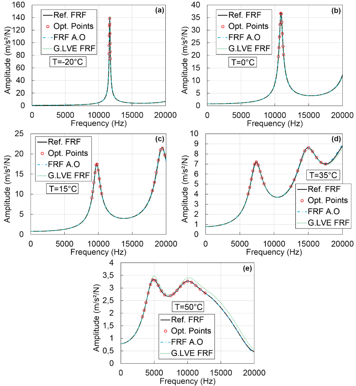
Figure 4.16. Comparison of the reference FRFs (noted Ref. FRF) with the FRFs after optimization (noted FRF A.O) and the global LVE FRFs (noted G.LVE FRF) for method III. Values of the reference FRFs at the frequencies where the optimization is performed (noted Opt. Points) are also plotted. Example for the longitudinal mode of the cylinder at: (a) -20^{\circ}\text{C} ; (b) 0^{\circ}\text{C} ; (c) 15^{\circ}\text{C} ; (d) 35^{\circ}\text{C} ; (e) 50^{\circ}\text{C} .
