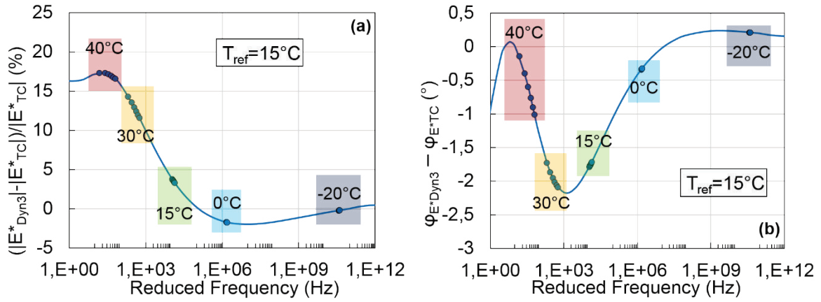
Figure 5.16 Master curve at 15^\circ\text{C} of: (a) the relative difference between the norm of the complex modulus determined from dynamic tests with method III ( |E_{Dyn3}^*| ) and from cyclic tests ( |E_{TC}^*| ); (b) the difference between the phase angle of the complex modulus determined from dynamic tests with method III ( \varphi_{E^*Dyn3} ) and from cyclic tests ( \varphi_{E^*TC} ). Results for the ABS-P4 beam tested in the SM experimental campaign.
