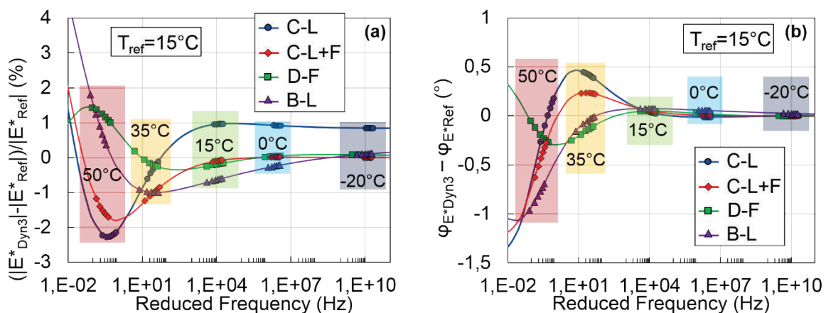
Figure 4.18. Master curve at 15°C of: (a) the relative difference between the norm of the complex modulus determined with method III ( |E^*_{Dyn3}| ) and of the reference LVE material ( |E^*_{Ref}| ); (b) the difference between the phase angle of the complex modulus determined with method III ( \phi_{E^*_{Dyn3}} ) and of the reference LVE material ( \phi_{E^*_{Ref}} ). Results for the four studied configurations.
