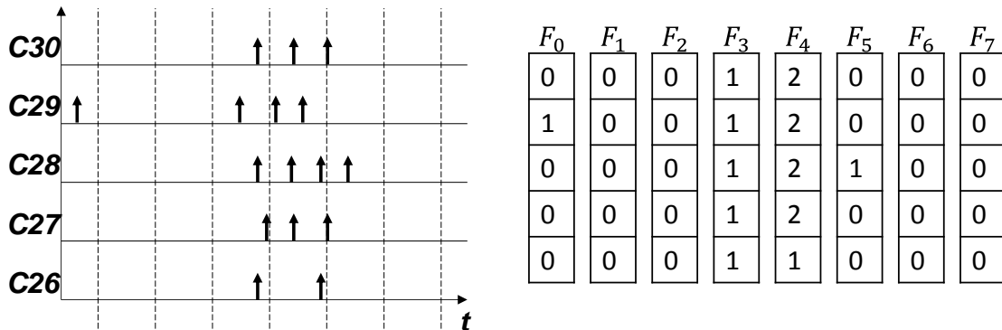
Figure 5.11: Constant time bins features: for each 5 ms window, count the number of event per channel and create an input vector.
