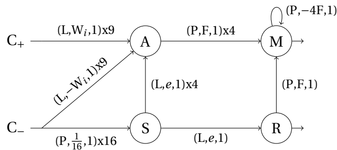
Figure 5.6: Convolution + pooling unit. The synchronization neuron (S) uses the second spike from the 16 input pixel in the max pooling zone. The spikes from the accumulators (A) are directly sent to the neuron (M) performing the maximum operation with the null signal being sent from (R).
