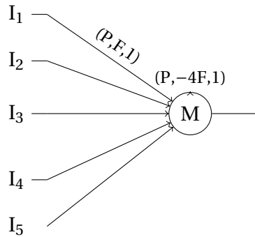
Figure 5.5: 5-input maximum operator used as max pooling unit. 5 neurons will stimulate M for each operation. The first stimulation makes it spike and inhibit itself. The 4 other stimuli reset the neuron to its rest potential.
