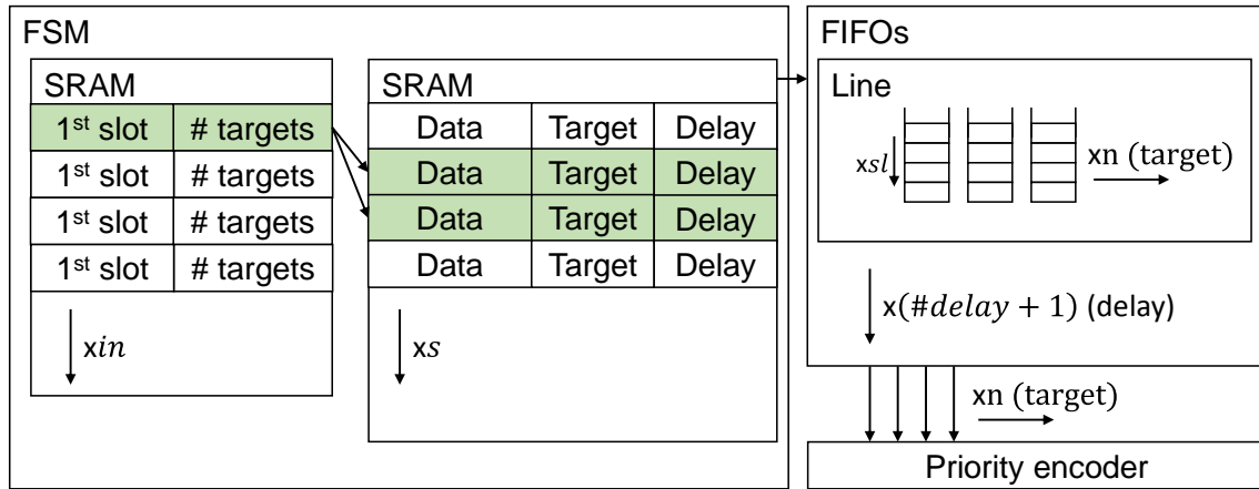
Figure 3.8: SRAMs + FIFOs implementation enables flexible connectivity.
