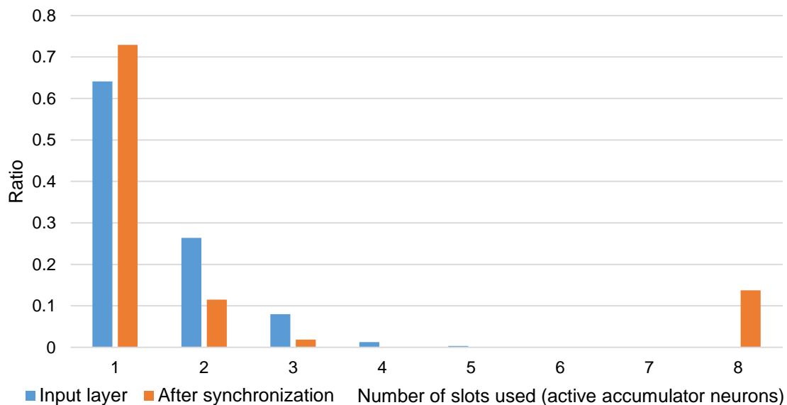
Figure 3.18: FIFO slots used for active accumulator neurons for 8 inputs, at network input vs after synchronization.
