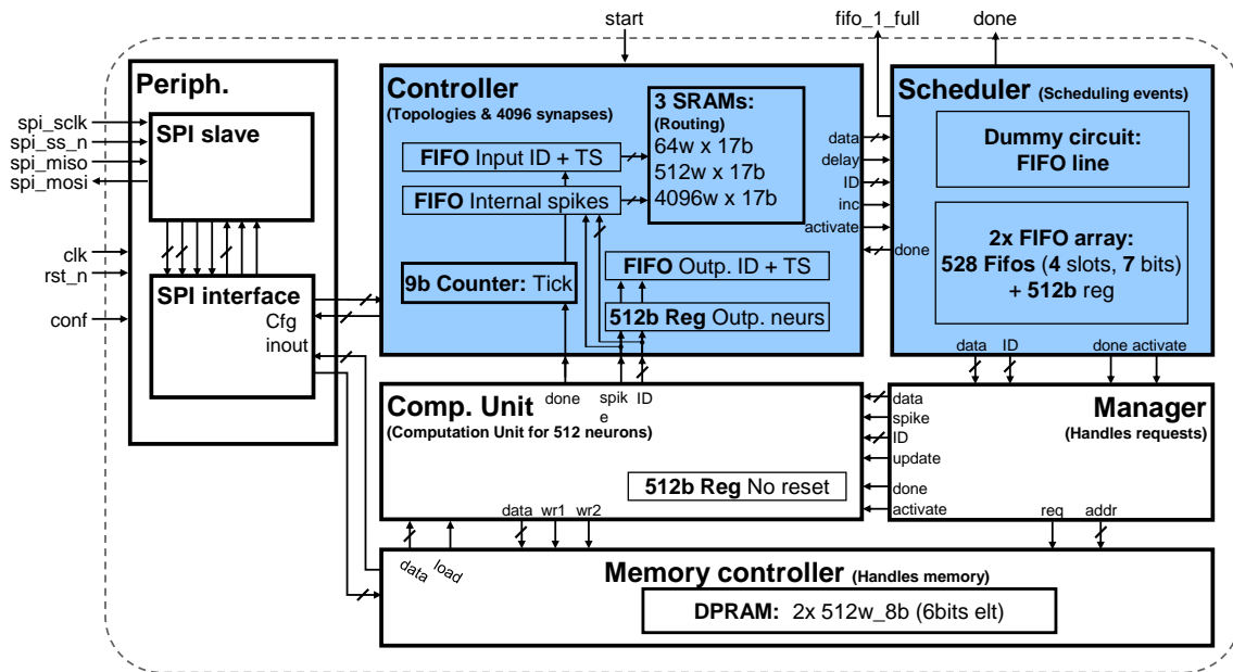
Figure 4.1: Micro architecture of INSPIRE.
