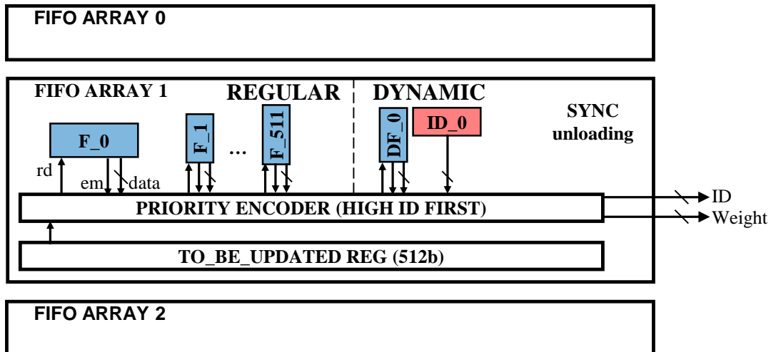
Figure 4.4: Synchronous retrieving of the synaptic stimuli when the simulation step is changed. Starts with the highest ID and sends in order stimuli to the Manager. The “To Be Updated” register represents neurons that have to be updated at this simulation tick: either neurons receiving stimuli or neurons having active linear synapse(s).
