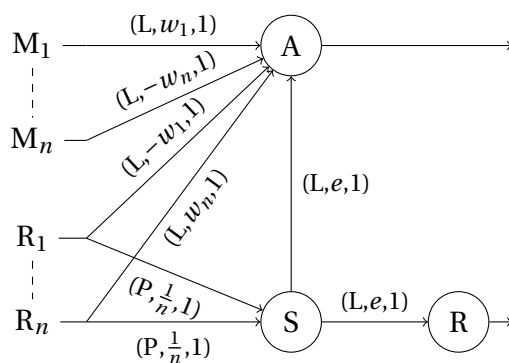
Figure 5.7: Topology used for FC layer computation.
