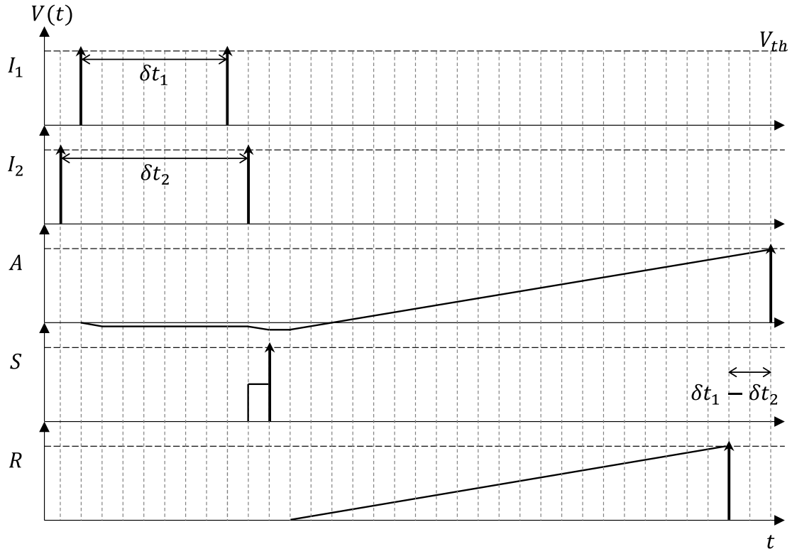
Figure 2.17: Subtraction chronogram.
