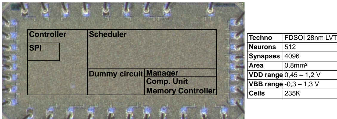
Figure 4.6: Chip characteristics.
