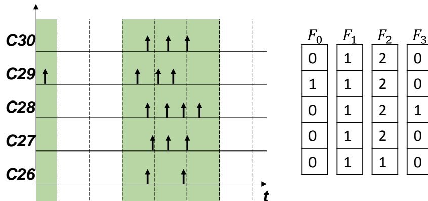
Figure 5.12: Event Driven Constant time bins features: for each 5 ms window, count the number of event per channel and create an input vector if not empty (green).
