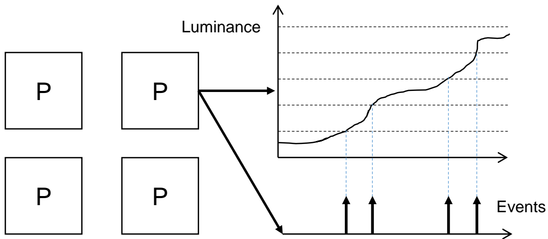
Figure 1.1: Luminance change events produced by a dynamic pixel in DVS.
