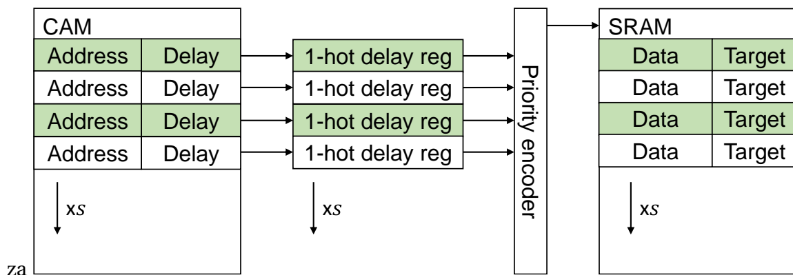
Figure 3.7: CAM oriented synapses handling enables flexible connectivity.
