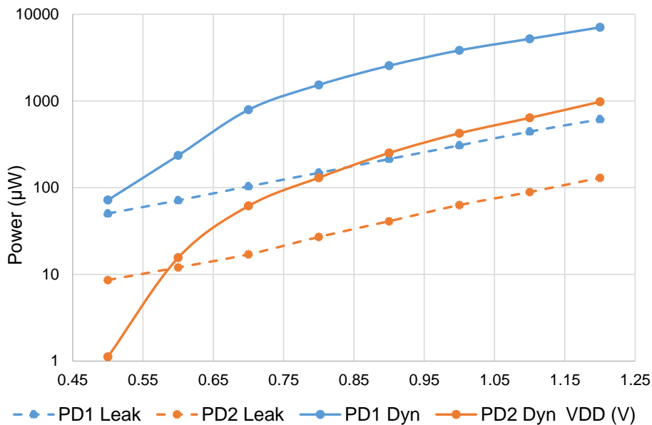
Figure 4.11: Power breakdown @-0.3VBB. The Power Domain 1 (PD1) (SPI + Controller + Scheduler) dominates the power consumption of the chip.
