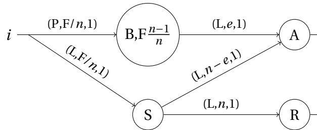
Figure B.1: Operator used to average n consecutive intervals.
