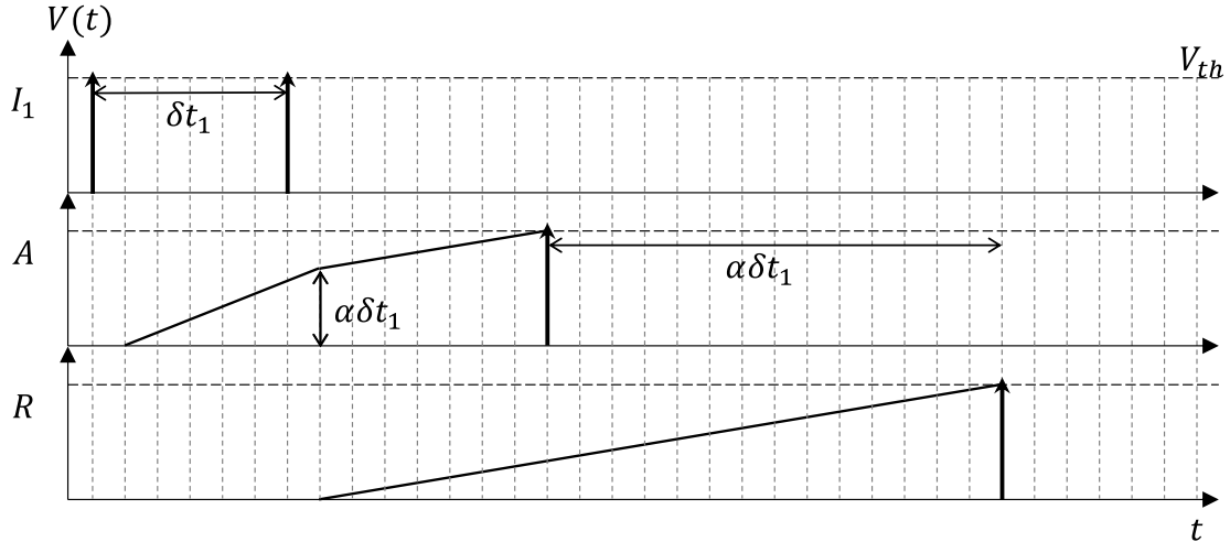
Figure 2.19: Multiplication chronogram.
