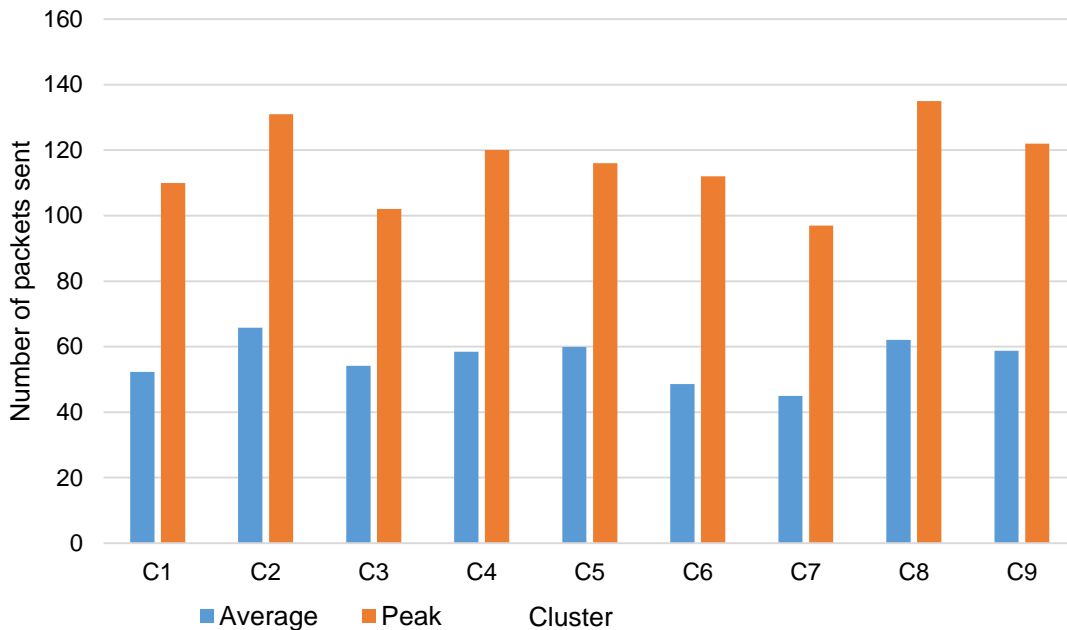
Figure 3.17: ANOC average and peak load, influence per cluster.
