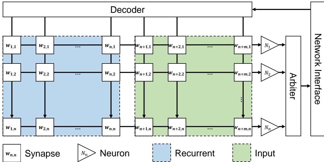
Figure 3.6: Synapse matrix enables high connectivity.
