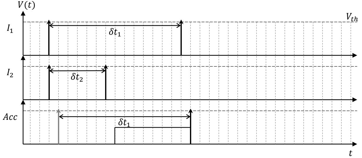
Figure 2.23: Maximum chronogram.
