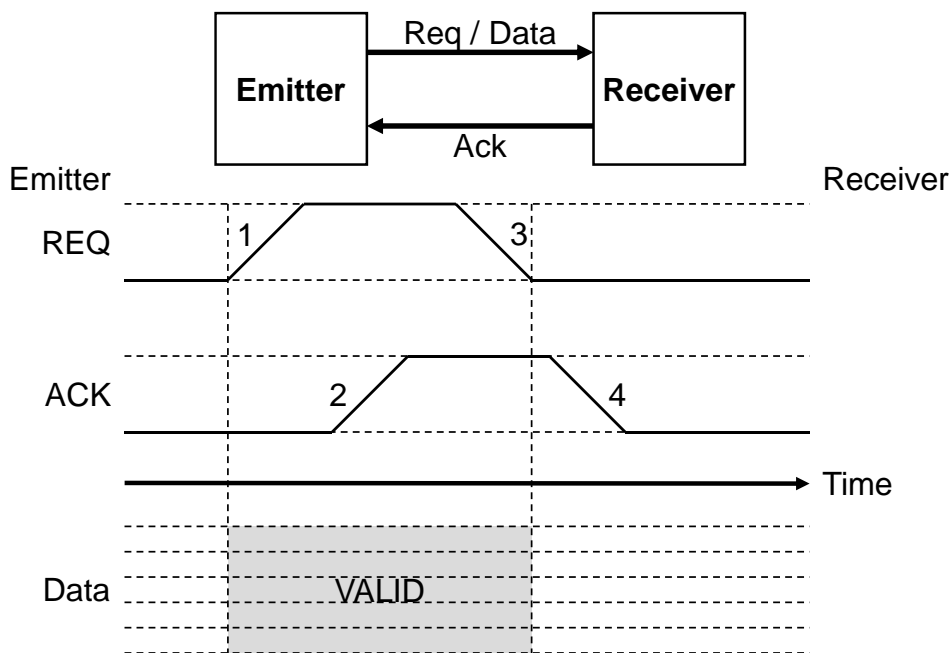
Figure 3.2: 4-phases handshake. Data is guaranteed valid in-between REQ and ACK being pulled up.
