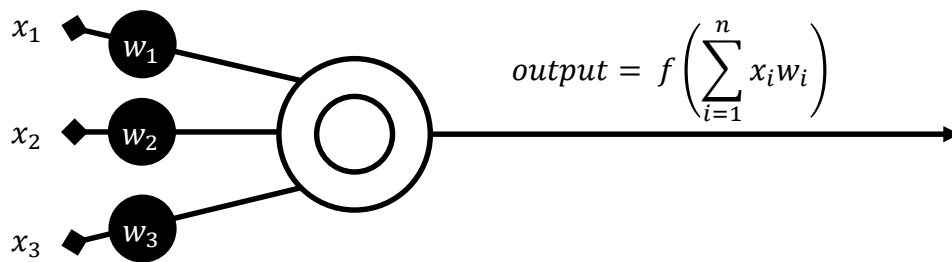
Figure 1.5: Perceptron: neuron model using normalized firing rates as data.
