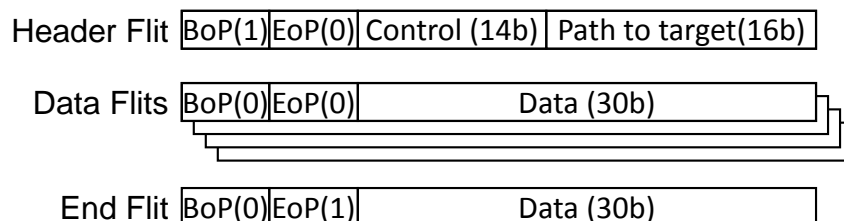
Figure 3.3: Packet composed of 2 flits of 32 bits.
