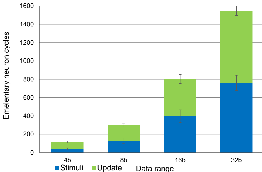
Figure 4.12: Computation unit cycles used and synaptic energy per operation versus accuracy.
