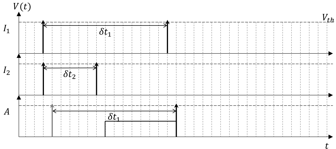
Figure 2.21: Synchronization chronogram.
