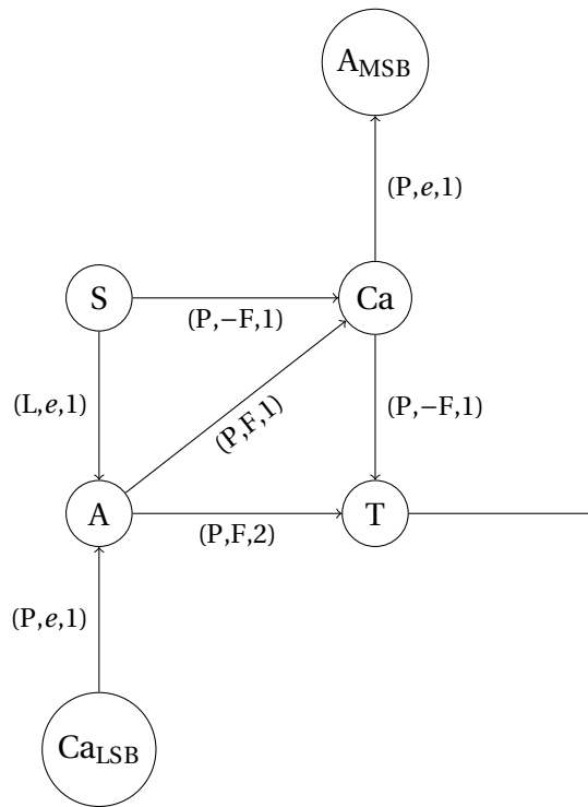
Figure B.8: Logic used to transmit carries as long as the synchronization neuron S does not spike.
