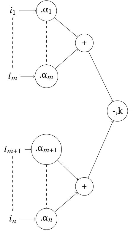
Figure 2.24: Full Linear Combination implementation using frequency coded operators.
