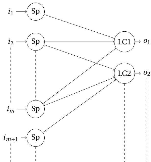
Figure 4.8: Array of Linear combination used for testing the INSPIRE chip.
