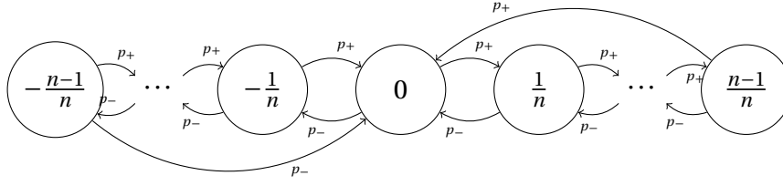
Figure 2.9: Markov process handling subtraction neuron's states.
