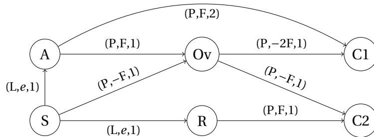
Figure 2.30: Overflow detection and filtering setting up a race between A and S. F weights denotes the full threshold potential. S spiking first inhibits the Overflow neuron Ov . A spiking first makes Ov spike to signal overflow.
