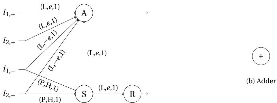
(a) Splitting input spike train into 2 spike trains holding interval information. e stands for elementary weight. + inputs holds the first spike and - the second one for each interval.
