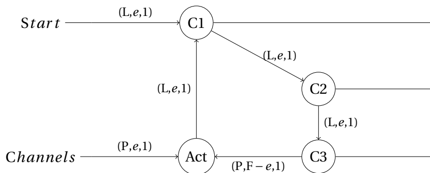
Figure 5.18: A condition is added to the Control Loop. The loop will continue only if it received at least one input spike. If it didnt receive any it will stop and wait for activity.
