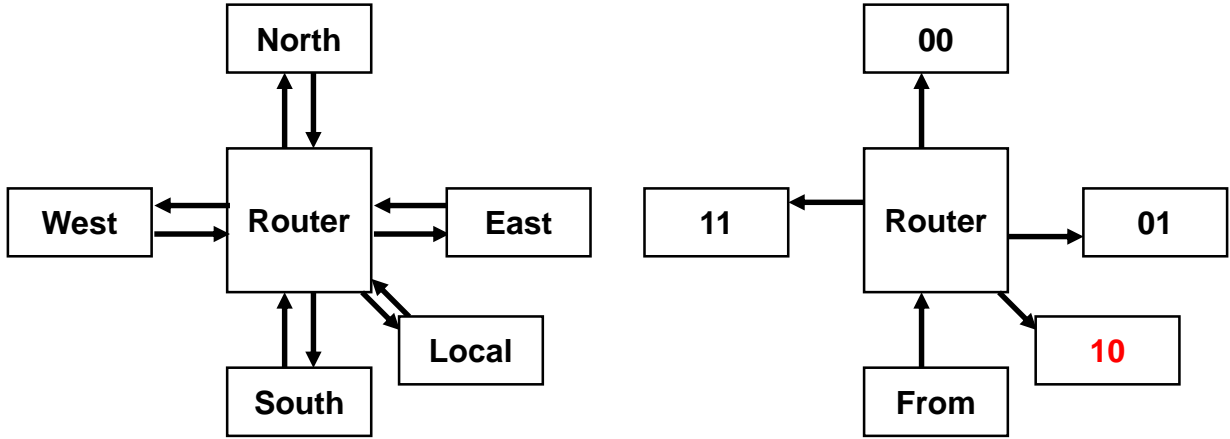
Figure 3.4: PTT explained.
