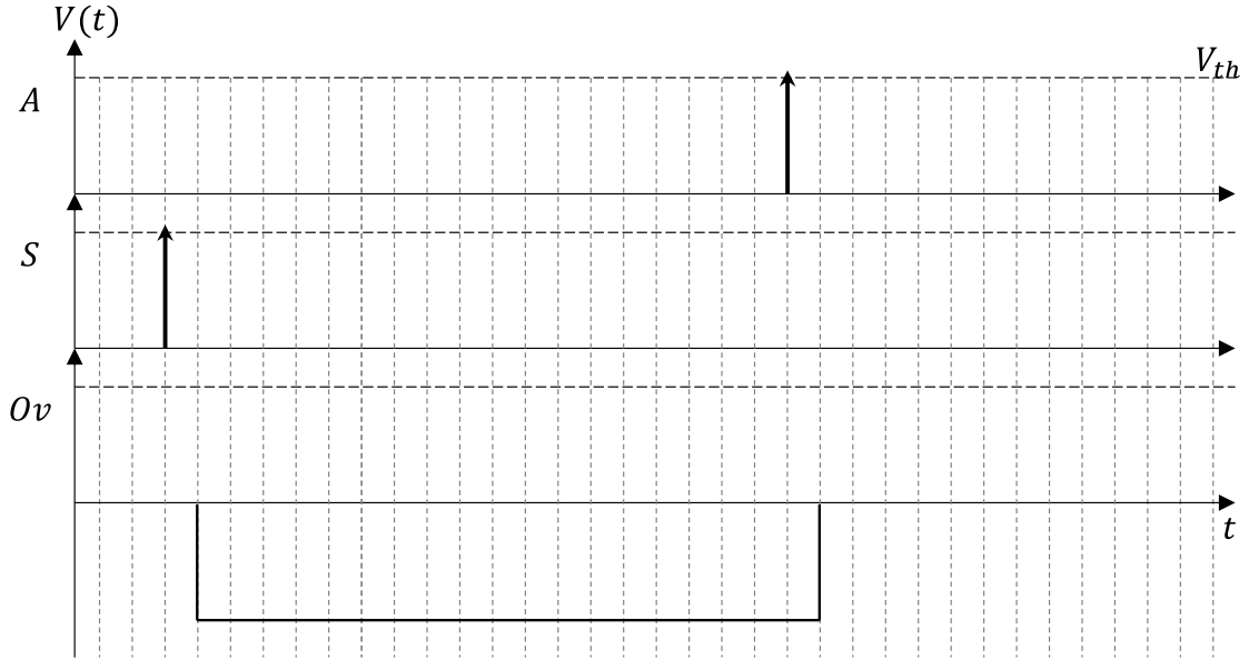
Figure B.5: Overflow chronogram: normal operation mode.
