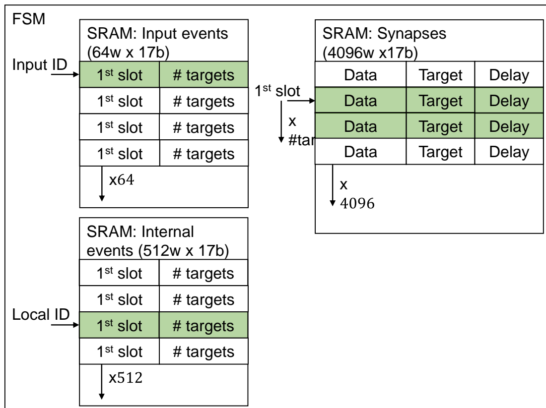
Figure 4.2: FSM handling the 3 SRAMs for ID to synapses conversion. Monitors the Input FIFO and Internal spike FIFO for activity. Retrieves the set of synapses using the corresponding first slot and number of targets to be stimulated.
