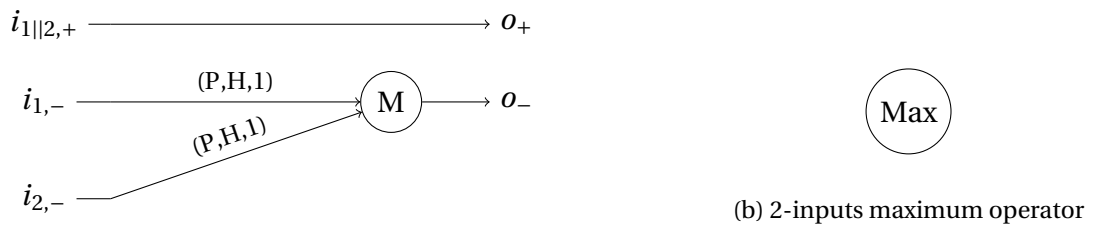
(a) Maximum operator. The M neuron will spike once it receives 2 input spikes.
