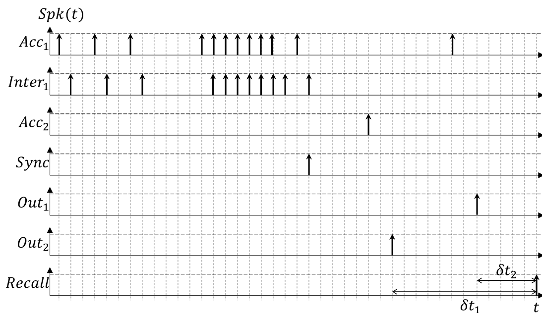
Figure 3.11: Activity for an 8b Linear Combination with 4b inputs.
