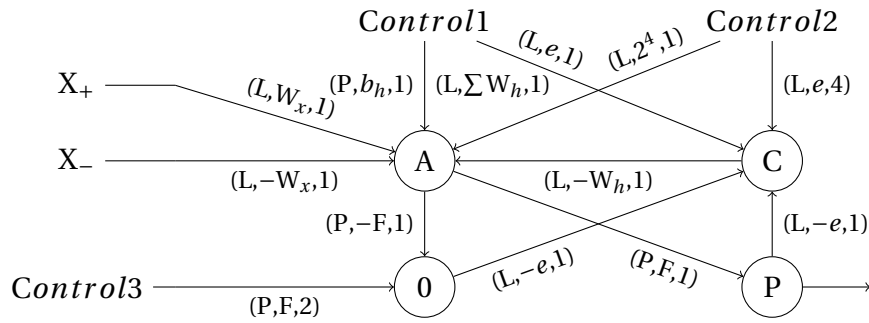
Figure 5.15: Unit used for the spiking RNN topology. The accumulation is performed by the neuron (A), the maximum operation by the neurons (0) and (P) and the copy by the neuron (C). The control channels are responsible for calling the stored values. The value copied in the (C) neuron is sent to every unit from the same layer as input data.
