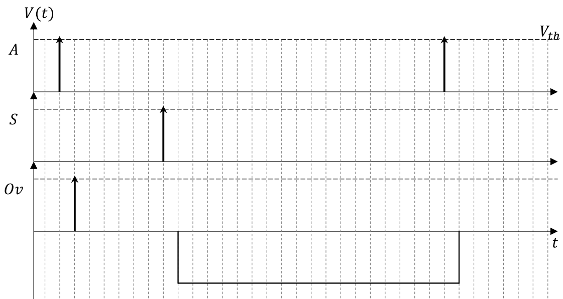
Figure B.4: Overflow chronogram: flagging on overflow.
