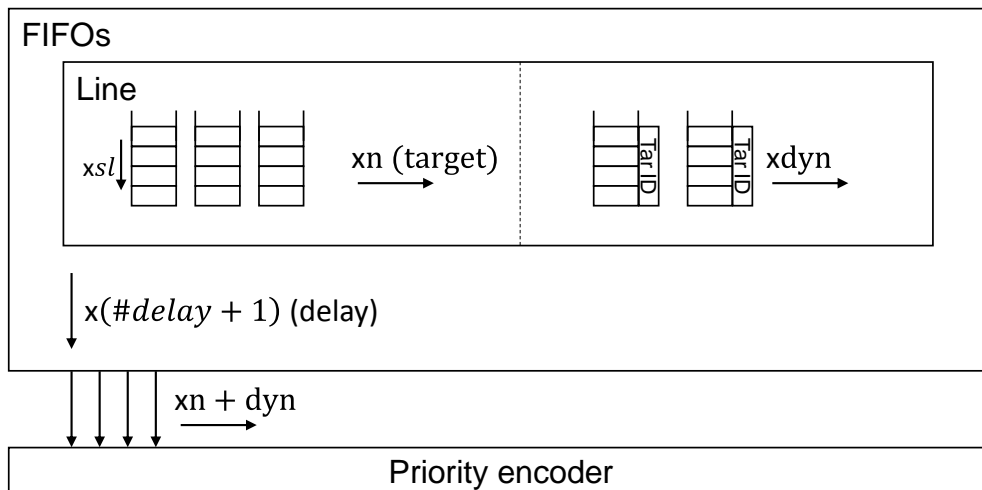
Figure 3.9: Dynamically allocable FIFOs are allocated when the regular FIFO to be written in is full.
