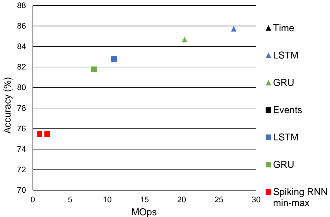
Figure 5.19: Accuracy versus MOps required for real time processing @1x100 recurrent layer size. 32b MAC for GRU and LSTM are counted as 2 operations. Synaptic events are counted as 1 operation for the Spiking RNN.
