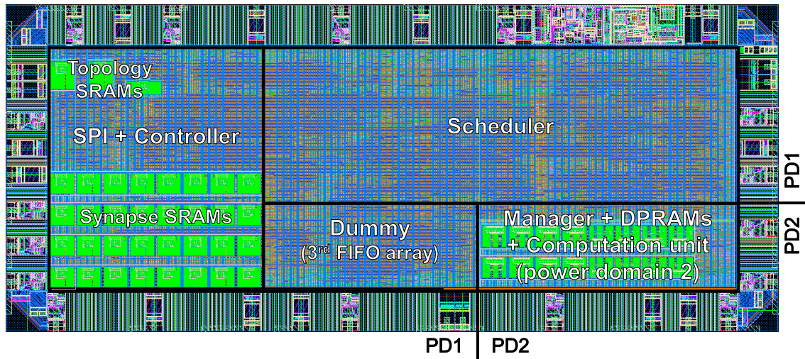
Figure 4.5: Layout of the POC INSPIRE.
