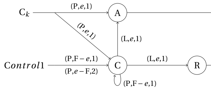
Figure 5.13: Counting input events and sending the result to the recurrent layers when recalled by the Control1 channel.
