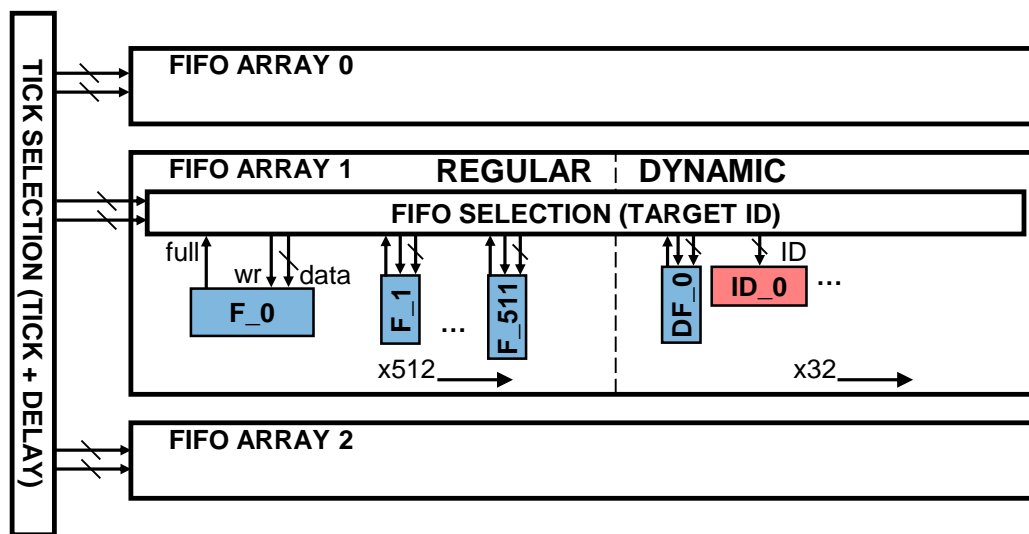
Figure 4.3: Synchronous storing of synaptic stimuli using the synaptic delay to determine in which array and the target ID to determine in which FIFO. F and DF are respectively the regular FIFOs and Dynamically allocable FIFOs (associated with a target ID register).
