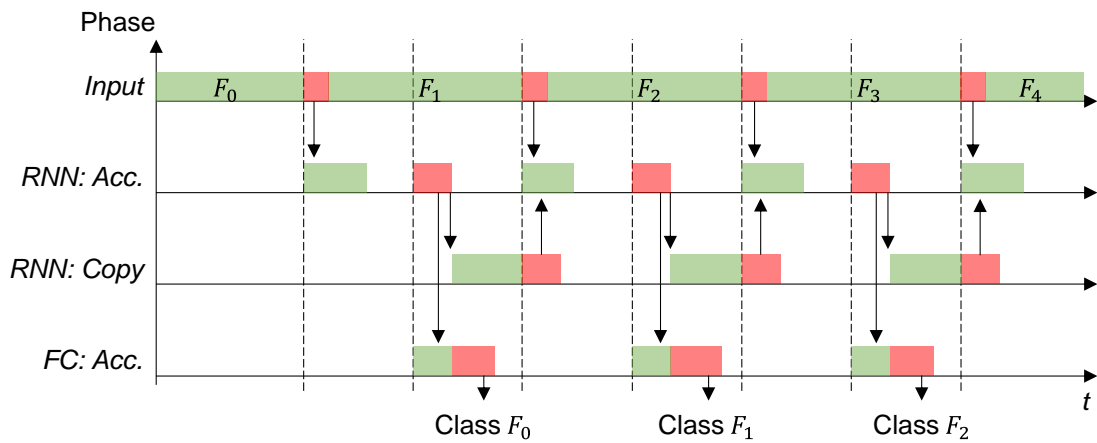
Figure 5.16: Scheduling RNN update. The topology used for this example is 1 RNN layer followed by the FC layer. The green phases represents accumulating the inputs and the red phases represent recalling the stored values. Scheduling the different phases is done using the Control channels.
