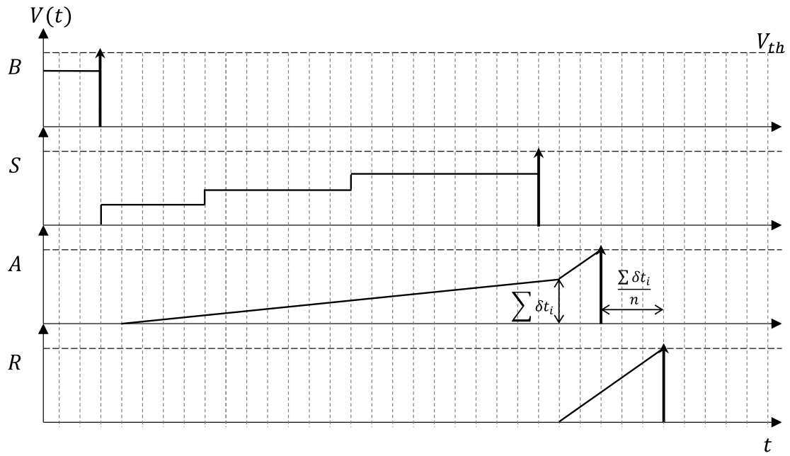
Figure B.2: Chronogram for averaging 4 intervals.
