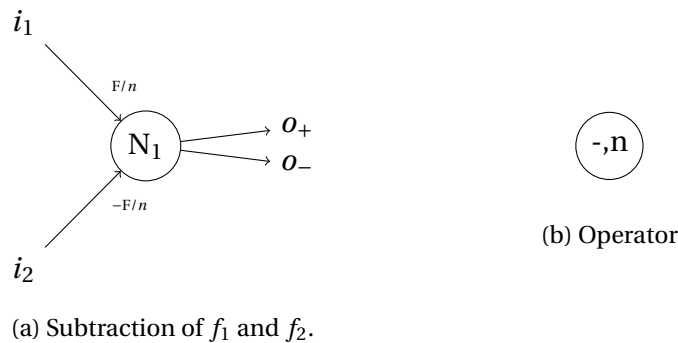
Figure 2.8: Subtraction implementation with parameter n .
