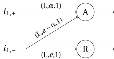
(a) Multiplication per \alpha using linear synapse and 2 neurons.
