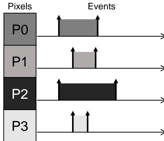
Figure 1.2: Static luminance measured by a DVS using active pixel and sent as a couple of events. The inter-event time interval defines the luminance value.
