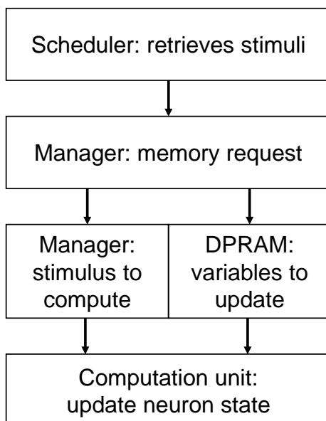
Figure 3.13: Stimulus processing pipeline, from the scheduler to the computation unit.
