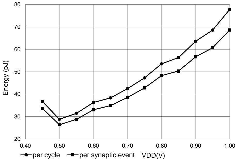
Figure 4.10: Energy per cycle and per synaptic events versus VDD @-0.3VBB.
