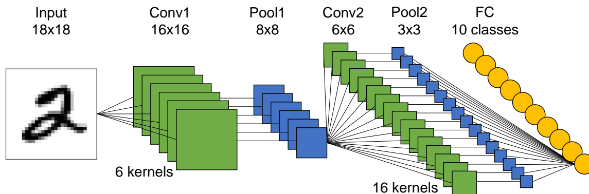
Figure 5.3: 5-layer CNN using 18x18 input images. Conv1 is composed of 6 kernels and conv2 16 kernels. The classifier is Fully Connected layer of 10 neurons.
