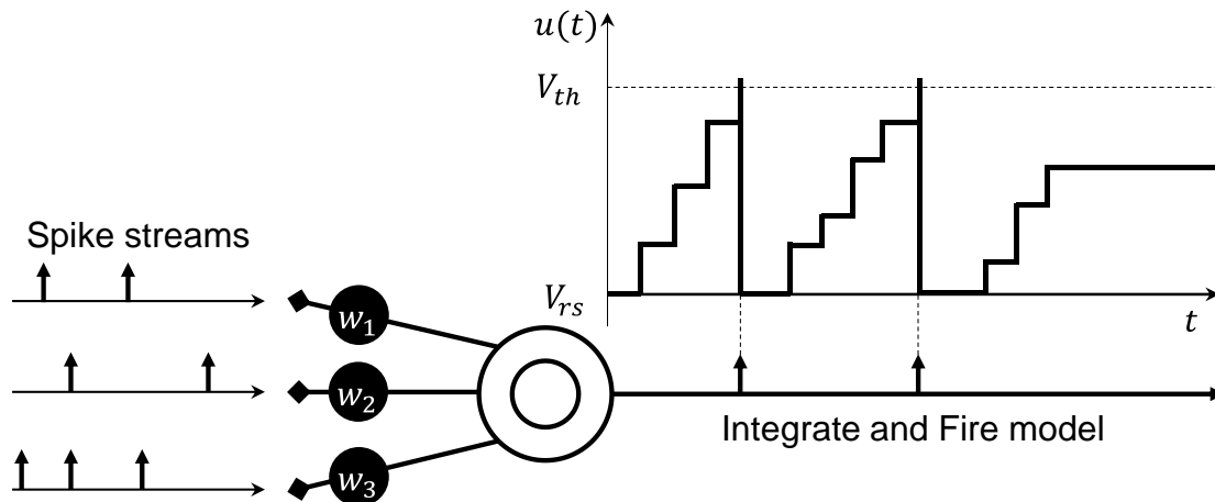
Figure 1.7: Example of spiking neuron model: Integrate and Fire. The synapses used here induce jumps in the membrane potential u(t) . Once u(t) reaches V_{th} , the neuron emits a spike and resets to V_{rs} .
