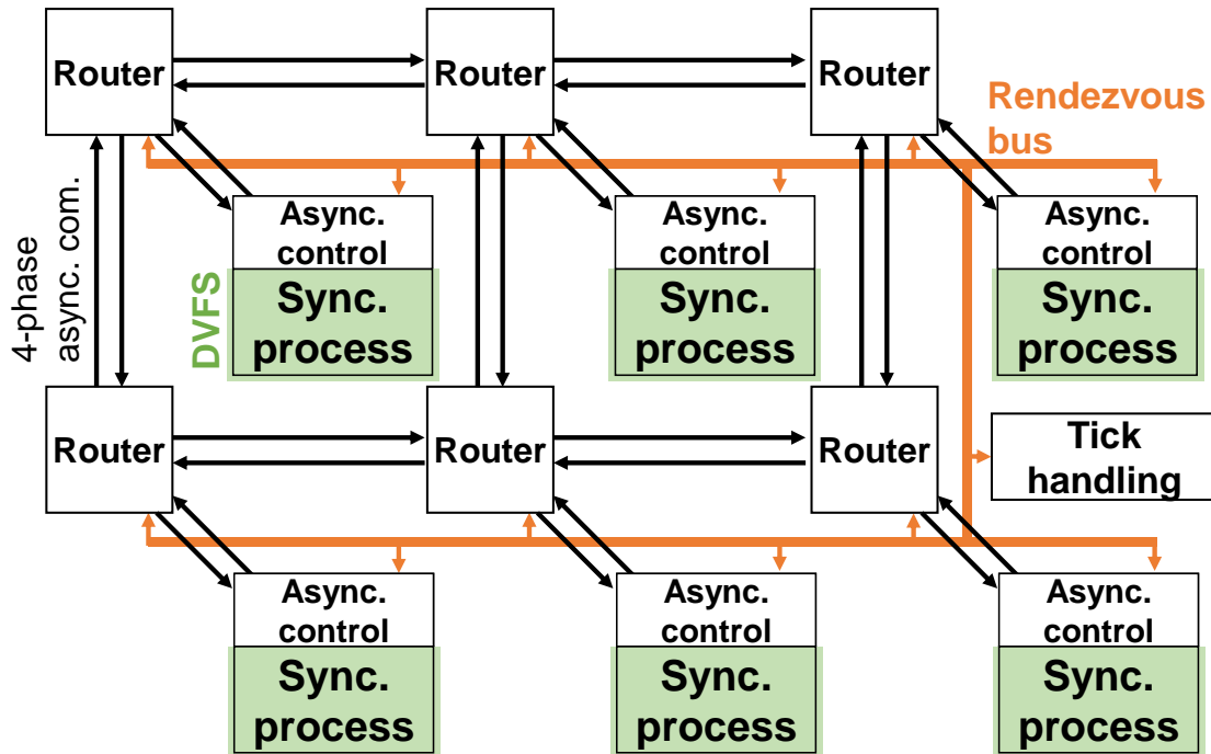
Figure 3.1: GALS architecture.
