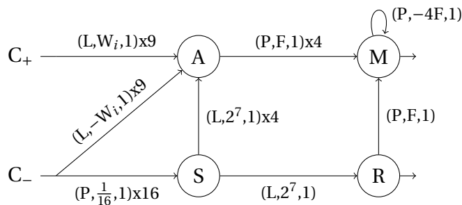
Figure 5.9: Rounding is computed when recalling the values stored in the accumulators and the recall neuron with the updated weight 2^7 .
