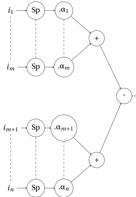
Figure 2.26: Naive Linear Combination implementation using time coded operators.
