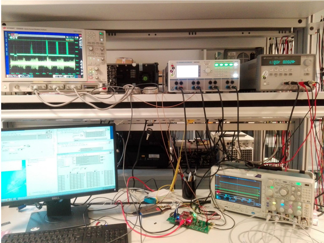
Figure 4.7: Test setup for INSPIRE.
