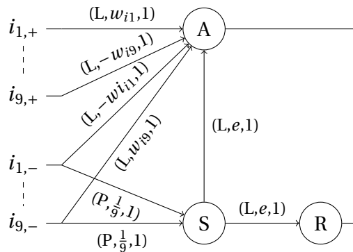
Figure 5.4: Topology used for Kernel computation.
