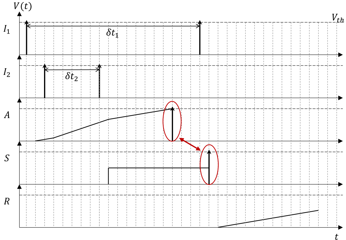
Figure 2.15: Adder chronogram including fixed-point addition overflow denoted by the accumulating neuron spiking before being recalled by the synchronization neuron.
