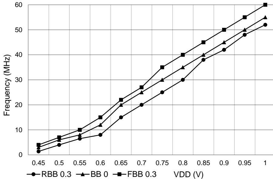
Figure 4.9: Maximum frequency versus VDD @(-0.3;0;0.3) VBB.
