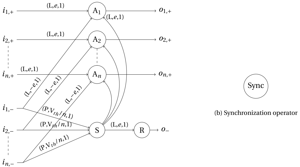
(a) Synchronization operator: store each value in a membrane potential and recall once channel transmitted its data. The output events have a shared second spike coming from o_{-} .
