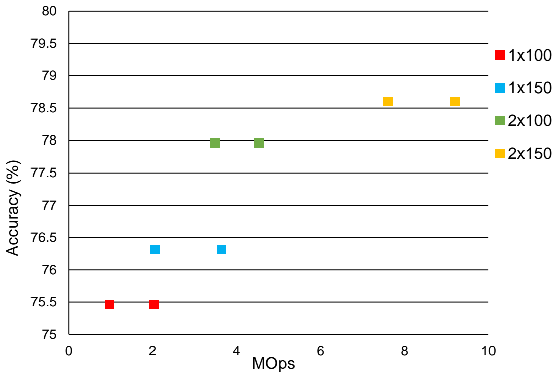
Figure 5.20: Accuracy versus MOps required for real time processing. Comparison of Spiking RNNs of different sizes.
