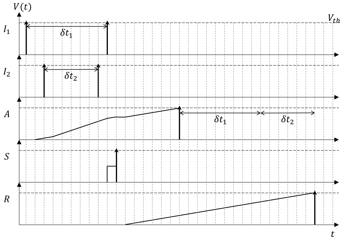
Figure 2.14: Adder chronogram.
