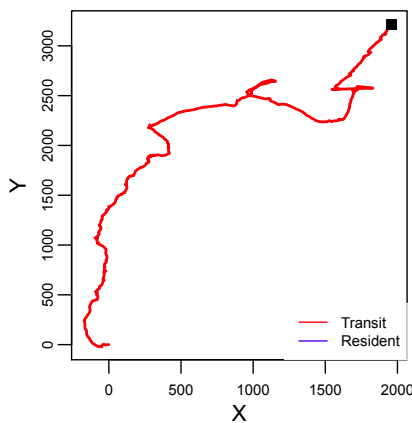
Figure C - 25: Transit and Resident phases. Transit and Resident phases on currents corrected tracks.
