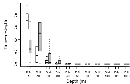
Figure C - 45: Time-at-depth. Time-at-depth histogram for individual X1.
