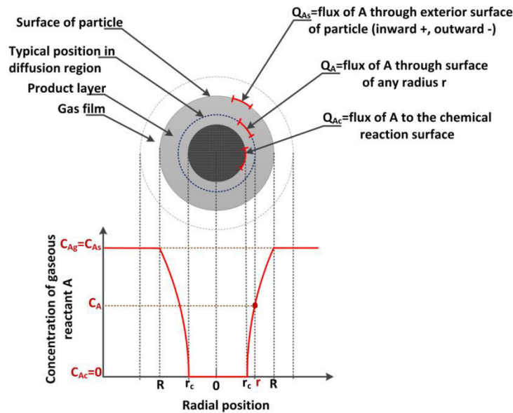
Figure 3. 3 Concentration of HCl gas under the condition that the reaction is only limited by internal diffusion of HCl through the product-layer (A refers to HCl gas)
