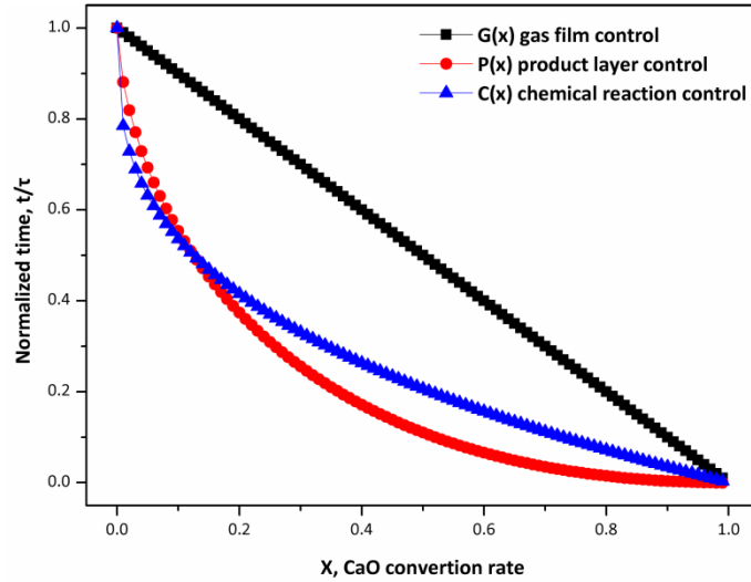
Figure 3.5 Normalized reaction time as a function of CaO reactant conversion rate
