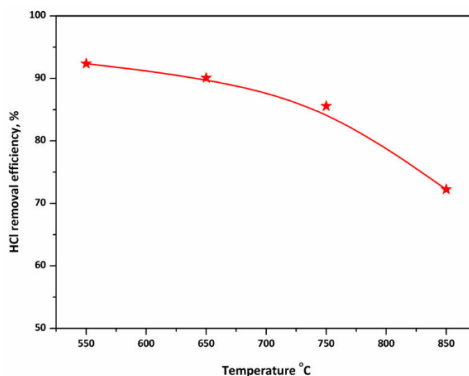
Figure 4. 12 Effect of temperature on HCl mitigation efficiency during PVC pyrolysis with the presence of in-furnace CaO reactant
