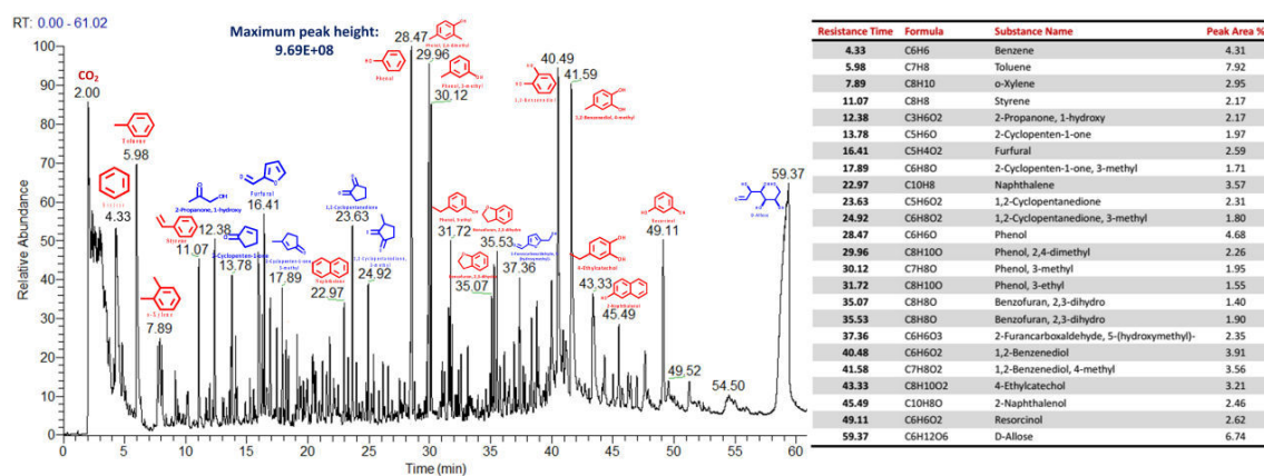
Figure 5. 3 Identified tar composition from wood biomass pyrolysis at 750 °C with the addition of CaO reactant
