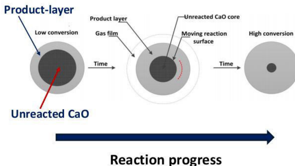
Figure 3. 1 Schematic diagram of the reaction between CaO and HCl, showing the growth of the CaCl 2 product-layer and the consumption of unreacted CaO core
