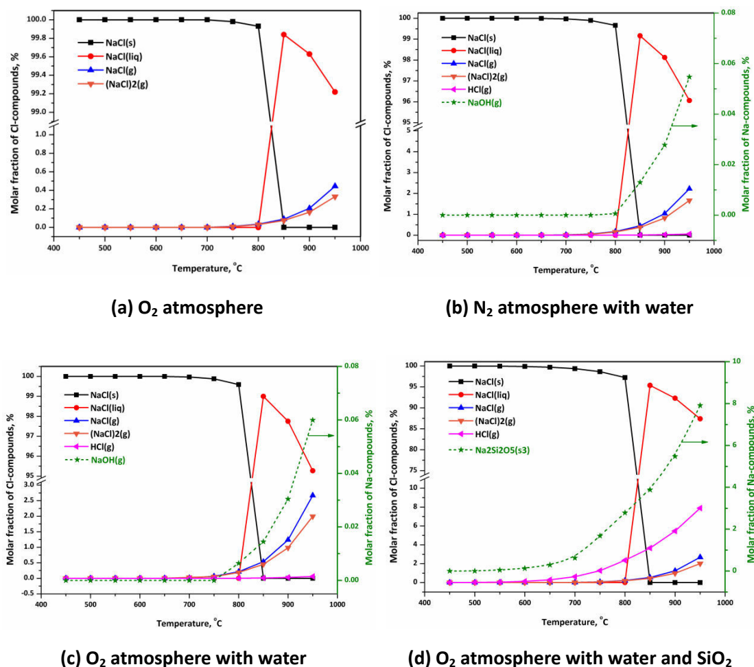
Figure 4. 3 Thermodynamic simulation results of NaCl under considered working conditions: (a) under O 2 atmosphere; (b) under N 2 atmosphere with water; (c) under O 2 atmosphere with water; and (d) with the presence of SiO 2 and water under O 2 atmosphere
