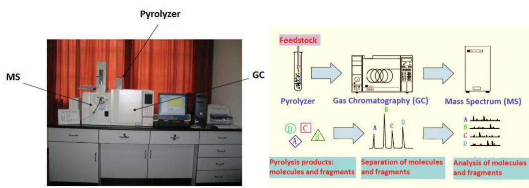
Figure 2. 6 General photograph and schematic diagram of the Py-GC/MS experimental apparatus
