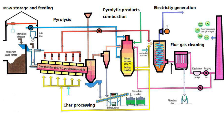
Figure 7. 3 Schematic diagram of the considered pyrolysis system, data obtained from the report of DGEEngineering [29]
