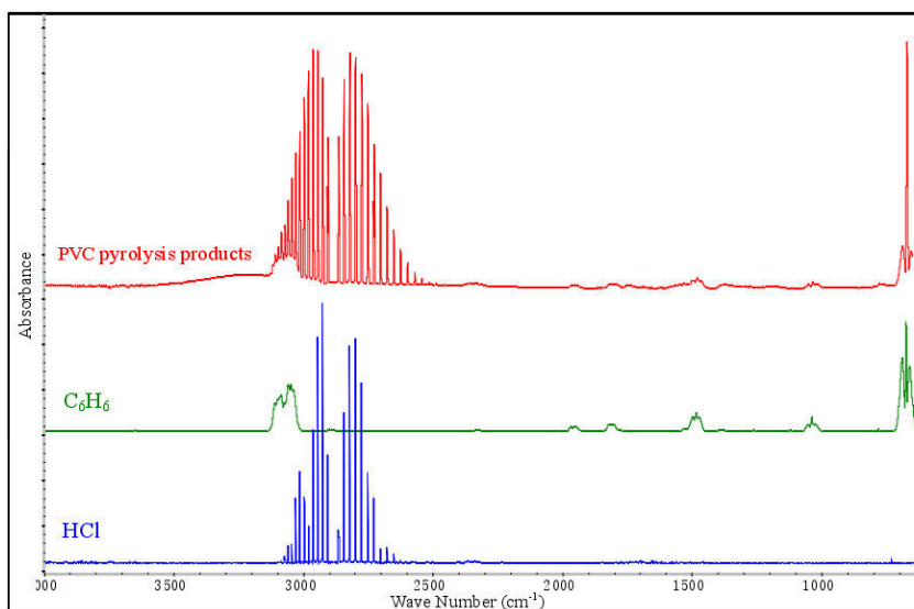
Figure 4. 8 Products identification of the first mass loss peak during PVC pyrolysis using TG-FTIR analysis
