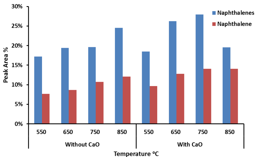
Figure 5. 23 The relative content of naphthalenes and naphthalene in pyrolytic tar derived from PVC pyrolysis without/with CaO reactant
