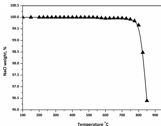
Figure 4. 4 TG analysis results of NaCl under N 2 atmosphere
