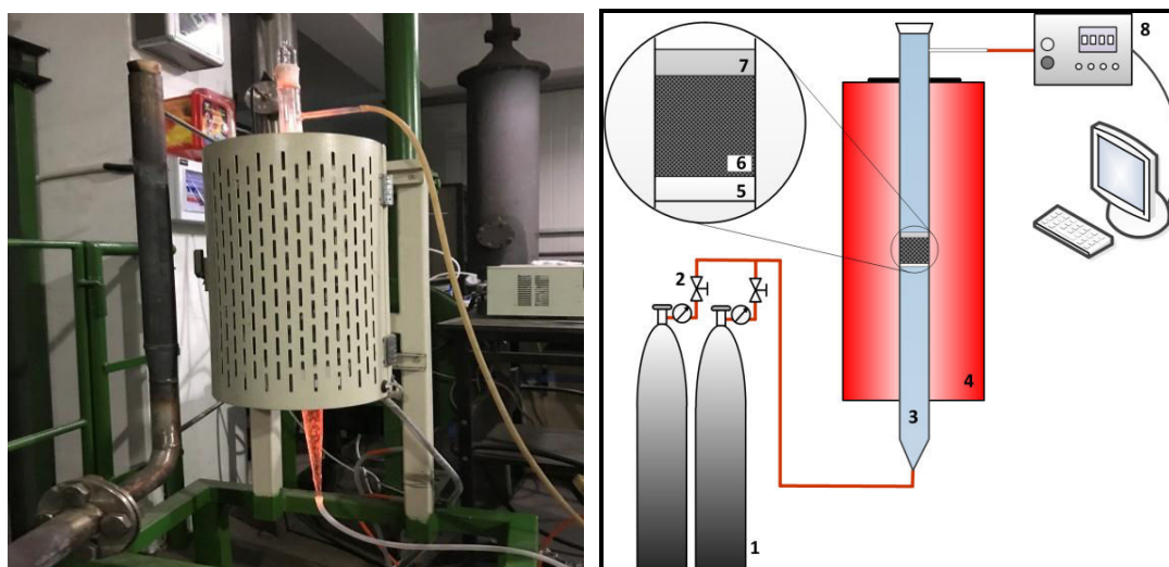
Figure 2. 4 General photograph and schematic diagram of the vertical tubular furnace reactor: 1, gas source; 2, gas flow meter; 3, vertical quartz tubular reactor; 4, electric heater and temperature controller; 5, quartz filter; 6, CaO reactant for HCl mitigation; 7, quartz wool; 8, HCl gas detector
