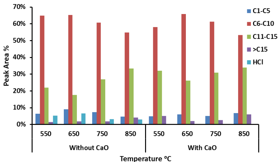
Figure 5. 21 Distributions of detected species of pyrolytic tar derived from PVC pyrolysis as a function of carbon atom numbers
