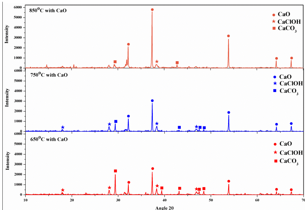
Figure 6. 3 XRD spectrums of the obtained solid residues (from bottom to top): 650 °C with CaO reactant; 750 °C with CaO reactant; and 850 °C with CaO reactant
