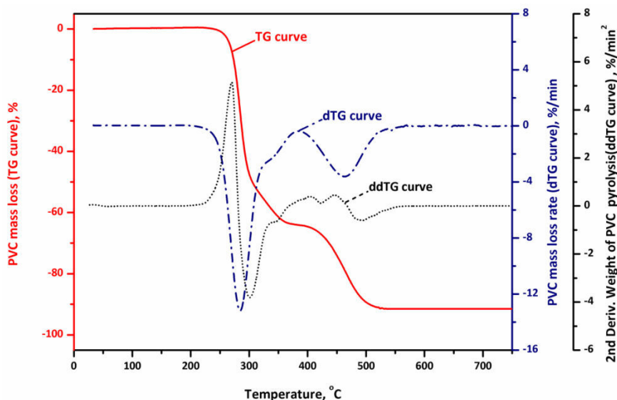
Figure 4. 7 TG, DTG and 2 nd order DTG curves of PVC pyrolysis under N 2 atmosphere at heating rate of 10 °C/min
