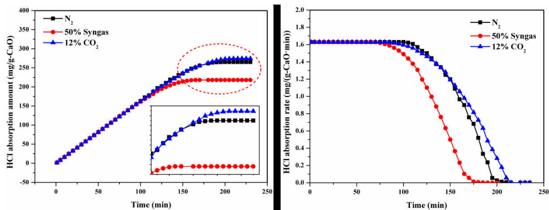
Figure 3. 15 Effect of gas composition on total HCl mitigation amount and HCl mitigation rate by CaO reactant
