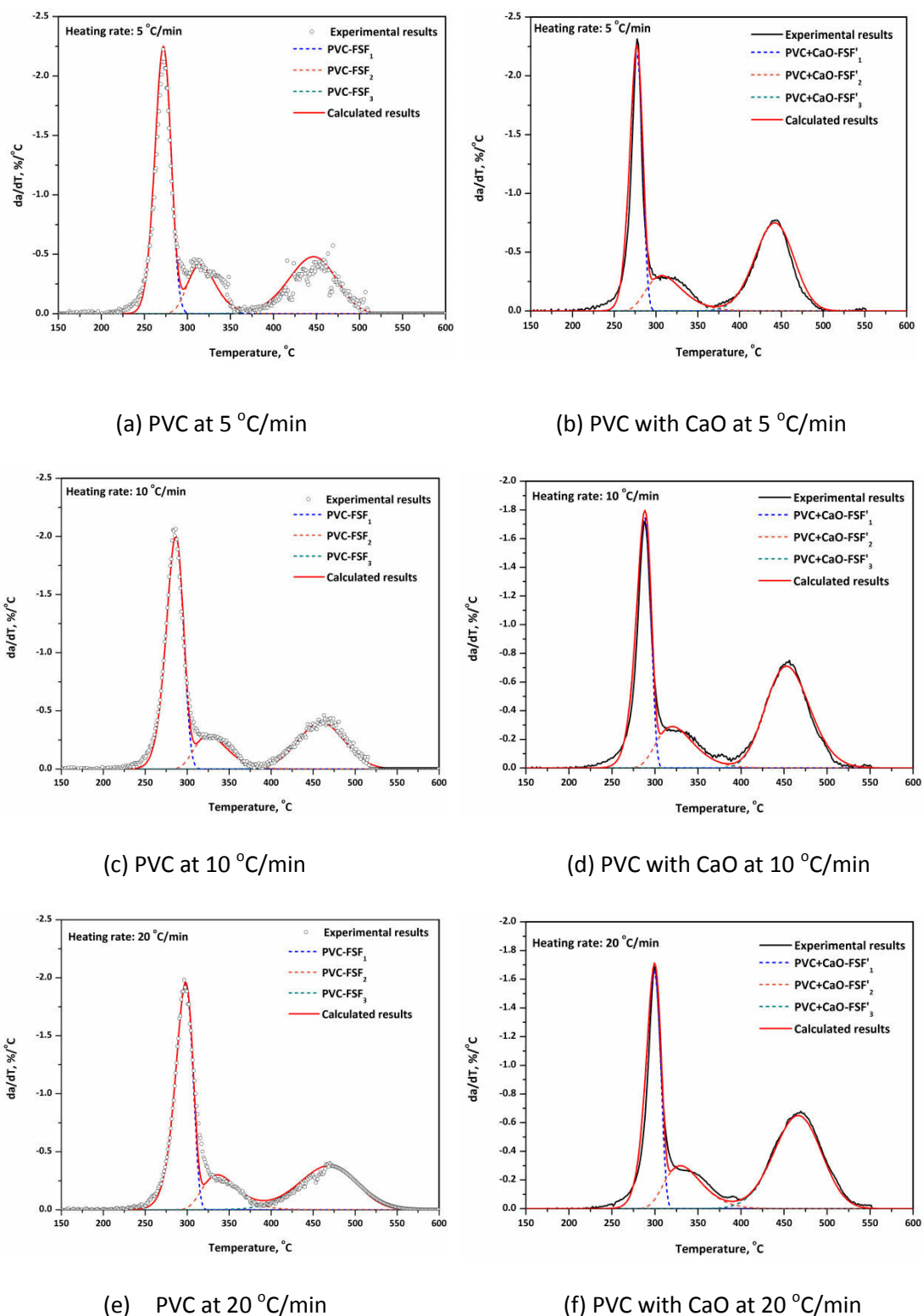
Figure 4. 16 Deconvoluted DTG curves of PVC and PVC with CaO reactant pyrolysis at 5 °C/min, 10 °C /min, and 20 °C /min
