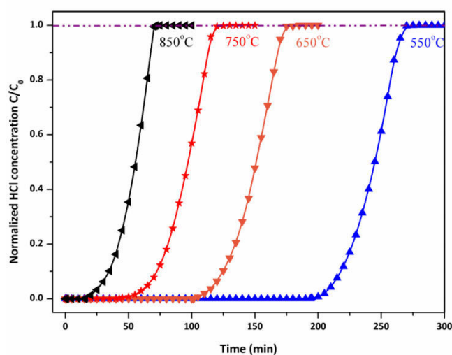
Figure 3. 6 The HCl breakthrough curves of CaO reactants under different temperature
