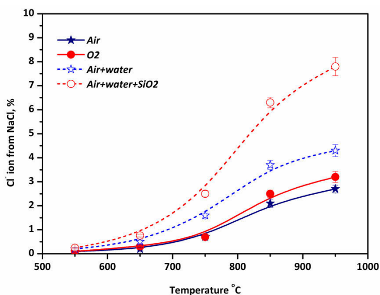
Figure 4. 6 Conversion of Cl - ion from NaCl under air atmosphere and O 2 atmosphere and the effect of water and SiO 2
