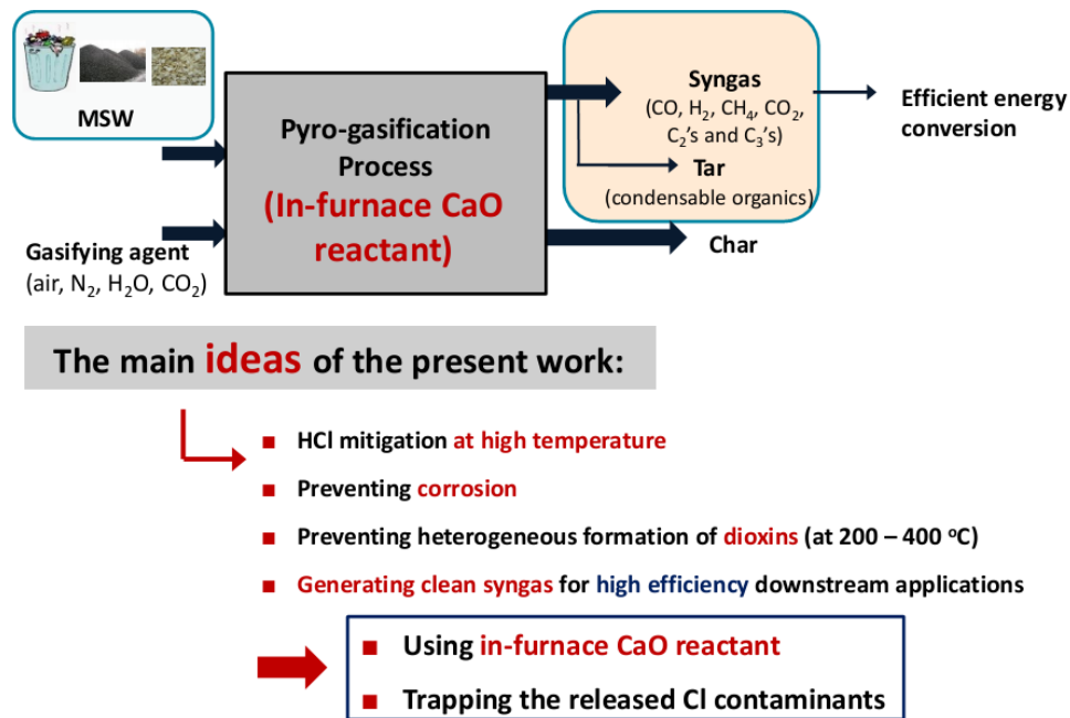
Figure 1. 5 The main ideas of this study: investigate in-furnace capture of chlorine to avoid the release of HCl by using in-situ CaO reactant
