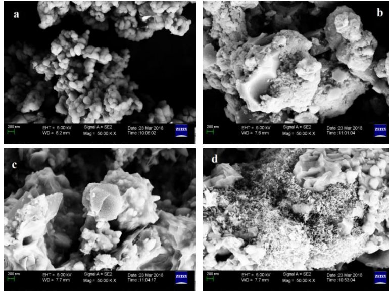
Figure 6. 5 SEM images of fresh (a) and spent CaO reactants (b, pyrolysis residues at 650 °C; c, pyrolysis residues at 750 °C; and d, pyrolysis residues at 850 °C)
