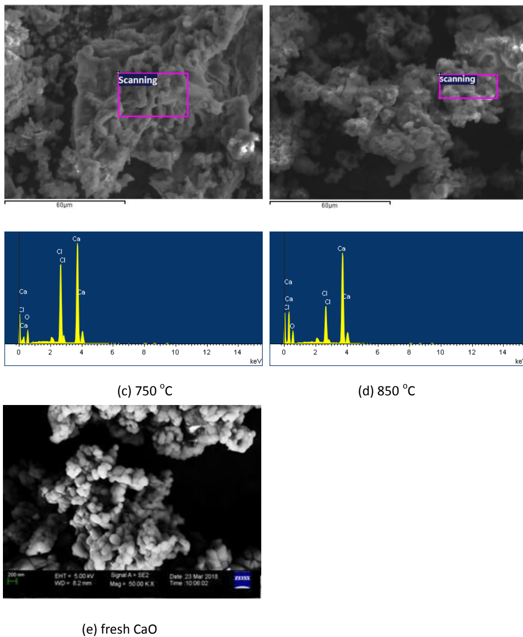
Figure 4. 13 SEM and EDS analysis of the spent CaO reactants at Ca/Cl molar ratio of 2:1: (1) 550 °C; (2) 650 °C; (3) 750 °C; (4) 850 °C; (e) SEM photograph of fresh CaO reactant
