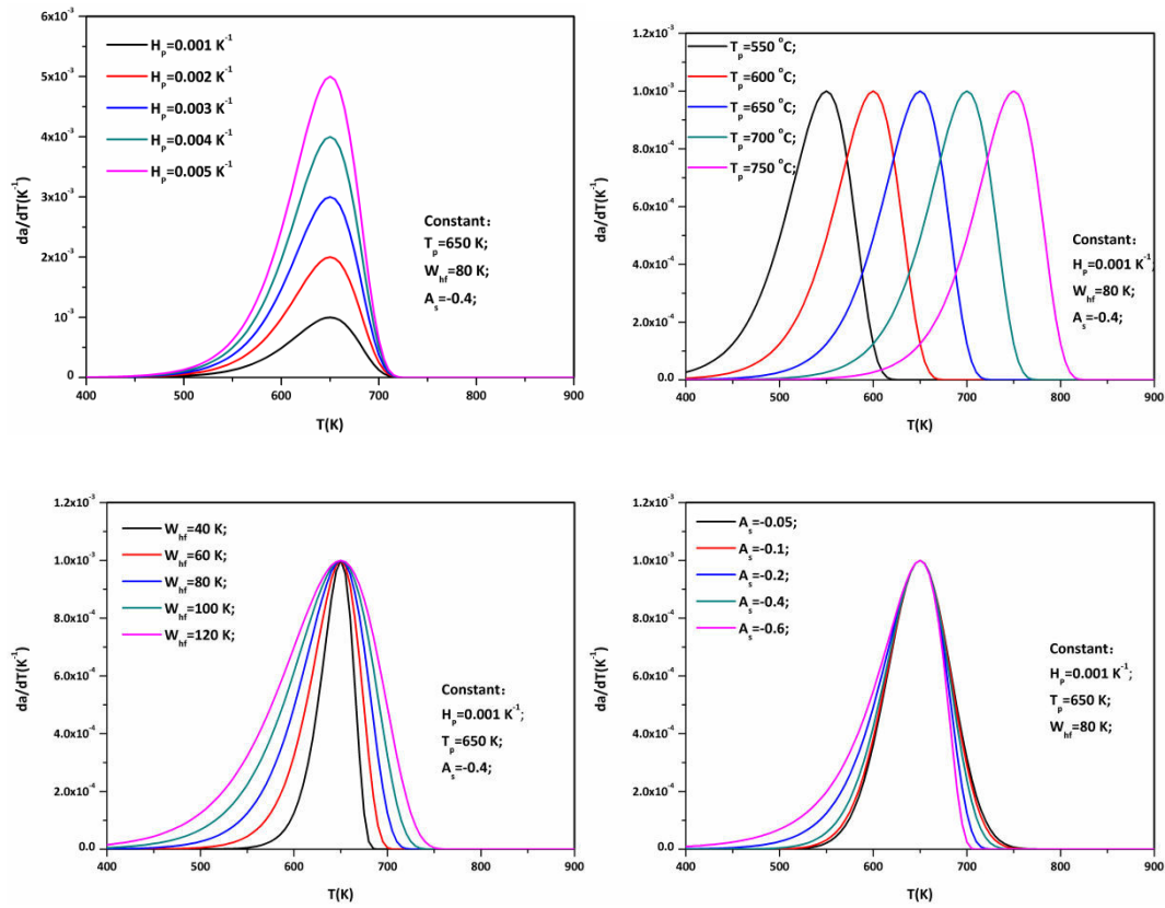
Figure 4. 15 Effect of the parameters in the Fraser-Suzuki function: 1 , the height, H_p ; 2 , the Peak temperature, T_p ; 3 , the half width, w_{hf} ; and 4 , the symmetry, A_s
