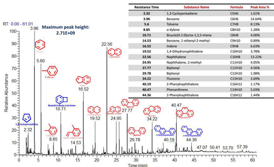
Figure 5. 10 Identified tar composition from PVC pyrolysis at 750 °C with the addition of CaO reactant
