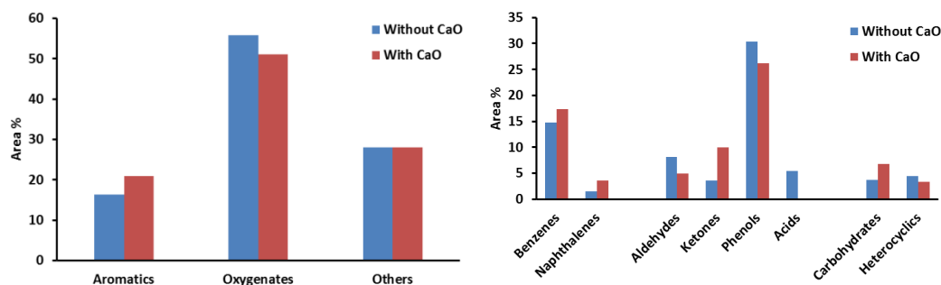
Figure 5. 4 Composition of pyrolytic tar derived from wood biomass pyrolysis at 750 °C without/with the addition of CaO reactant (others here represent the detected compounds which are not presented in Figure 5.1 and Figure 5.2)
