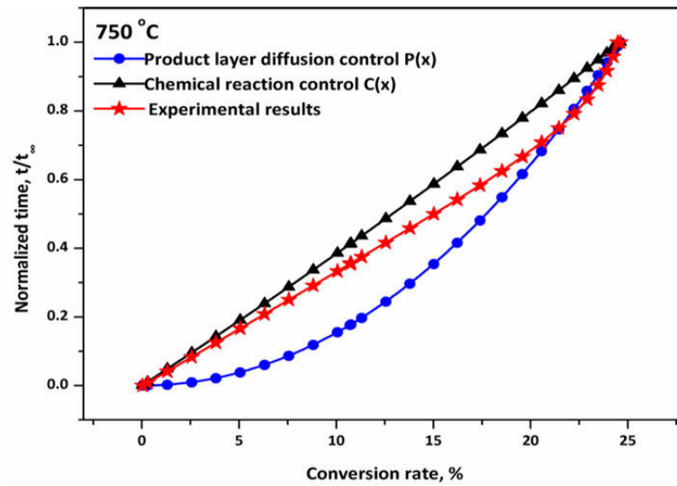
Figure 3. 9 Experimental and calculated P(x) , C(x) vs CaO conversion rate curves at 750 °C
