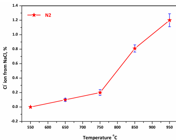
Figure 4.5 Conversion of Cl - ion from NaCl under N 2 atmosphere
