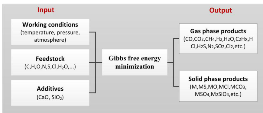
Figure 2. 7 General principle of the thermodynamic equilibrium calculation system
