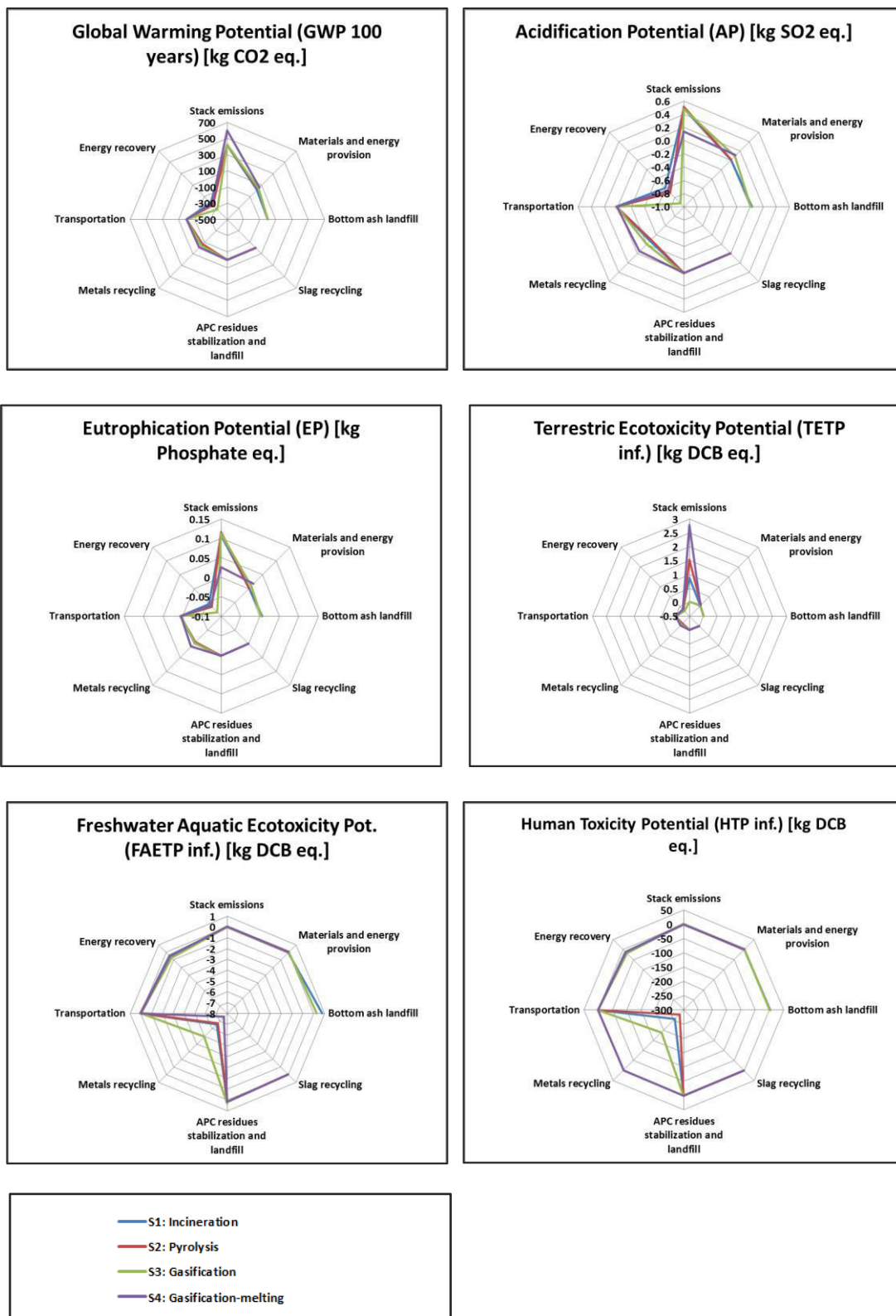
Figure 7. 7 Contribution analysis of the selected environmental impact categories
