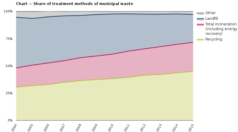
Figure 1. 3 Share of MSW treatment methods in the EU during 2004-2015, data source from Eurostat database [7]
