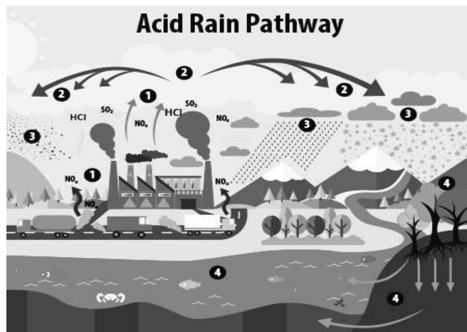
Figure 1. 6 Graphic principle of acid rain formation pathway: (1) Emissions of SO 2 , NO x and HCl are released into the air, where (2) the pollutants are transformed into acid particles that may be transported in a long distance, (3) the acid particles then fell to the earth as wet and dry deposition (dust, rain, snow, or etc.) and (4) may cause harmful effects on soil, forests and water, data obtained from [42]
