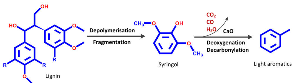
Figure 5. 6 Representative lignin pyrolysis, decarboxylation and decarbonylation of pyrolytic tar over CaO reactant
