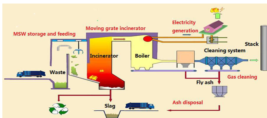
Figure 7. 2 Schematic diagram of the considered incineration system
