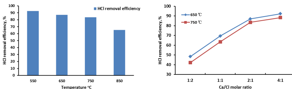
Figure 6. 4 Effect of temperature and Ca/Cl molar ratio on HCl mitigation efficiency during S-MSW pyrolysis
