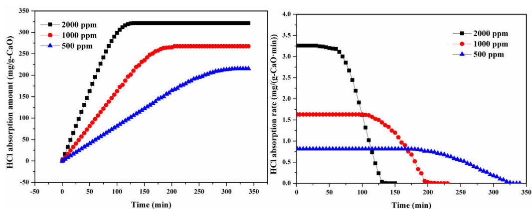
Figure 3.14 Effect of raw HCl concentration on total HCl mitigation amount and HCl mitigation rate by CaO reactant
