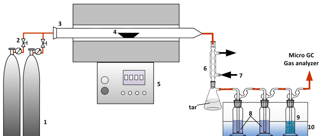
Figure 2. 5 Schematic diagram of the experimental fixed bed tubular furnace apparatus. 1, gas source; 2, gas flowmeter; 3, quartz tubular furnace; 4, quartz boat; 5, electric heater and temperature controller; 6, condenser for tar collection; 7, cooling water; 8, HCl mitigation solution (0.1 mol/L NaOH); 9, silica gel; 10, ice-water bath
