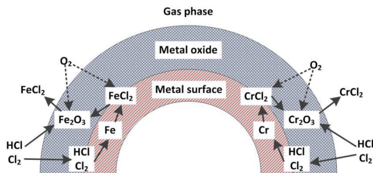
Figure 1. 7 Schematic diagram of high temperature corrosion occurred on the surface of the equipment, data obtained from Wang [49]
