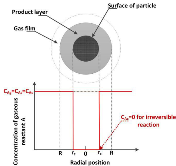
Figure 3.4 Concentration of HCl gas under the condition that the reaction is only limited by gas-solid chemical reaction (A refers to HCl gas)
