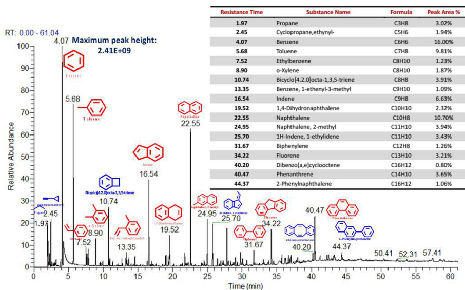
Figure 5. 9 Identified tar composition from PVC pyrolysis at 750 °C in the absence of CaO reactant
