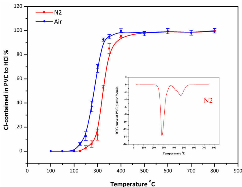
Figure 4. 9 HCl release from PVC pyrolysis and incineration in fixed bed tubular furnace reactor
