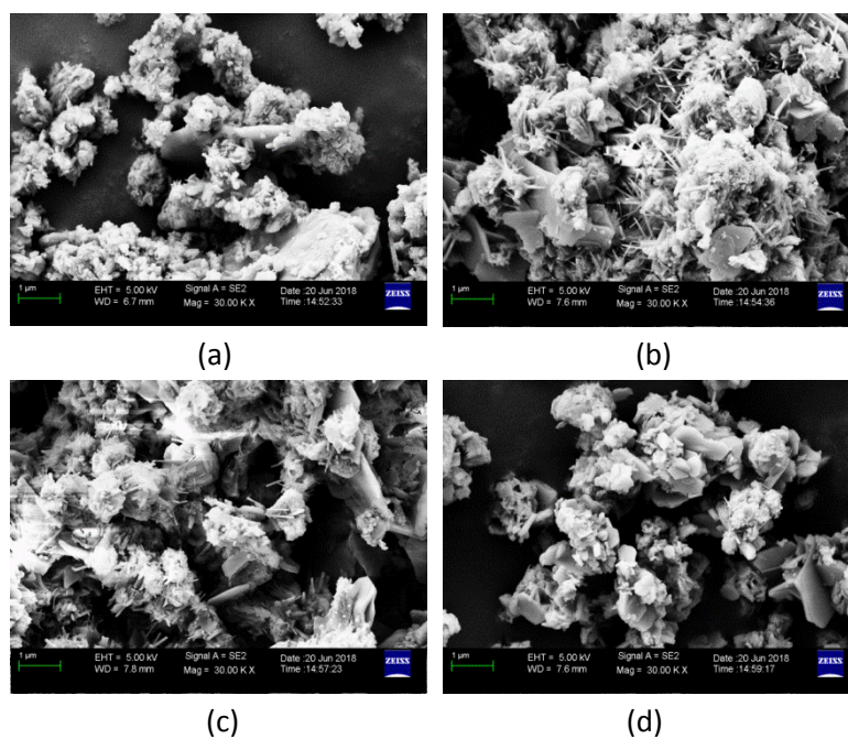
Figure 3. 12 Formation of the product-layer at temperature of 850 °C: a, t/t_f = 0.1 ; b, t/t_f = 0.3 ; c, t/t_f = 0.5 ; d, t/t_f = 1
