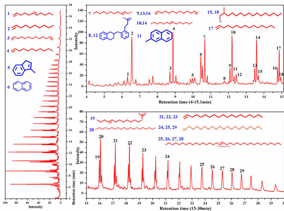
Figure 6. 8 Tar produced form S-MSW pyrolysis with CaO reactant at 550 °C
