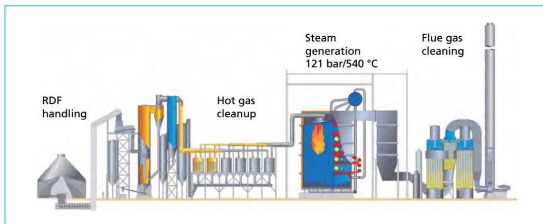
Figure 1. 4 Conceptual diagram of Kymijärvi II RDF gasification power plant, located in Lahti region, Finland, data acquired from [13]
