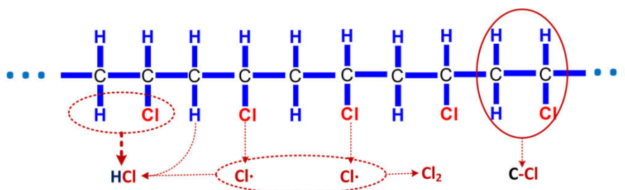
Figure 5. 11 Chlorine-content compounds formation from PVC pyrolysis, data derived from Ruizhi ZHANG [22]
