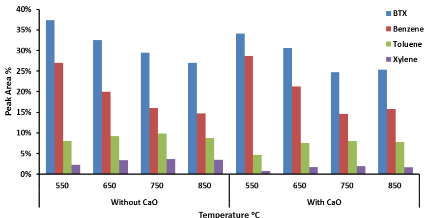
Figure 5. 22 The relative content of BTX in pyrolytic tar derived from PVC pyrolysis without/with CaO reactant
