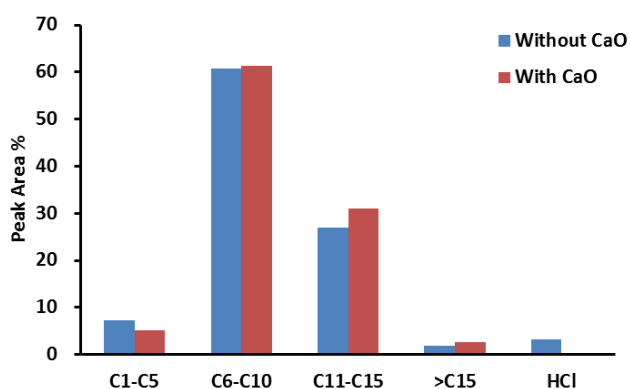
Figure 5. 12 Distributions of detected species of pyrolytic tar derived from PVC pyrolysis at 750 °C as a function of carbon atom numbers
