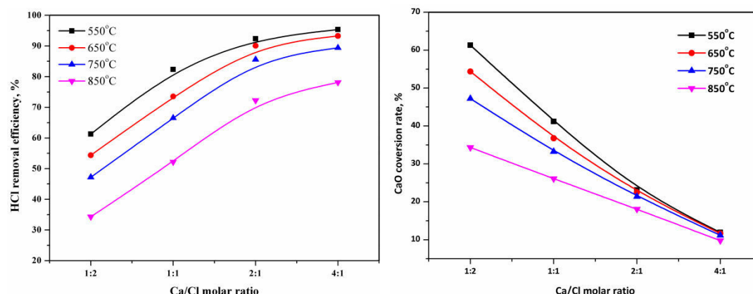
Figure 4. 10 Effect of Ca/Cl molar ratio on HCl mitigation efficiency and CaO conversion rate during PVC pyrolysis with the presence of in-furnace CaO
