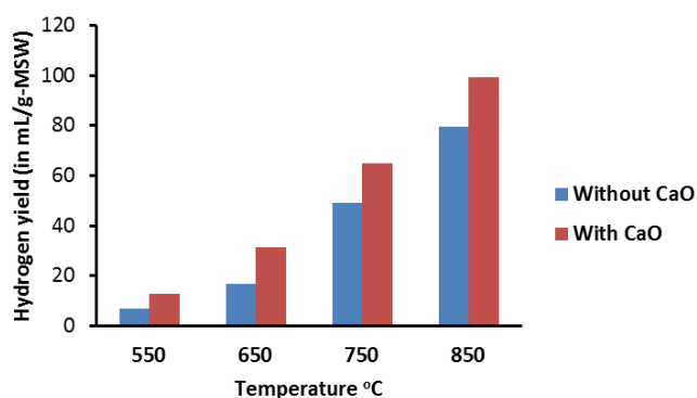
Figure 6. 2 Effect of temperature and CaO reactant on hydrogen yield (in mL/g-MSW)
