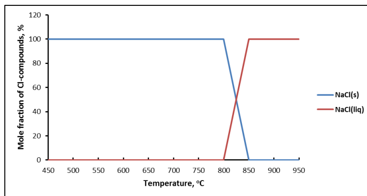
Figure 4. 2 Thermodynamic simulation results of pure NaCl under N 2 atmosphere
