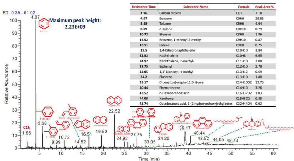
Figure 5. 15 Identified tar composition from PVC pyrolysis at 550 °C with the addition of CaO reactant
