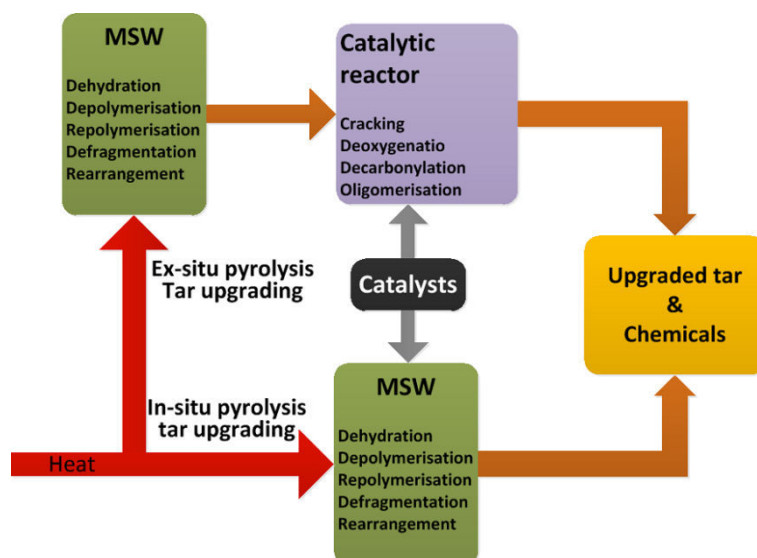
Figure 5. 1 Schematic diagram of in-situ and ex-situ of tar cracking during MSW pyrolysis, data source from Kabir et al. [7]
