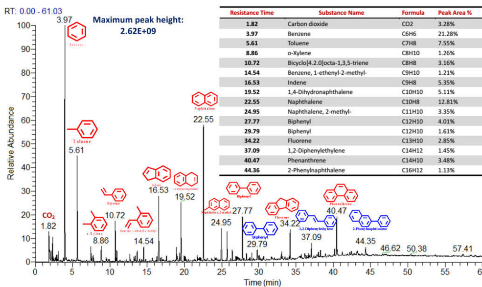
Figure 5. 17 Identified tar composition from PVC pyrolysis at 650 °C with the addition of CaO reactant
