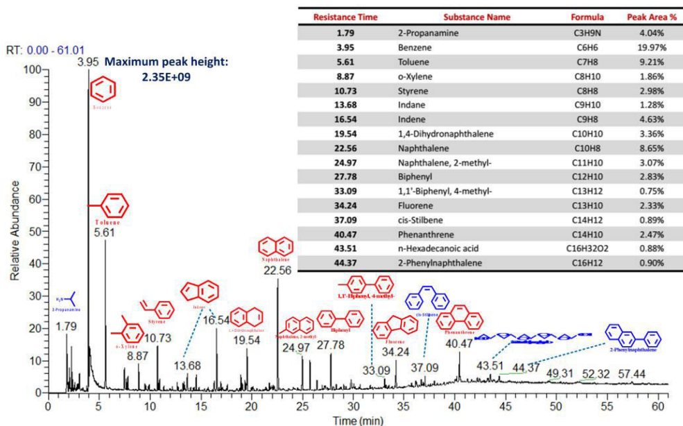
Figure 5. 16 Identified tar composition from PVC pyrolysis at 650 °C in the absence of CaO reactant
