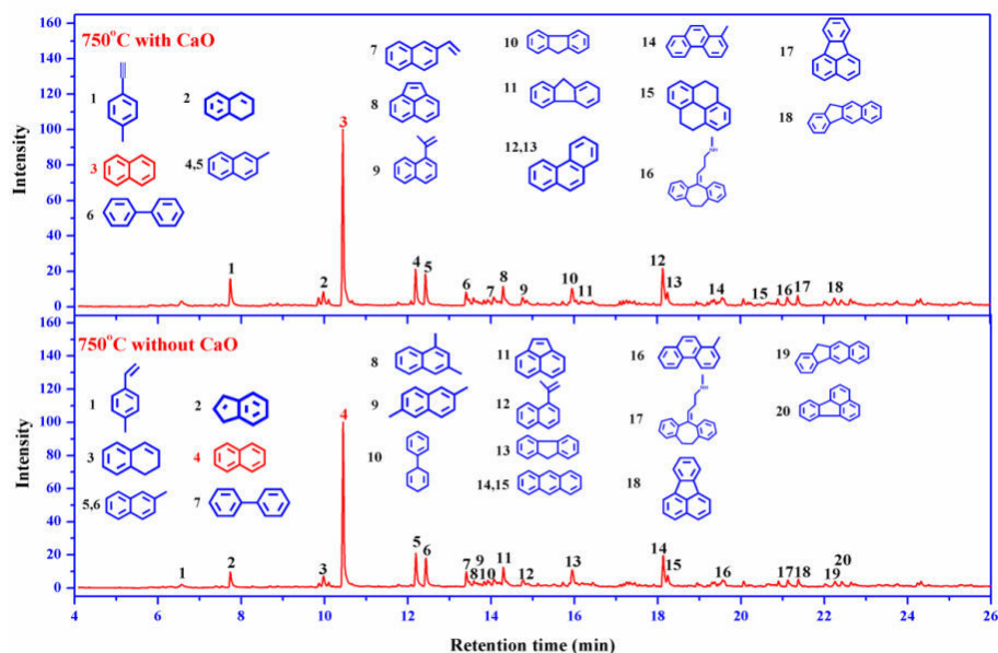
Figure 6. 9 Tar produced form S-MSW pyrolysis without/with CaO reactant at 750 °C
