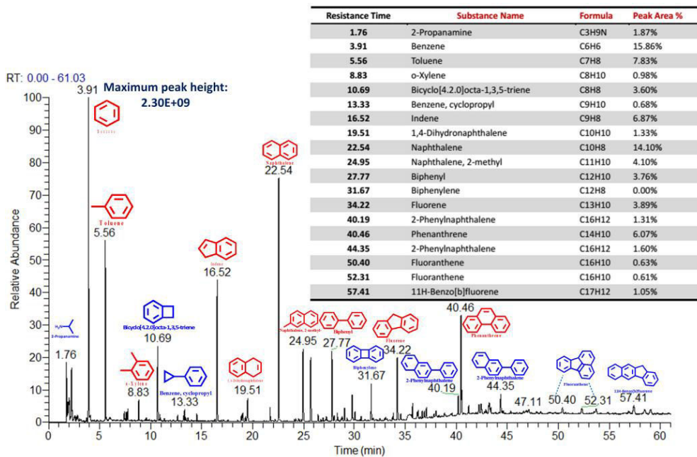
Figure 5. 19 Identified tar composition from PVC pyrolysis at 850 °C with the addition of CaO reactant
