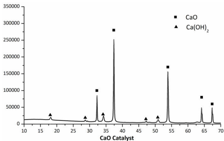
Figure 2. 2 XRD analysis of CaO reactant
