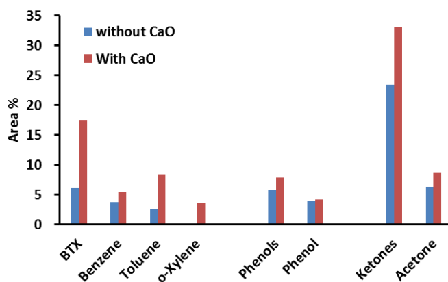
Figure 5. 8 The relative content of BTX, phenols, and ketones in pyrolytic tar derived from food waste pyrolysis at 750 °C without/with CaO reactant
