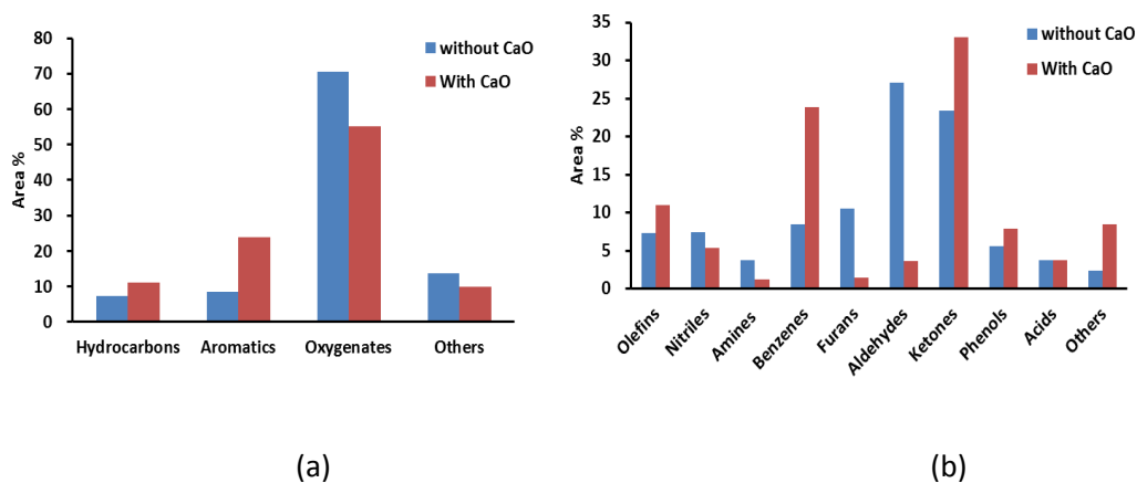
Figure 5. 7 Composition of pyrolytic tar derived from food waste pyrolysis at 750 °C without/with the addition of CaO reactant (others represent mainly nitrogen-content compounds)
