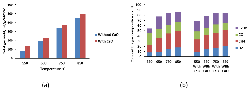
Figure 6. 1 Effect of temperature and CaO reactant on produced gas characteristics: a, total gas yield; and b, combustible gas composition (the carrier gas N 2 is subtracted from the produced gas)
