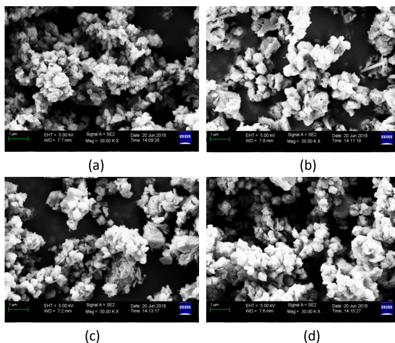
Figure 3. 11 Formation of the product-layer at temperature of 750 °C: a, t/t_f = 0.1 ; b, t/t_f = 0.3 ; c, t/t_f = 0.5 ; d, t/t_f = 1
