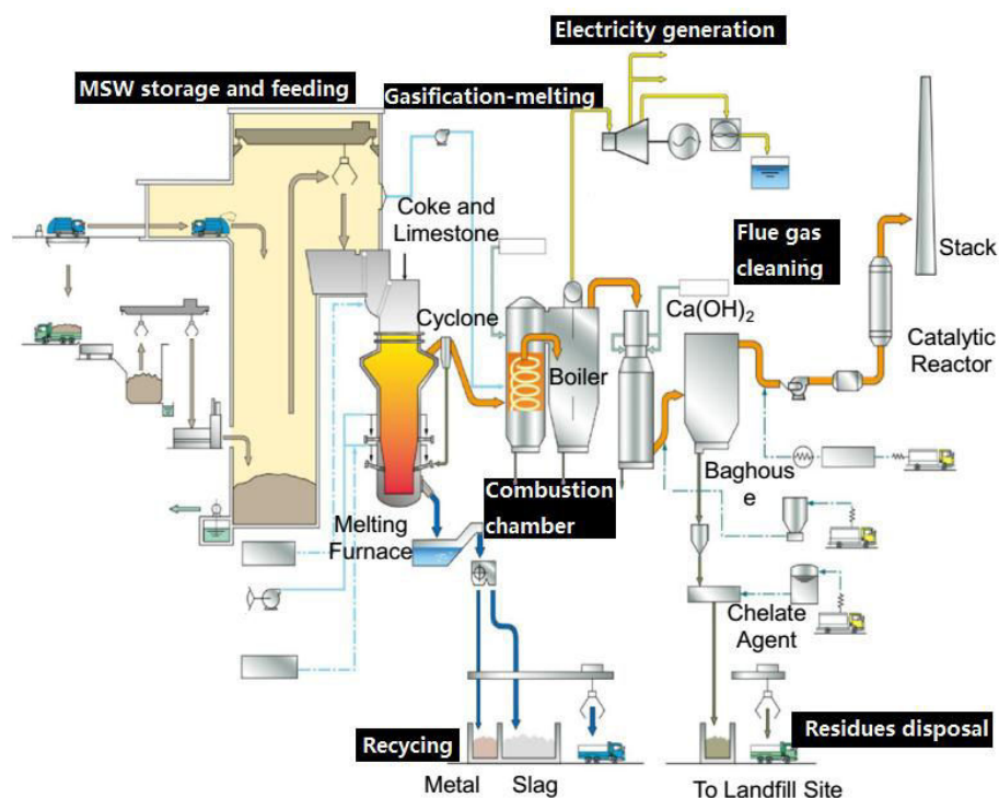
Figure 7. 5 Schematic diagram of the considered gasification-melting system, data obtained from the work of Tanigaki et al. [33]
