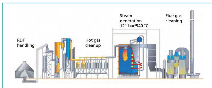
Figure 7. 4 Schematic diagram of the considered gasification system, data obtained from the work of Bolhàr-Nordenkampf et al. [30]
