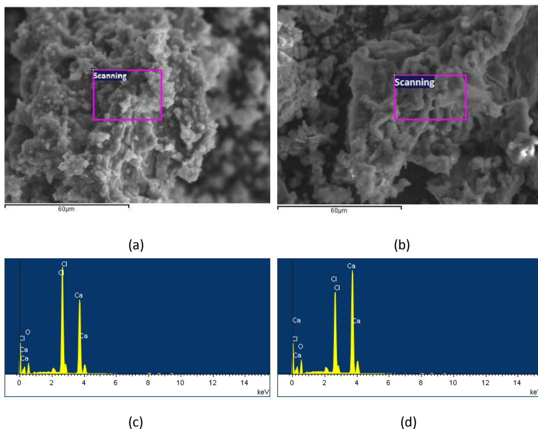
Figure 4. 11 SEM and EDS detection of the spent CaO reactants: (1) SEM, Ca/Cl molar ratio: 1:1, 750 °C; (2) SEM, Ca/Cl molar ratio: 2:1, 750 °C; (3) EDS, Ca/Cl molar ratio: 1:1, 750 °C; (4) EDS, Ca/Cl molar ratio: 2:1, 750 °C
