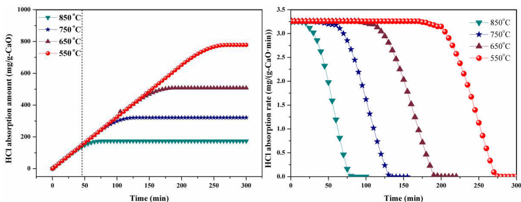
Figure 3. 7 The total HCl mitigation amount and mitigation rate with time under different reaction temperature
