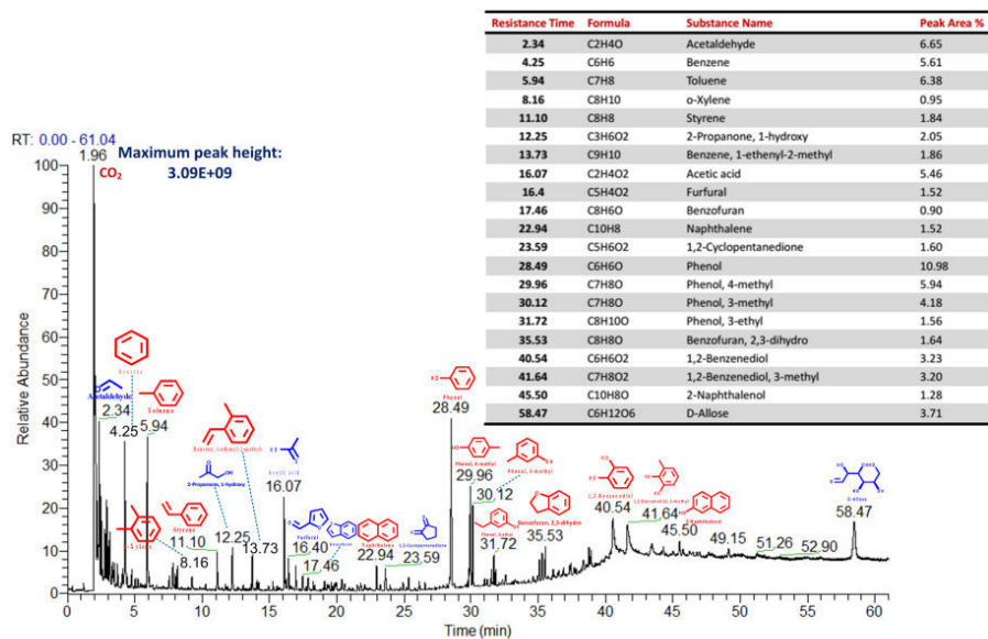
Figure 5. 2 Identified tar composition from wood biomass pyrolysis at 750 °C in the absence of CaO reactant
