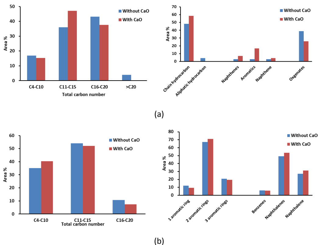
Figure 6. 10 Distributions of products in pyrolytic tar with and without the addition of CaO reactant: (a) pyrolysis at 550 °C and (b) pyrolysis at 750 °C
