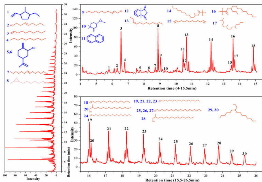
Figure 6. 7 Tar produced form S-MSW pyrolysis without CaO reactant at 550 °C
