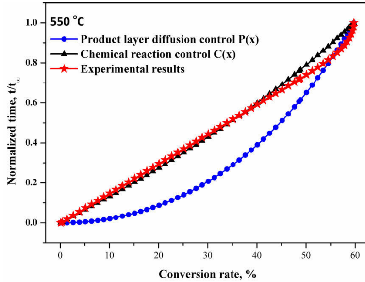
Figure 3. 8 Experimental and calculated P(x) , C(x) vs CaO conversion rate curves at 550 °C
