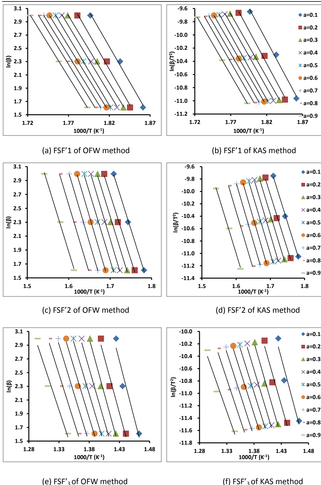
Figure 4. 18 Kinetic plots for the pseudo-components of PVC pyrolysis with CaO reactant between conversion rates of 0.1 and 0.9 using both OFW and KAS methods
