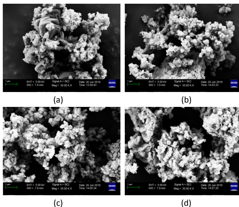
Figure 3. 10 Formation of the product-layer at temperature of 650 °C: a, t/t_f = 0.1 ; b, t/t_f = 0.3 ; c, t/t_f = 0.5 ; d, t/t_f = 1 ( t_f refers to the saturation time of the process)
