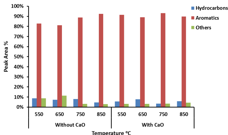
Figure 5. 20 Composition of pyrolytic tar derived from PVC pyrolysis at 550, 650, 750, and 850 °C with/without CaO addition (Others here represent CO 2 , HCl, and acid compounds)
