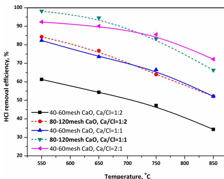
Figure 4. 14 Effect of CaO particle size on HCl mitigation efficiency during PVC pyrolysis with the presence of in-furnace CaO reactant
