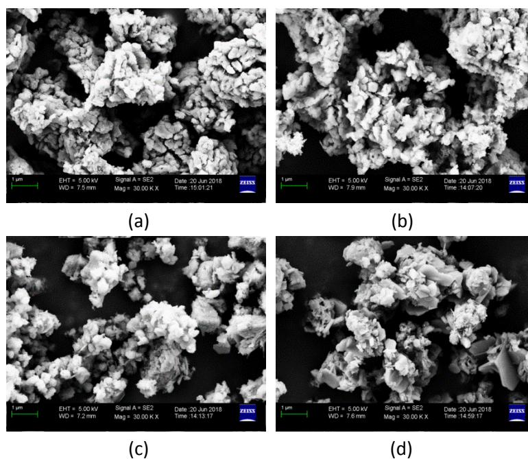
Figure 3. 13 The formed product-layer of the final spent CaO reactants: a, 550 °C; b, 650 °C; c, 750 °C; d, 850 °C
