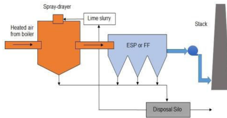
Figure 1. 8 Spray Drying Gas Cleaning System, data obtained from Razvan Lisnic et al. [74]
