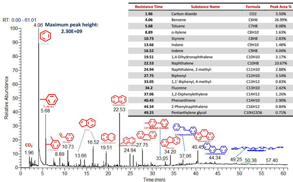
Figure 5. 14 Identified tar composition from PVC pyrolysis at 550 °C in the absence of CaO reactant
