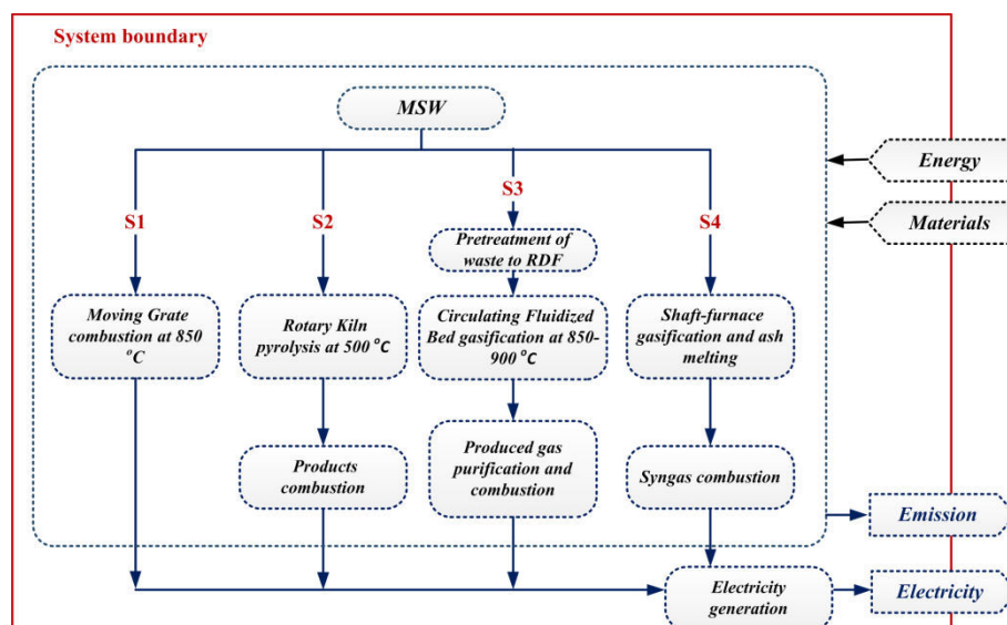
Figure 7. 1 System boundary of the considered scenarios
