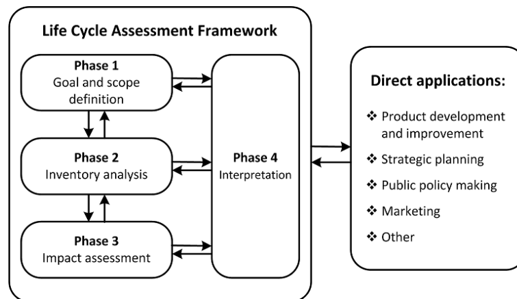
Figure 1. 9 Phases and applications of an LCA standardized by ISO, data obtained from the work of Jun Dong [102]
