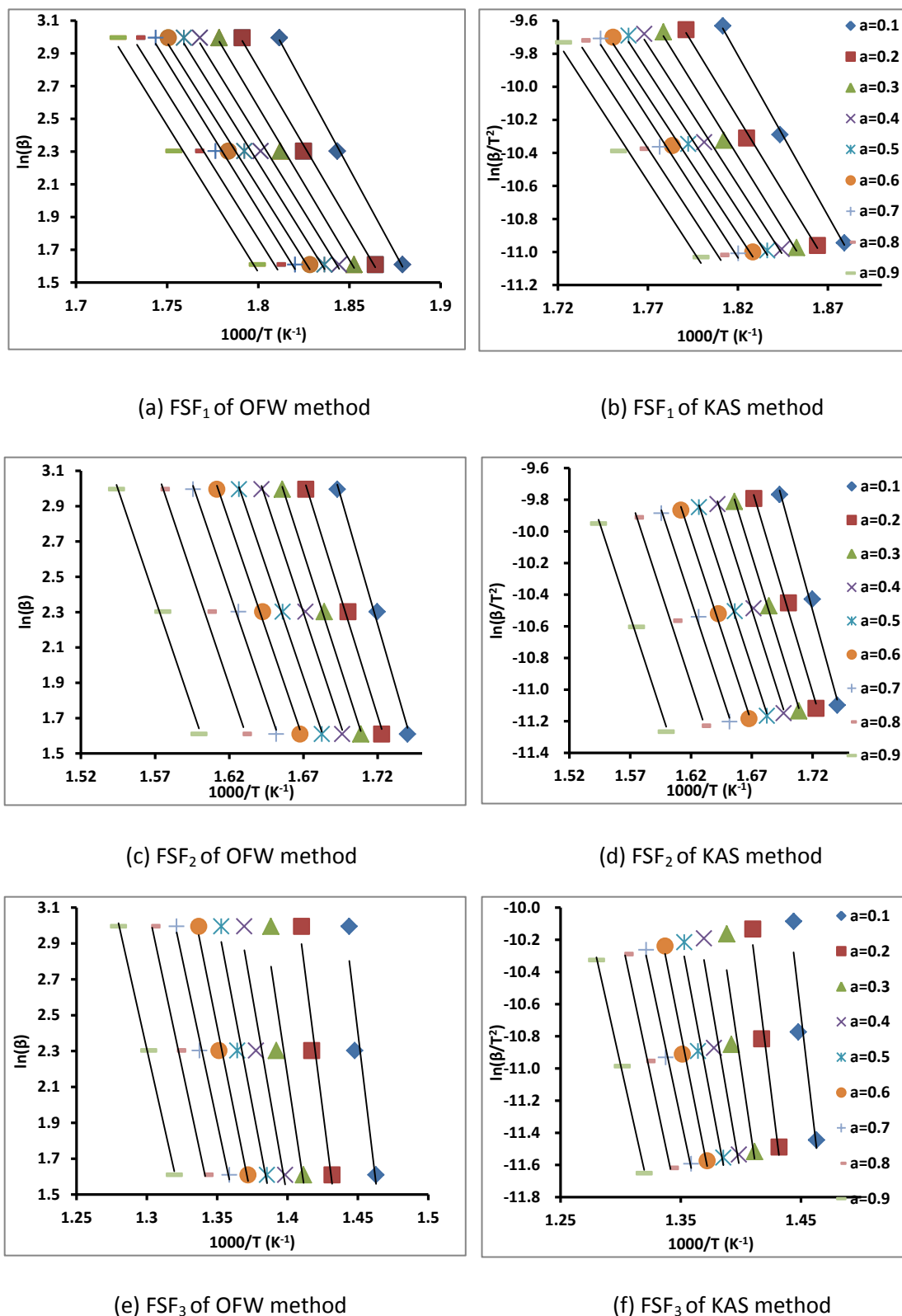
Figure 4. 17 Kinetic plots for the pseudo-components of PVC pyrolysis between conversion rates of 0.1 and 0.9 using both OFW and KAS methods
