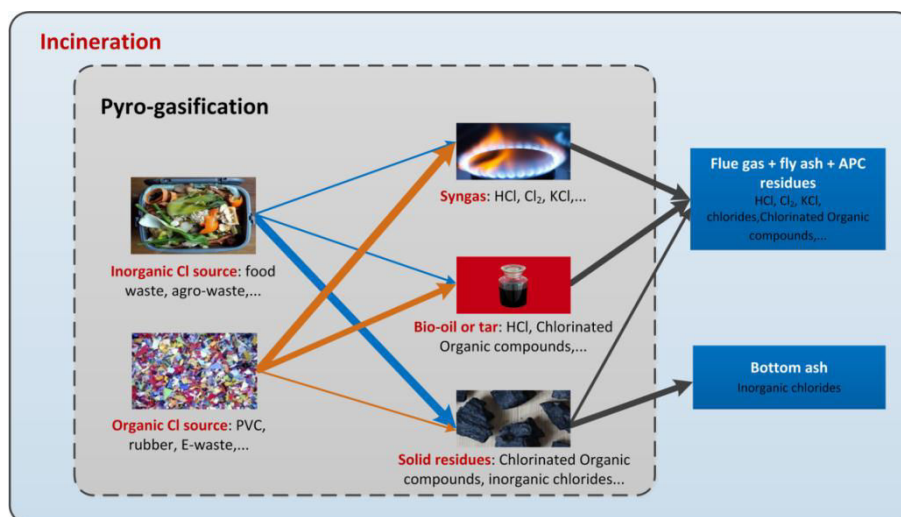
Figure 4. 1 Schematic diagram of the possible conversion routes of chlorine during MSW thermal treatments
