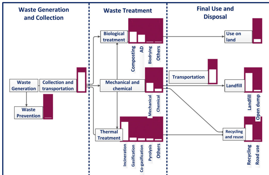
Figure 1. 10 LCA concerns in waste management field, data source from Laurent et al. [125]
