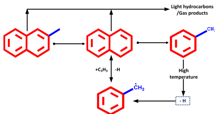
Figure 5. 24 Schematic diagram of the formation and cracking of naphthalene with CaO reactant
