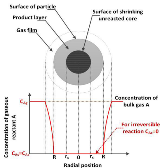
Figure 3. 2 Concentration of HCl under the condition that the reaction is only limited by gas film diffusion (A refers to HCl gas)
