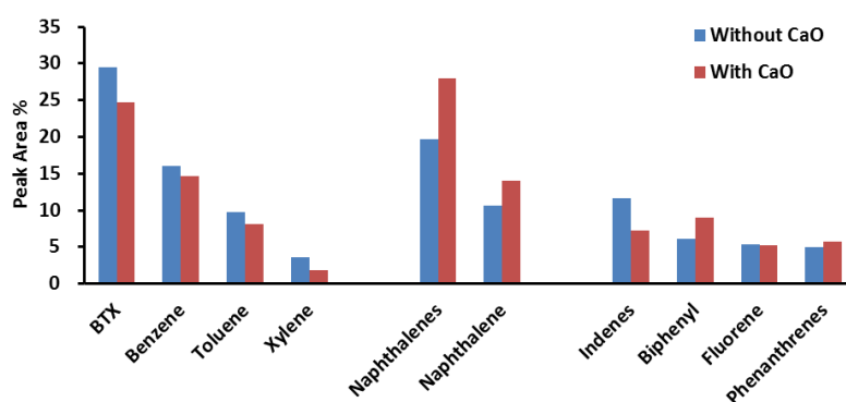
Figure 5. 13 The relative content of BTX, Naphthalene, Indene, Biphenyl, Fluorene, and Phenanthrene in pyrolytic tar derived from PVC pyrolysis at 750 °C without/with CaO reactant
