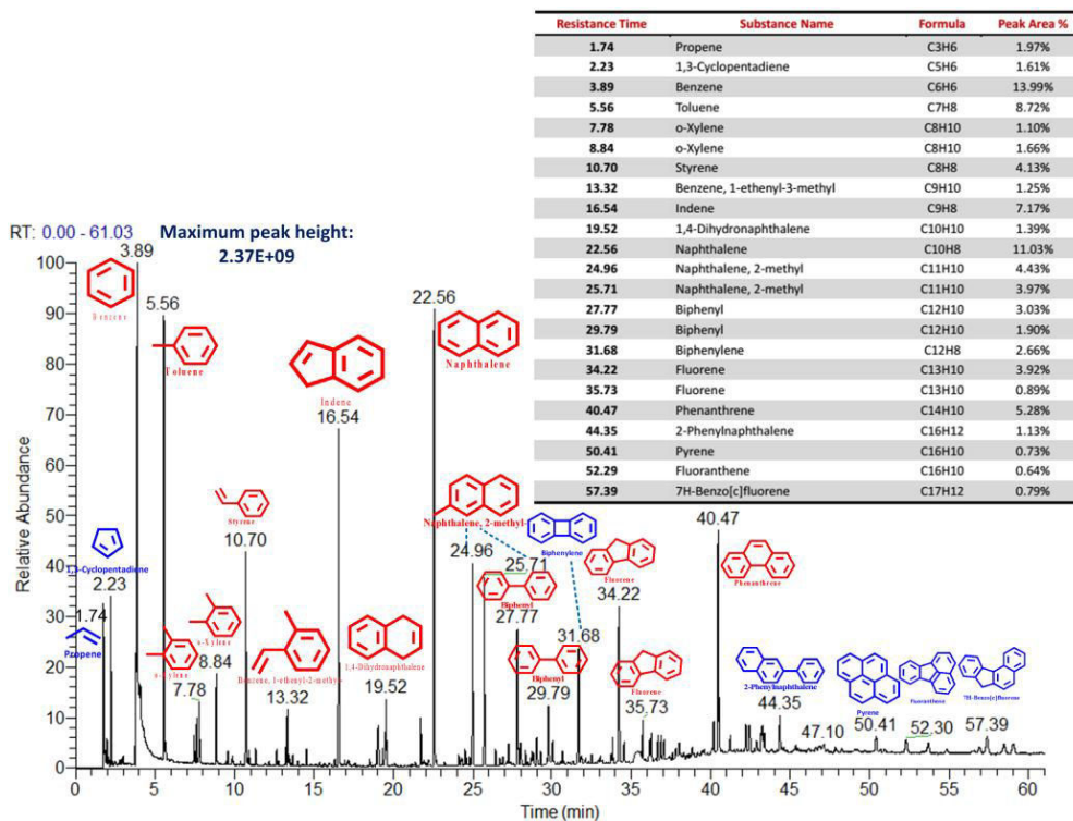
Figure 5. 18 Identified tar composition from PVC pyrolysis at 850 °C in the absence of CaO reactant
