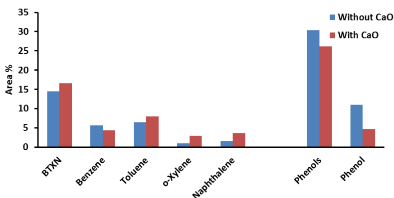
Figure 5. 5 The relative content of BTXN and Phenols in pyrolytic tar derived from wood biomass pyrolysis at 750 °C without/with CaO reactant
