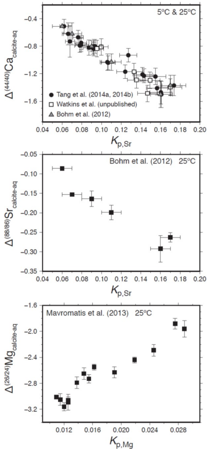
Figure 7. Stable isotope fractionation of a) Ca, b) Sr and c) Mg correlated with their partitioning between calcite and fluid. Watkins et al. (2017)
