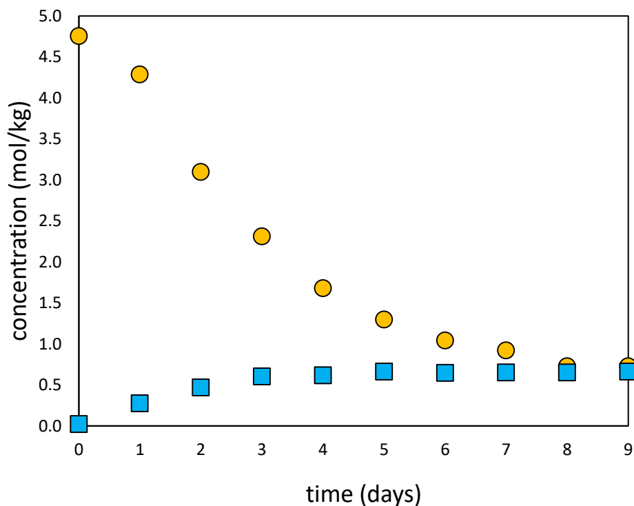
Figure 12. Results of C15 and C16 Ni co-precipitation experiments started without and with Ni in the reactor at the beginning of the experiment. Blue squares correspond to experiment C15 where no Ni was present in reactors at the beginning of the run. Orange circles represent experiment C16 where Ni was added to the reactor prior to the beginning of the run.
