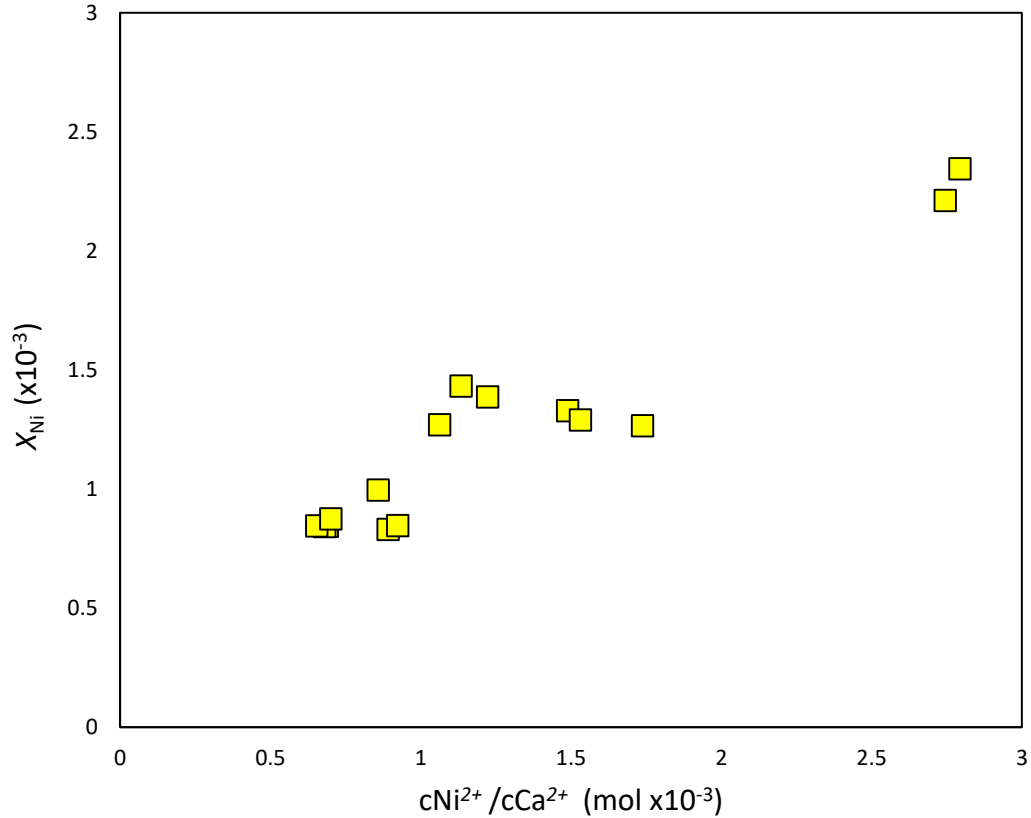
Figure 29. Ni molar fraction in calcite, X_{\text{Ni}} , as a function of the steady state \text{Ni}^{2+} to \text{Ca}^{2+} concentration ratio in the aqueous solution. The error associated with these measurements is included within the symbol size.
