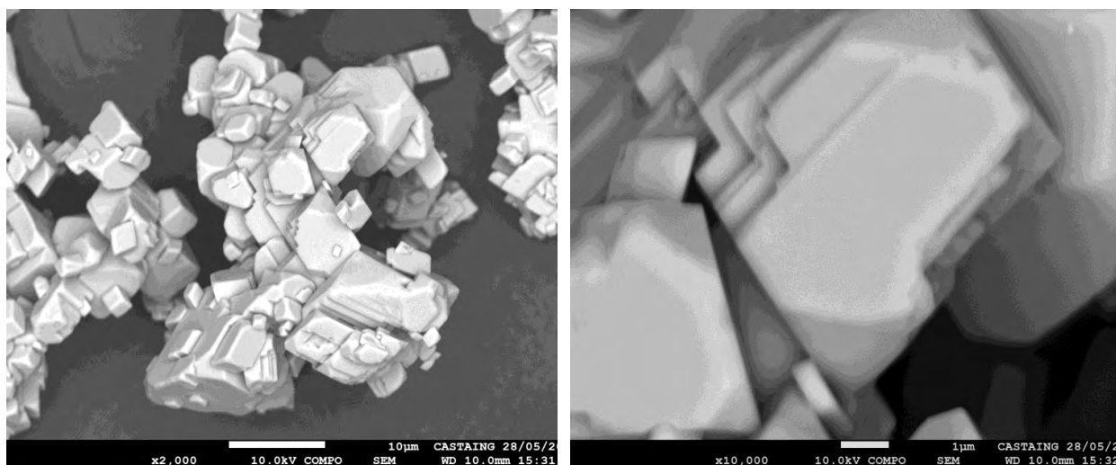
Figure 1. SEM images of the synthetic calcite used in the present study. The scale bar in the left image is 10 \mu\text{m} long, whereas the scale bar in the right image is 1 \mu\text{m} long.
