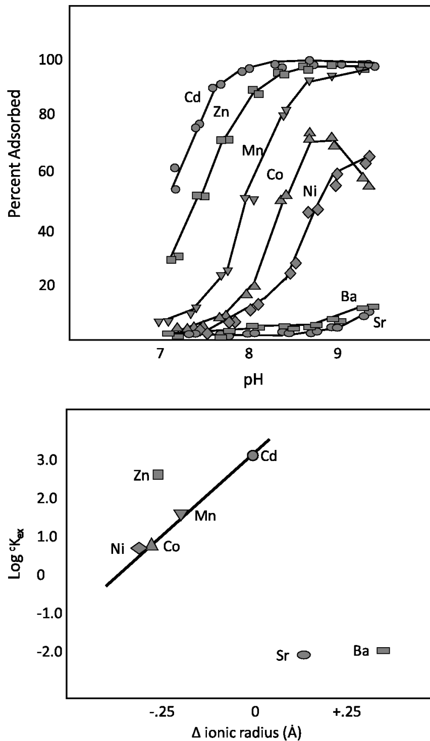
Figure 4. Adsorption of divalent cations on calcite (top) and the relationship between the difference in ionic radius between the Me^{2+} and calcite and their conditional equilibrium constant (bottom) from (Zachara et al., 1991)
