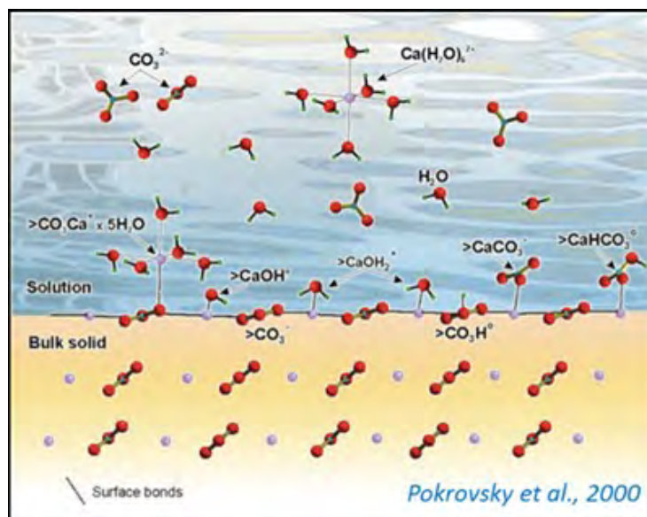
Figure 2. Speciation at the calcite-fluid interface. Figure taken from Pokrovsky et al. (2000).
