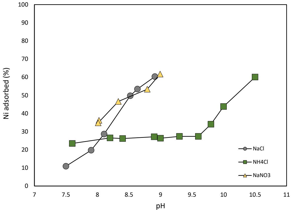
Figure 11. Effect of background electrolyte on the adsorption edge of Ni. The experiments shown were conducted using different background electrolytes: grey circles represent experiments where NaCl was used, green squares show experiments performed using NH 4 Cl, and yellow triangles show experiments performed using NaNO 3 as a background electrolyte. All experiments were kept at 25°C, atmospheric pCO 2 , and 0.1 ionic strength.
