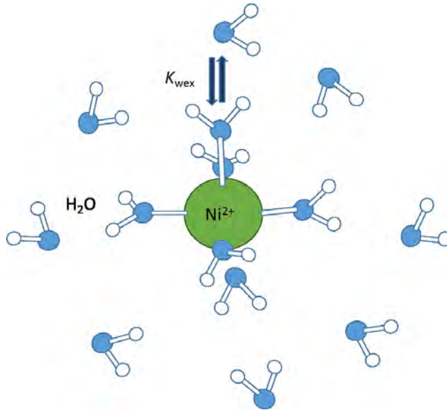
Figure 6. Sketch of the Ni^{2+} aqueous ion
