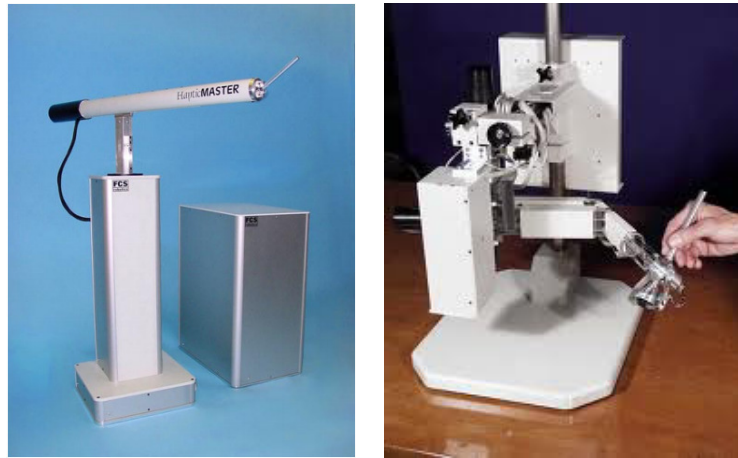
(a) HapticMaster de FCS Control Systems (b) Freedom 6s
