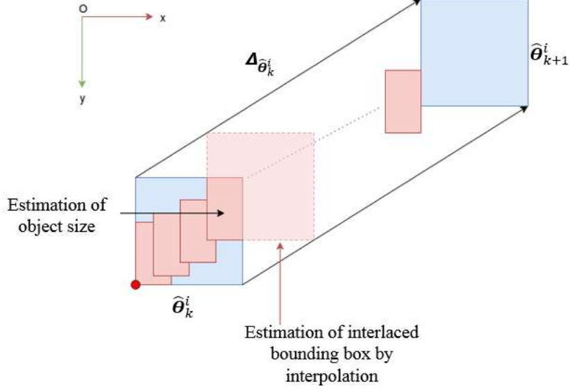
Figure 4.4: Estimation of bounding boxes by interpolation strategy. The interpolation makes it possible to determine the size of an object that is assumed to be constant over all the interlacing strategies.
