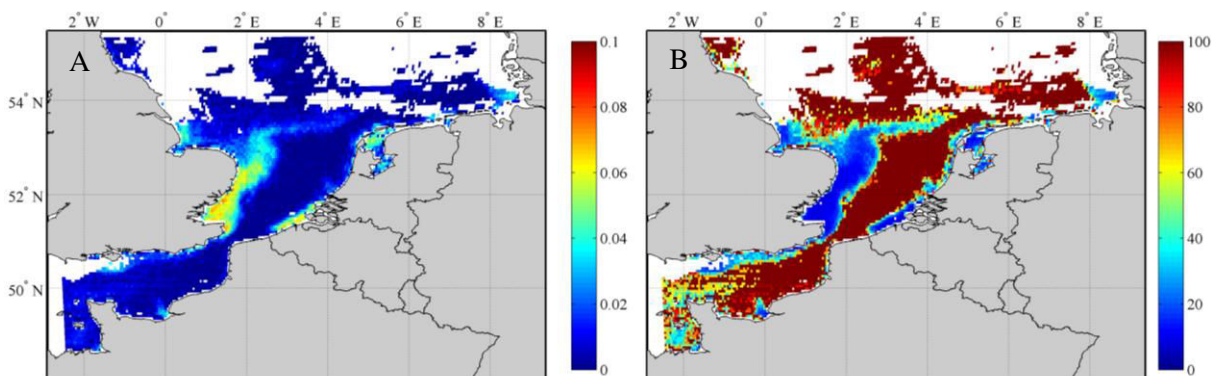
Figure 4.14. (A) Marine reflectance from SEVIRI VIS06 on 16-02-08 at 13:00 h UTC and (B) associated relative uncertainty in %, obtained from Eq. (4.51).
