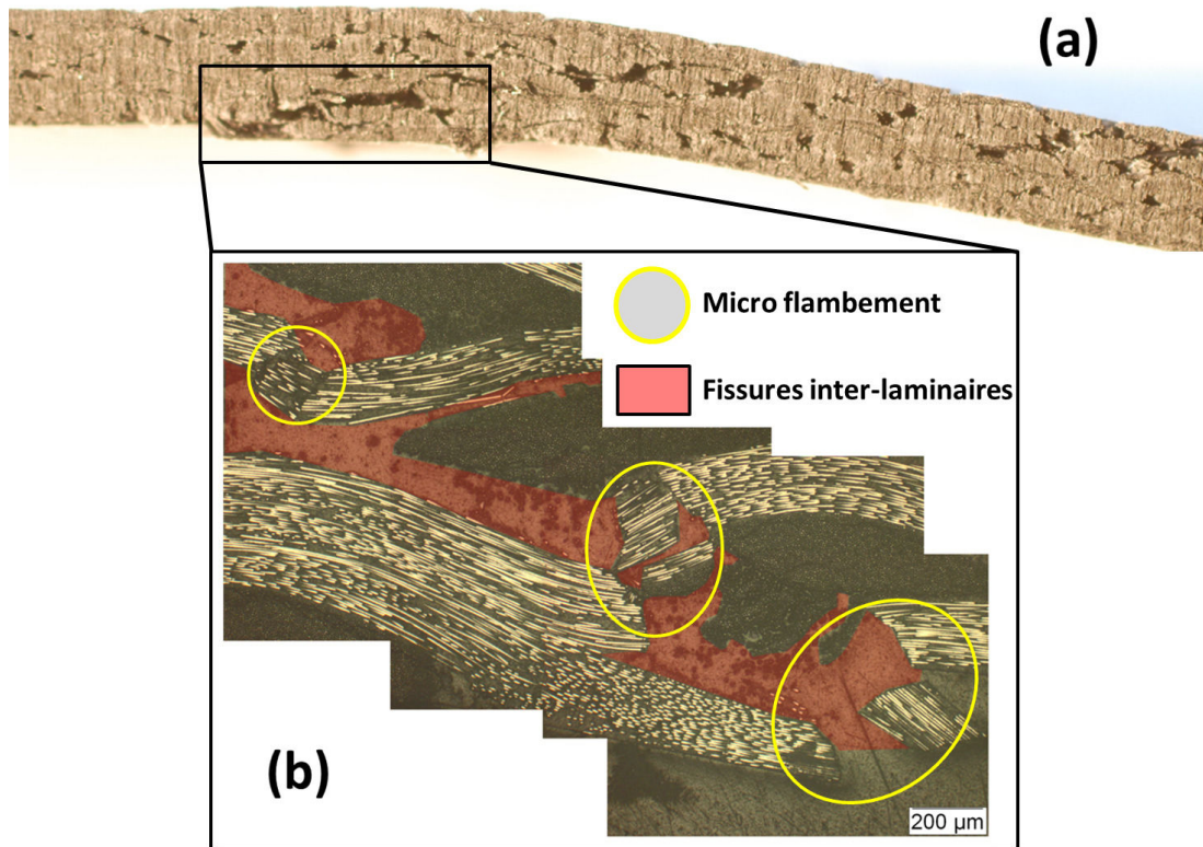
Figure 3.58 – Mode de rupture en flexion de la plaque B4 ( V_p = 12,11\% ) : (a) Observation macroscopique - (b) Micrography (x100)
