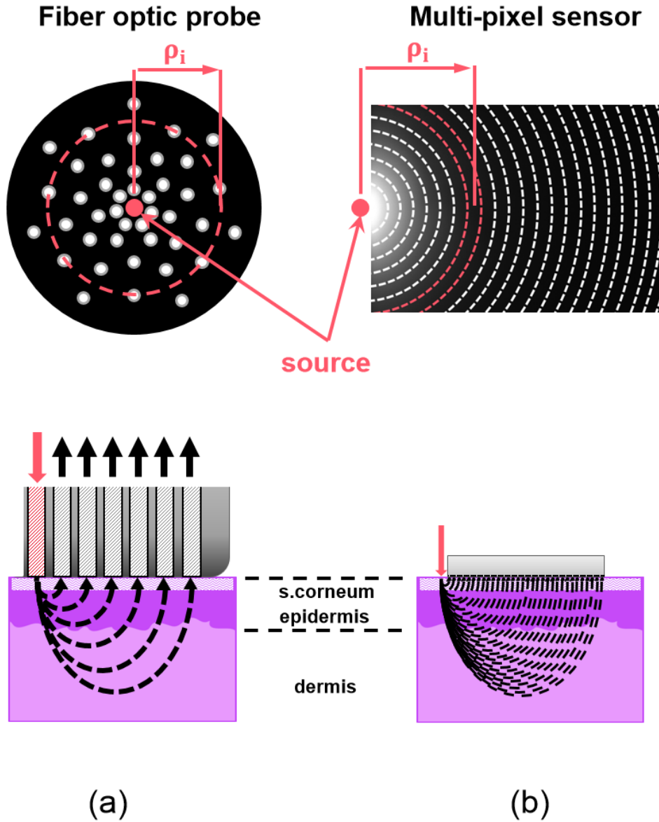
Fig. 2-1 Detection schemes for fiber-based (a) and CMOS-based (b) srDRS instruments. Views from the top (top) and side (bottom) of the instruments are shown. The diffuse reflectance at distance \rho_i to the source is radially averaged (red dotted lines).
