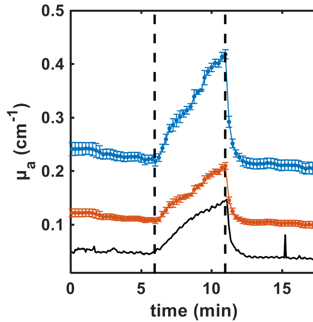
Fig. 4-6 Measured (blue) and scaled (red) \mu_a at 660 nm along with the SSOP measurement at 665 nm. Error bars correspond to standard deviations between properties calculated from different calibration phantom measurements.
