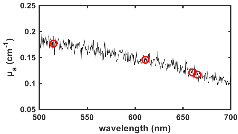
Fig. 4-2 Extrapolation of the calibration phantom absorption coefficient. The black line is the extrapolated absorption spectrum obtained from srDRS fiber-optic probe measurements. Extrapolated \mu_a at 515nm, 611nm and 660nm are displayed as red circles along with the known \mu_a at 665 nm.
