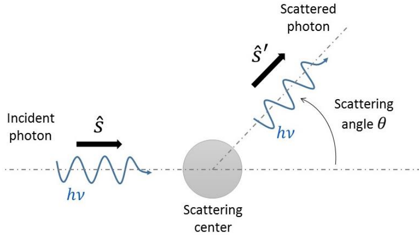
Fig. 1-2 Scattering event. A photon incident on a scattering center with a direction \hat{s} is deviated toward a direction \hat{s}' making an angle \theta with the initial direction.
