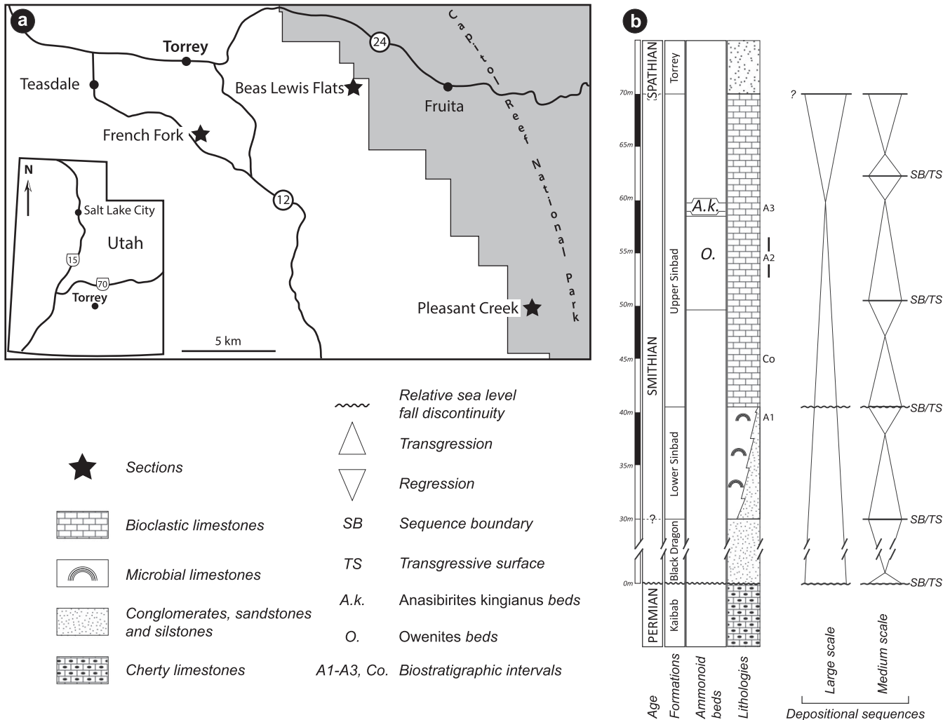
Figure 1. (a) Geographic location of the French Fork, Beas Lewis Flats and Pleasant Creek sections in the Torrey area (southern Utah). (b) Synthetic lithological succession of the Torrey area and its depositional sequence interpretation.
