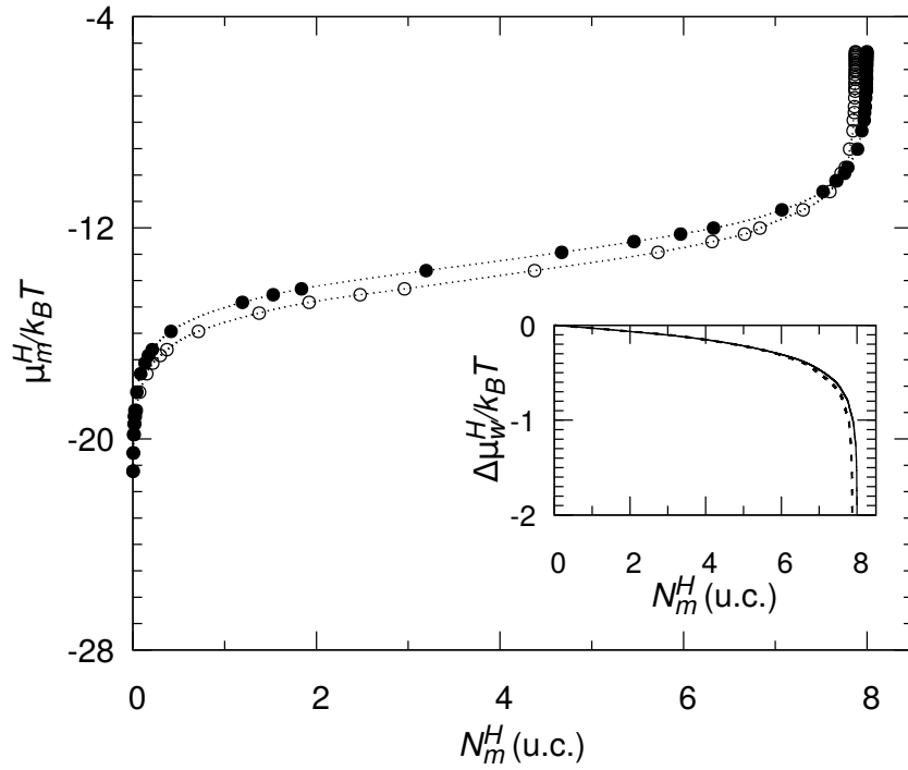
Figure 3.5 Chemical potential of methane, \mu_m^H , versus number of methane molecules, N_m^H , in methane hydrate at T = 250 K and P = 10 atm. N_m^H is expressed as the number of methane molecules per methane hydrate unit cell. The empty and filled circles are for TIP4P/Ice and TIP4P/2005 water models, respectively. The dotted lines correspond to cubic interpolation of the data. The insert shows the chemical potential difference of water relative to the zero-occupancy methane hydrate, \Delta\mu_w^H = \mu_w^H - \mu_w^H(x_m = 0) , as a function of the number of methane molecules, N_m^H (these data are obtained from N_m(\mu_m) using Eq. (3.9)). The dashed and solid lines are for the TIP4P/Ice and TIP4P/2005 water models. All chemical potentials are normalized to the thermal energy, k_B T .
