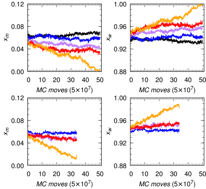
Figure B.2 (color online) Methane ( x_m , left panels) and water ( x_w , right panels), mole fractions during the different GCMC simulation runs: T = 230 K (black), 240 K (blue), 250 K (purple), 260 K (red), and 270 K (orange) for D_p = 2.8554 nm (top panels); and T = 260 K (blue), 270 K (purple), 280 K (red), and 290 K (orange) for D_p = 5.2308 nm (bottom panels). The x -axis, which indicates progress along the GCMC simulation, is expressed as a number of attempted MC moves where one move is a molecule translation, rotation, insertion or deletion. The dimensions of the simulation box are: L_x = 2.3754 nm, L_y = 4.7508 nm, and L_z = 4.3670 nm for D_p = 2.8554 nm (top panels) while L_z = 6.7424 nm for D_p = 5.2308 nm (bottom panels).
