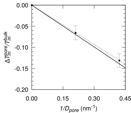
Figure B.3 Shift in the melting temperature of confined methane hydrate with respect to the bulk, \Delta T_m^{pore}/T_m^{bulk} , as a function of the reciprocal of the pore width, 1/D_p : the dashed line is for the larger molecular system (i.e., L_y = 4.3670 nm); while the solid line is for the smaller one (i.e., L_y = 2.3754 nm). Note that T_m^{pore} for larger system reads from Figure B.2, while T_m^{bulk} and k_{GB} are estimated using these data.
