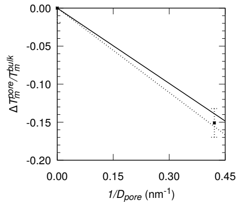
Figure B.5 Shift in the melting temperature of confined methane hydrate with respect to the bulk, \Delta T_m^{pore}/T_m^{bulk} , as a function of the reciprocal of the pore width, 1/D_p : the dashed line is for P = 10 atm while the solid line is for P = 100 atm. The black circles read from Figure B.4 (DCM simulations); while the dashed and solid lines are computed using k_{GB} = (\gamma_{LS}v^L - \gamma_{HS}v^H)/\Delta h_{fus} .
