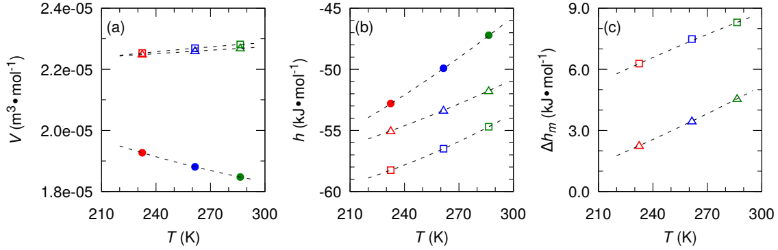
Figure 4.6 (color online) Molar volume v (a) and molar enthalpy h (b) of liquid water (solid circles), full-methane hydrate (empty squares), and empty-methane hydrate (empty triangles). Enthalpy of melting \Delta h_m (c) from full-methane hydrate (empty squares) to liquid water and from empty-methane hydrate (empty triangles) to liquid water using MD simulations. The dashed lines indicate that these parameters are along the L–H–V phase boundary for bulk phase: the red, blue, and green colors are for (T, P) = (233 \text{ K}, 1 \text{ atm}) , (262 \text{ K}, 10 \text{ atm}) , and (286 \text{ K}, 100 \text{ atm}) , respectively. All the thermodynamic parameters are per mole of water.
