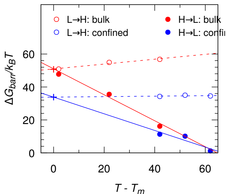
Figure 4.11 (color online) Free energy barriers, \Delta G_{barr}/k_B T , between methane hydrate and liquid water as a function of the shift with respect to the melting point, T - T_m , for bulk phase (red) and for confined phase (blue): (1) free energy barriers from liquid water to methane hydrate, i.e., methane hydrate formation ( left ), \Delta G_{barr}^{L \rightarrow H} ; and (2) free energy barrier from methane hydrate to liquid water, i.e., methane hydrate dissociation ( right ), \Delta G_{barr}^{H \rightarrow L} . The red cross is for bulk methane hydrate while the blue cross is for confined methane hydrate using the extrapolation described in the text. The free energy barriers are normalized using the thermal energy, k_B T .
