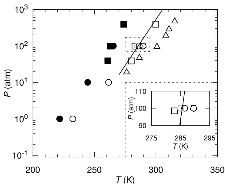
Figure 3.7 Pressure–Temperature phase diagram of methane hydrate as determined using free energy calculations (circles, this work), direct coexistence method (gray pentagon, this work), hyper parallel tempering method (black pentagon, this work). The empty and filled symbols are for TIP4P/Ice and TIP4P/2005 water models, respectively. The empty and filled squares are the results obtained for TIP4P/Ice and TIP4P/2005 by Conde et al. (Conde and Vega, 2010) using the direct coexistence method. The empty triangles are the free energy calculations for TIP4P/Ice by Jensen et al. (Jensen et al., 2010). The solid line shows the experimental data by Sloan et al. (Sloan, 2003). The insert shows a zoomed view of the region shown depicted as a dashed rectangle in the main figure.
