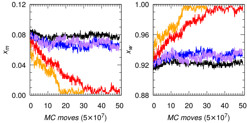
Figure 4.3 (color online) Pore size, D_p , effect on the melting temperature, T_m^{pore} , of confined methane hydrate/liquid water using the direct coexistence method: methane ( x_m , left ), and water ( x_w , right ) mole fractions for D_p = 2.8554 nm during the different GCMC simulation runs at T = 230 K (black), 240 K (blue), 250 K (purple), 260 K (red), and 270 K (orange). The x -axis, which indicates progress along the GCMC simulation, is expressed as a number of attempted MC moves where one move is a molecule translation, rotation, insertion or deletion.
