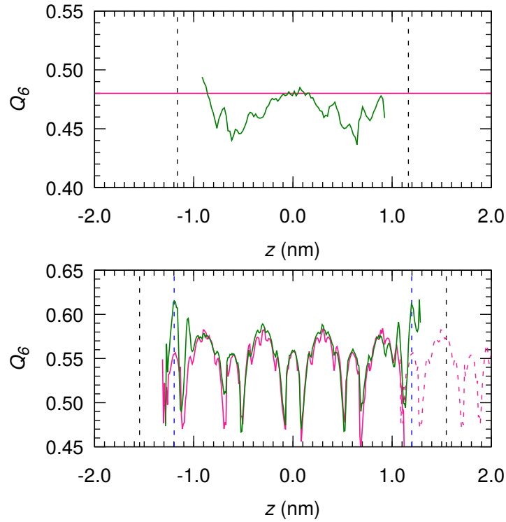
Figure 5.3 Local bond order parameters along the z -axis, Q_6(z) , in liquid water ( top ) and methane hydrate ( bottom ) at T = 240 K and P = 100 atm. The red solid lines are for bulk phases while the green solid lines are for confined phases. The black dashed lines are the positions of the pore walls with the pore width D_p . The blue dashed lines indicate the dimension in the z -direction for bulk methane hydrate with L_z = 2 u. The red dashed lines are the local bond order parameters for a duplicated bulk phase.
