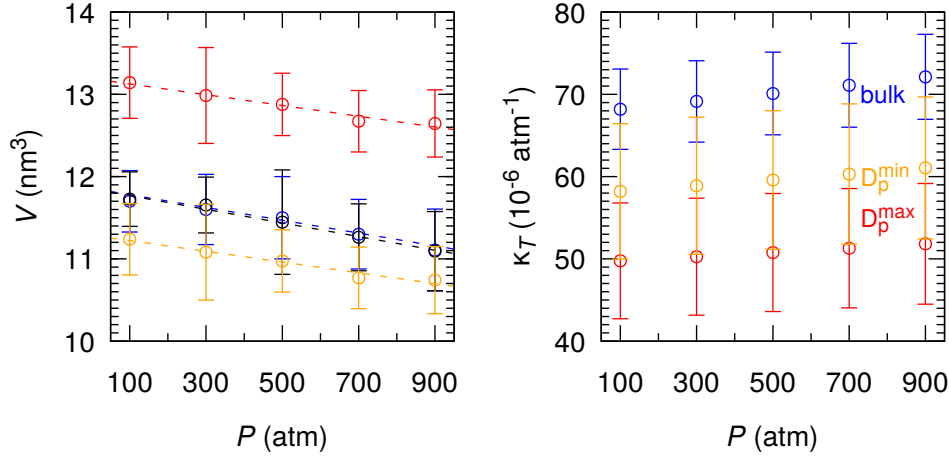
Figure 5.6 (color online) Volume ( V , left) and isothermal compressibility ( \kappa_T , right) of bulk and confined liquid water as a function of pressure P at T = 240 K. Two different ensembles were considered for bulk liquid water: NPT ensemble (blue circles) and NP_zT ensemble (black circles). For confined liquid water, a minimum value D_p^{min} (orange circles) and a maximum value D_p^{max} (red circles) of the pore width were considered. The dashed lines are linear fits.
