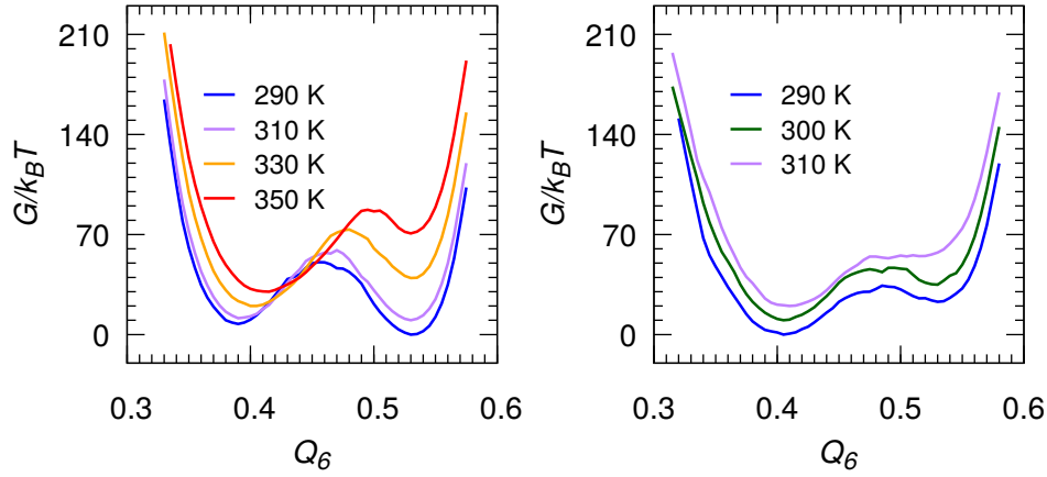
Figure 4.9 (color online) Free energy, G , of methane hydrate and liquid water in bulk phase ( left ) and in confined phase for D_p = 2.8554 nm ( right ) as a function of the local bond order parameter, Q_6 . G(Q_6) of bulk phase ( left ) is shown at T = 290 K (blue), 310 K (purple), 330 K (orange) and 350 K (red). G(Q_6) upon confinement ( right ) is shown at T = 290 K (blue), 300 K (green), and 310 K (purple). The free energy is normalized using the thermal energy, k_B T . For the sake of clarity, a shift of +10, +20, and +30 in G/k_B T is added for the bulk phase at T = 310 K, 330 K, and 350 K. A shift of +10 and +20 in G/k_B T is added for the confined phase at T = 300 K and 310 K.
