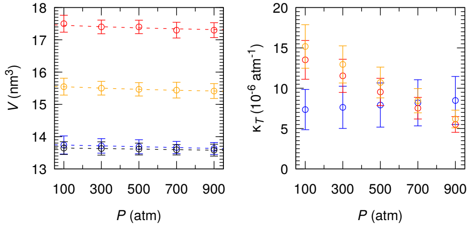
Figure 5.7 (color online) Volume ( V , left) and isothermal compressibility ( \kappa_T , right) of bulk and confined methane hydrate as a function of pressure P at T = 240 K. Two different ensembles were considered for bulk methane hydrate: NPT ensemble (blue circles) and NP_zT ensemble (black circles). For confined methane hydrate, a minimum value D_p^{min} (orange circles) and a maximum value D_p^{max} (red circles) of the pore width were considered. The dashed lines are linear fits.
