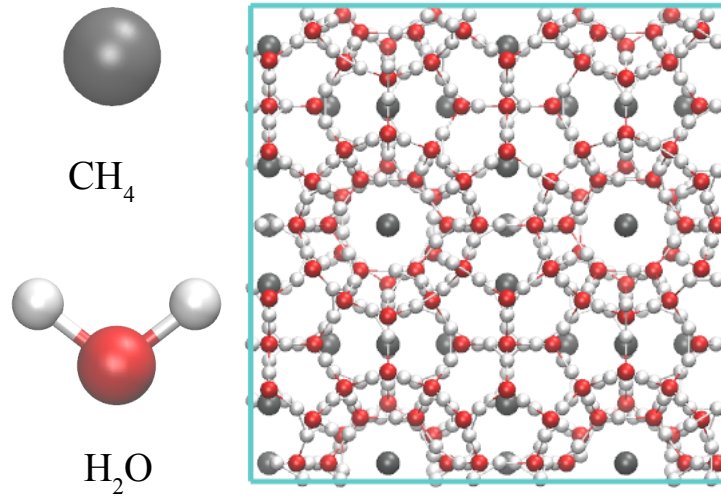
Figure 3.1 (color online) Molecular configuration of methane hydrate with structure sI. The red and white spheres are the oxygen and hydrogen atoms of water, respectively. The gray spheres are the methane molecules which are trapped inside the hydrogen-bonded cages formed by water molecules (1 methane molecule for 8 water molecules). The dimensions of this molecular configuration, which corresponds to 2 \times 2 \times 2 unit cells, are: L_x = L_y = L_z = 2.3754 nm.
