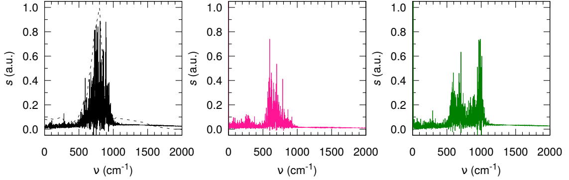
Figure 5.9 (color online) Fourier transform \mathcal{F}[\nu] of the autocorrelation function of the heat-flux for bulk ( h(t) , left ) and confined ( h_T(t) , center ; h_N(t) , right ) methane hydrate. For bulk methane hydrate, the black solid line is from this work while the black dashed line is from English et al. (English and Tse, 2009; English et al., 2009). For confined methane hydrate, the red solid line is for h_N = V/k_B T \langle J_z(t) J_z(0) \rangle while the green solid line is for h_T = V/2k_B T \langle J_x(t) J_x(0) + J_y(t) J_y(0) \rangle .
