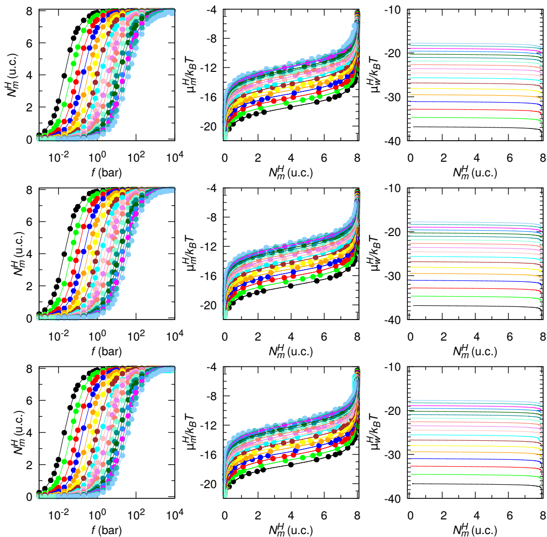
Figure A.5 Same as Figure A.4 but for the TIP4P/Ice water model.
