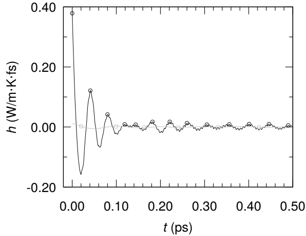
Figure 5.10 Inverse Fourier transform of the power spectrum for bulk methane hydrate. The acoustic mode (gray line) and optical mode (black line) are separated as described in the text. The maxima/peaks of the optical modes (black circles) and the smoothed points for the acoustic modes (gray circles) are considered to determine the relaxation time and amplitudes ( see text ).
