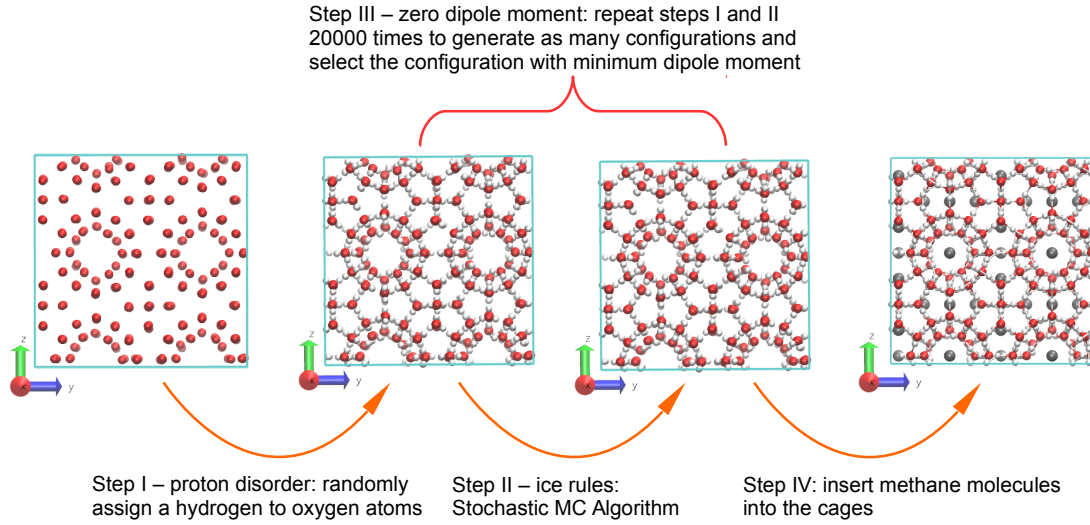
Figure 3.2 Stochastic algorithm to generate methane hydrate molecular configurations with sI structure (Buch et al., 1998): (1) set the oxygen positions according to the experimental X-ray crystallographic data (Kirchner et al., 2004); (2) generate proton disorder by randomly assigning a hydrogen atom to one of the oxygen atoms in each O–O pair (step I); (3) use a stochastic MC algorithm to verify the ice rules (step II); (4) repeat steps I and II 20000 times to generate as many configurations and select the configuration with minimum dipole moment (step III); and (5) insert the methane molecules into the cages of the methane hydrate (step IV). The red and white spheres are the oxygen and hydrogen atoms of water, respectively. The gray spheres are the methane molecules. The dimensions of the system shown here are L_x = L_y = L_z = 2.3754 nm which correspond to 2 \times 2 \times 2 unit cells.
