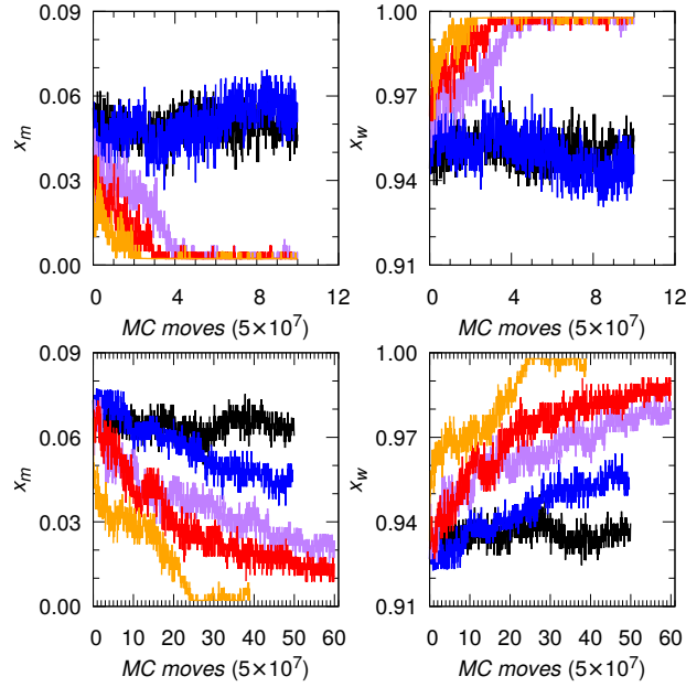
Figure B.4 (color online) Methane ( x_m , left panels ) and water ( x_w , right panels ) mole fractions during the different GCMC simulation runs: T = 250 K (black), 260 K (blue), 270 K (purple), 280 K (red), and 290 K (orange) for bulk phase ( top panels ); while T = 210 K (black), 220 K (blue), 230 K (purple), 240 K (red), and 250 K (orange) for confined system with D_p = 2.8554 nm ( bottom panels ). The x-axis, which indicates progress along the GCMC simulation, is expressed as a number of attempted MC moves where one move is a molecule translation, rotation, insertion or deletion. The dimensions of the simulation box in x- and y-directions are L_x = L_y = 2.3754 nm, and in z-direction are L_z = 2.3754 nm for bulk system while L_z = 4.3670 nm for confined system. T_m^{bulk} = 265 \pm 5 K and T_m^{pore} = 225 \pm 5 K at P = 10 atm for methane hydrate are summarized in Table 4.1.
