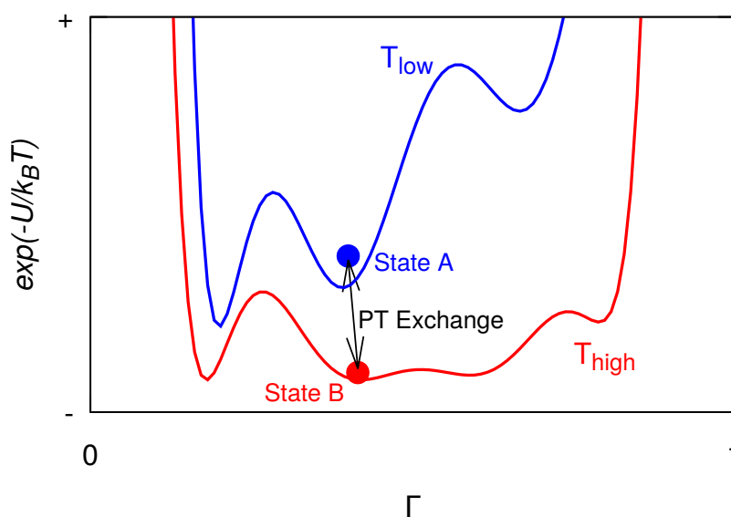
Figure 1.8 Boltzmann factor, \exp(-U/k_B T) , in the phase space, \Gamma , as an example to illustrate the parallel tempering technique. The blue line is for the low temperature, while the red line is for the high temperature. The system in state A (blue circle) remains easily trapped into a metastable state, while the system in state B (red circle) escape more easily. Parallel tempering between A and B is used to make the escape easier.
