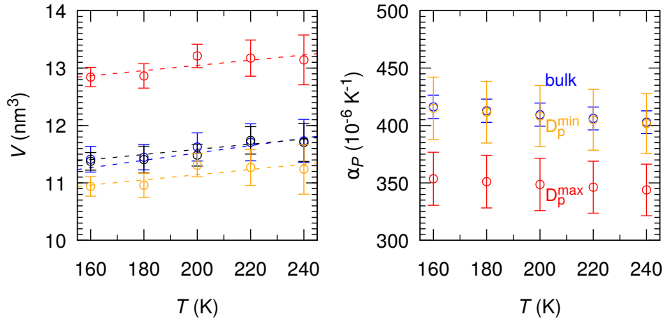
Figure 5.4 (color online) Volume ( V , left) and thermal expansion ( \alpha_P , right) of bulk and confined liquid water as a function of temperature T at P = 100 atm. Two different ensembles were considered for bulk liquid water: NPT ensemble (blue circles) and NP_zT ensemble (black circles). For confined liquid water, a minimum value D_p^{min} (orange circles) and a maximum value D_p^{max} (red circles) of the pore width were considered. A total of 368 water molecules were used to determine these data. The dashed lines are linear fits.
