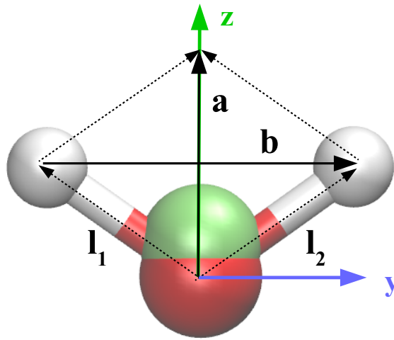
Figure A.1 Definition of the normalized vectors a and b in the 4-site rigid water molecule (TIP4P/2005 and TIP4P/Ice). These two vectors are formed by the subtraction \mathbf{a} = (\mathbf{l}_1 - \mathbf{l}_2)/|\mathbf{l}_1 - \mathbf{l}_2| and summation \mathbf{b} = (\mathbf{l}_1 + \mathbf{l}_2)/|\mathbf{l}_1 + \mathbf{l}_2| of the two bond vectors, \mathbf{l}_1 and \mathbf{l}_2 . The red and white spheres are the oxygen and hydrogen atoms, respectively. The green sphere is the electronic site M of the oxygen atom.
