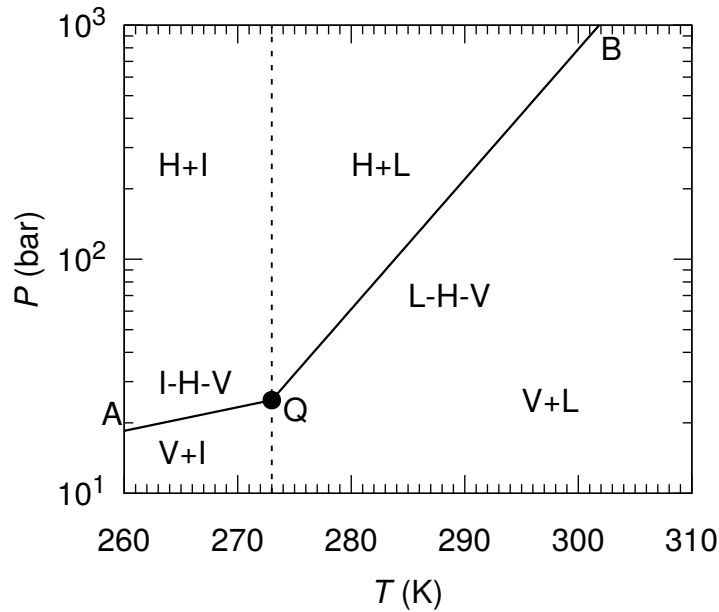
Figure 1.5 Pressure–temperature ( P – T ) phase diagram for liquid (L), ice (I), vapor (V), and hydrate (H) phases. The phase boundary – dashed line – indicates the conditions for which ice coexists with liquid water, L–I. The phase boundary – solid line AQ – indicates the conditions for which methane hydrate coexists with ice and methane vapor, I–H–V. The phase boundary – solid line QB – indicates the conditions for which methane hydrate coexists with liquid water and methane vapor, L–H–V. Four regions involving the two phase coexistence are shown: (1) hydrate coexists with ice, H+I; (2) hydrate coexists with liquid water, H+L; (3) methane vapor coexists with liquid water, V+L; and (4) methane vapor coexists with ice, V+I. Q is a four phase coexistence point, L–H–I–V.
