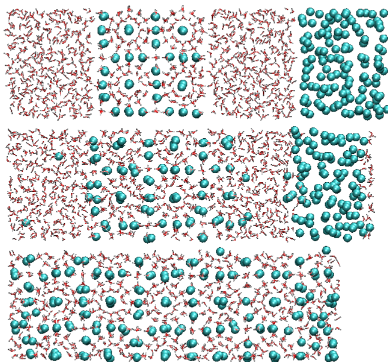
Figure 1.7 (color online) Typical molecular configurations obtained in the direct coexistence method at T = 294 K and P = 600 bar (where methane hydrate is stable): ( top ) the coexisting phases, i.e., liquid water (L) + methane hydrate (H) + methane vapor (V), are the initial configuration; ( center ) the growth of methane hydrate; and ( bottom ) the perfect methane hydrate formed at the end of the molecular simulation. The red and white lines denote the water molecules while the blue spheres are the methane molecules. [Picture from Ref. (Conde and Vega, 2010)]
