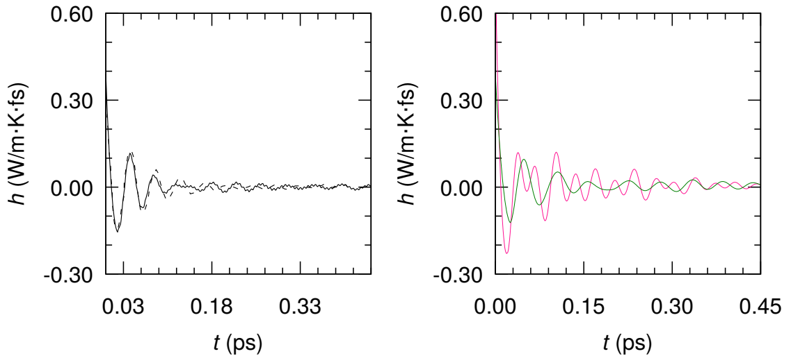
Figure 5.8 (color online) Autocorrelation function of the heat-flux vector, h(t) , as a function of time, t , for bulk (left) and confined (right) methane hydrate. For bulk methane hydrate, the black solid line is from this work while the black dashed line is from English et al. (English and Tse, 2009; English et al., 2009). For confined methane hydrate, the red solid line is the tangential component h_N = V/k_B T \langle J_z(t) J_z(0) \rangle while the green solid line is the normal component h_T = V/2k_B T \langle J_x(t) J_x(0) + J_y(t) J_y(0) \rangle .
