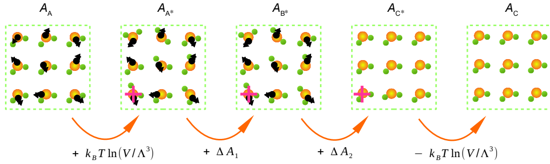
Figure 3.3 Thermodynamic path used in the Einstein molecule approach to calculate the free energy of the zero-occupancy methane hydrate, A_C . Orange and green spheres are the oxygen and hydrogen atoms of water, respectively. The green box shows the periodic boundary conditions of the simulation cell. The superscript * indicates that the system has one of its water molecules at a fixed position shown by the big pink '+' sign ( see text ). A_A is the free energy of the non-interacting Einstein molecule while A_{A*} is the free energy of the same system with one of its water molecules at a fixed position. A_{B*} is the free energy of the interacting Einstein molecule with one of its water molecules at a fixed position. A_{C*} is the free energy of the zero-occupancy methane hydrate with one of its water molecules at a fixed position while A_C is the free energy of the same system without fixing any water molecule positions. Constraining a water molecule position (3 degrees of freedom) increases the free energy by k_B T \ln(V/\Lambda^3) . The change in free energy between the non-interacting and interacting Einstein molecule is \Delta A_1 = A_{B*} - A_{A*} . The change in free energy between the constrained interacting Einstein molecule and the constrained methane hydrate is \Delta A_2 = A_{C*} - A_{B*} ( see text ).
