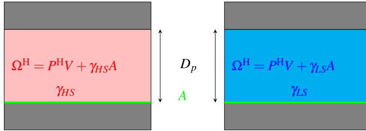
Figure 4.5 (color online) Gibbs-Thomson equation for L–H–V equilibrium upon confinement: methane hydrate (H, red region) and liquid water (L, blue region) are confined in a slit pore of a width D_p formed by two parallel substrates (S, the gray regions). \Omega^H and P^H are the grand potential and pressure of methane hydrate while \Omega^L and P^L are the grand potential and pressure of liquid water. \gamma_{LS} is the surface tension of liquid water–substrate (LS) interface while \gamma_{HS} is the surface tension of methane hydrate–substrate (HS) interface. V = D_p A is the pore volume where A is the surface area.
