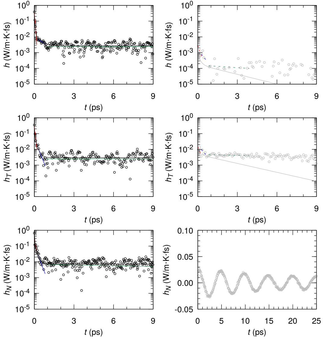
Figure 5.11 (color online) Piecewise linear fits applied to the acoustic – smoothed points – (gray circles, right panels ) and optical – maxima/peaks – (black circles, left panels ) modes for bulk methane hydrate ( top panels ) and the tangential ( center panels ) and normal ( bottom panels ) components of confined methane hydrate. Piecewise linear fits for optical modes are shown for short-range (red solid lines), long-range (blue solid lines), and constant term (green solid lines) terms. for h_N(t) , two optical modes are included but only one optical mode ( \omega_j = 186.7 rad/ps) is shown here (the fit results for the other one are shown in Table 5.2). Piecewise linear fits for acoustic modes are shown for short-range (red hashed lines), medium-range (blue dashed lines), and long-range (green dashed lines) terms. The black solid lines are for overall optical fits while the gray solid lines are for overall acoustic fits.
