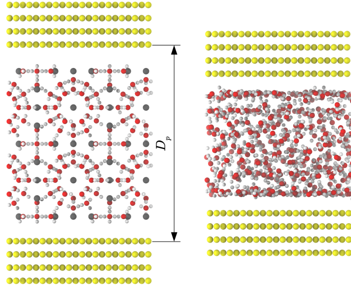
Figure 5.1 (color online) Molecular configuration of confined methane hydrate ( left ) and liquid water ( right ). The red and white spheres are the oxygen and hydrogen atoms of water, respectively. The gray spheres are the methane molecules which are inside the hydrogen-bonded cages formed by water molecules. The yellow spheres are the solid atoms of the pore walls. Pore walls are set as described in Chapter 4 but with pistons at the top wall and bottom wall. In this specific configuration, the sI methane hydrate with dimensions of L_x = L_y = L_z = 2.3754 nm is confined inside the porosity ( left ). The liquid water ( right ) is obtained by first removing methane molecules and then melting the hydrate phase in the canonical ensemble followed by simulations at constant pressure. The dimensions of the simulation box are L_x = L_y = 2.3754 nm and L_z = 44.5734 nm ( left ) and 41.4932 nm ( right ). Periodic boundary conditions are used along the x - and y -directions.
