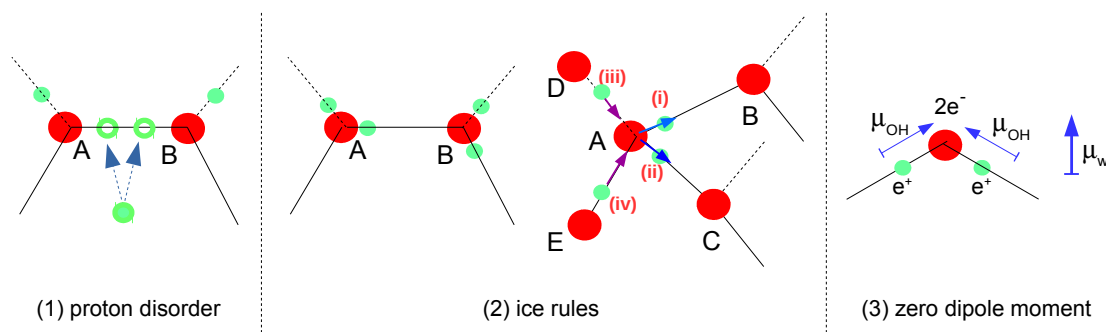
Figure 1.2 Three criteria should be satisfied for methane hydrate with sI structure (Bernal and Fowler, 1933; Chakraborty and Gelb, 2012a): (1) proton disorder; (2) ice rules; and (3) zero dipole moment. The red and green spheres are the oxygen and hydrogen atoms of water, respectively.
