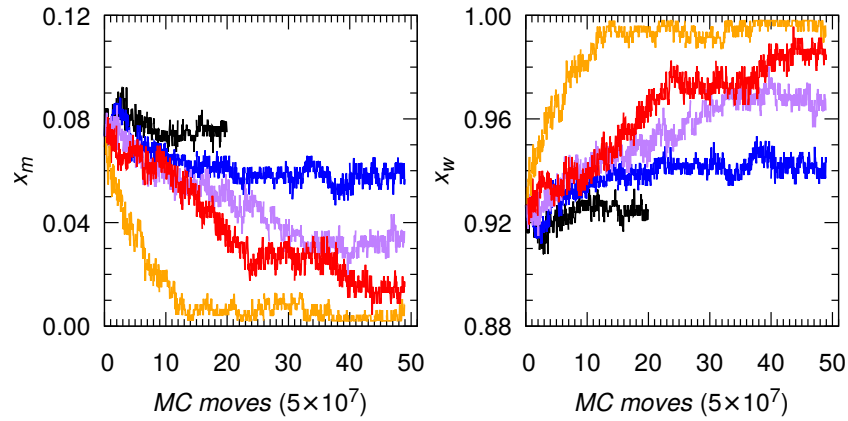
Figure B.1 (color online) Methane ( x_m , left ) and water ( x_w , right ) mole fractions during the different GCMC simulation runs: T = 230 K (black), 240 K (blue), 250 K (purple), 260 K (red), and 270 K (orange). The x -axis, which indicates progress along the GCMC simulation, is expressed as a number of attempted MC moves where one move is a molecule translation, rotation, insertion or deletion. The dimensions of the simulation box are: L_x = L_y = 2.3754 nm and L_z = 8.3674 nm (corresponding to D_p = 2.8554 nm with a vacuum layer D_v = 2.0000 nm in each side).
