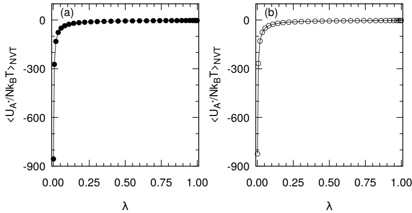
Figure A.3 Canonical ensemble average of the harmonic potential energy U_{A^*} as a function of the coupling parameter \lambda at T = 250 K and P = 100 atm: (a) TIP4P/2005 water model (filled circles) and (b) TIP4P/ICE water model (empty circles). These values are obtained from several canonical ensemble MC simulations for the hybrid potential energy, U(\lambda) = (1 - \lambda)U_{C^*} + \lambda U_{B^*} . The first molecule in the corresponding molecular system have a fixed position in all these MC simulations. All energies are normalized to the thermal energy k_B T . The absolute error bar for each average energy is smaller than 0.6.
