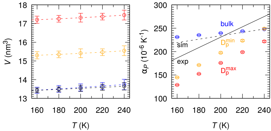
Figure 5.5 (color online) Volume ( V , left) and thermal expansion ( \alpha_P , right) of bulk and confined methane hydrate as a function of temperature T at P = 100 atm. Two different ensembles were considered for bulk methane hydrate: NPT ensemble (blue circles) and NP_zT ensemble (black circles). For confined methane hydrate, a minimum value D_p^{min} (orange circles) and a maximum value D_p^{max} (red circles) of the pore width were considered. The dashed lines (left) are linear fits. The solid black line are experimental data while the dashed black line (right) are simulation data for bulk methane hydrate (Ning et al., 2012, 2015).
