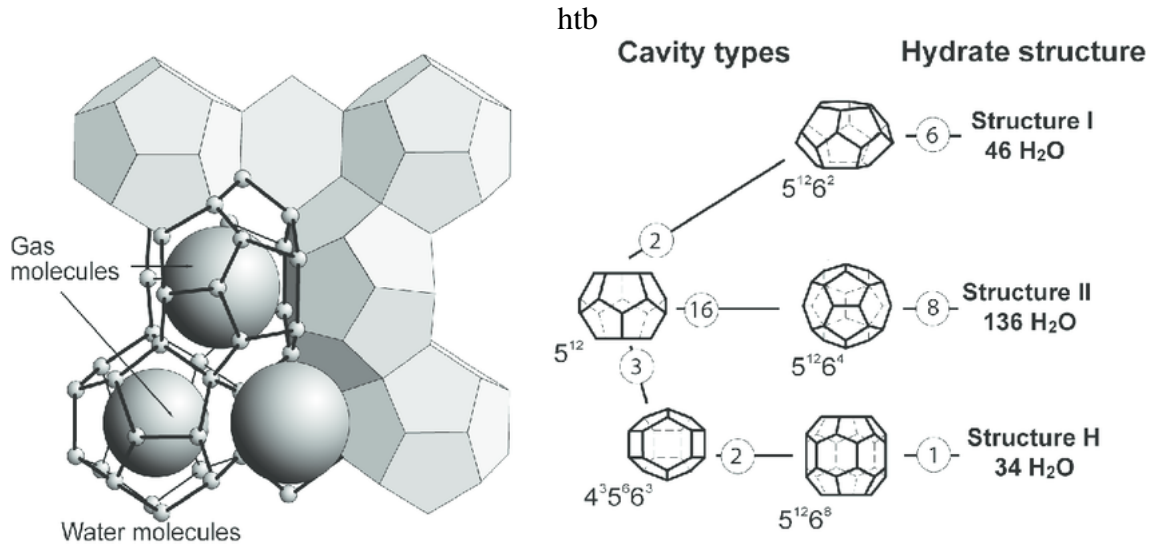
Figure 1.1 ( left ) Gas hydrate with structure I (sI): the small spheres are water molecules forming hydrogen-bonded cavities and the large spheres are the gas molecules. The gray polyhedrons represent the cavities generated by the water molecules. ( right ) Typically, the types and numbers of water cavities correspond to one of the three following structures of gas hydrate: sI, sII, and sH. The circled numbers are the numbers of such water cavities which are used to form the corresponding hydrate structure. [Picture from Ref. (Schulz and Zabel, 2006)]
