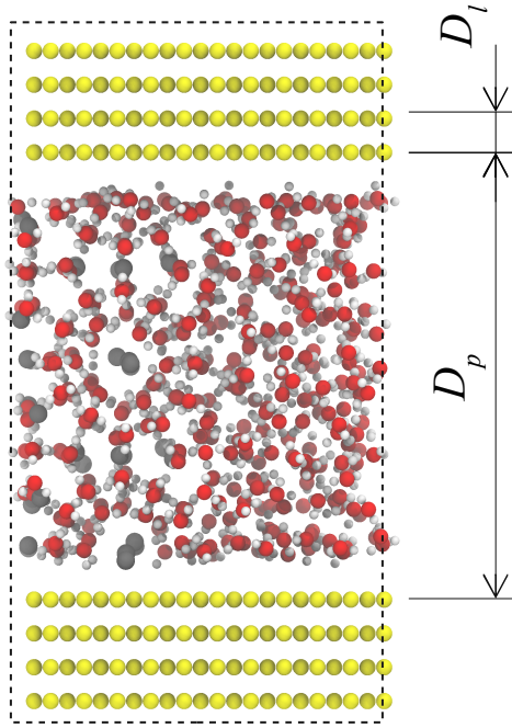
Figure 4.1 (color online) Molecular configuration of the confined coexisting phases (i.e., methane hydrate + liquid water) considered in this work. The red and white spheres are the oxygen and hydrogen atoms of water, respectively. The gray spheres are the methane molecules which are inside the hydrogen-bonded cages formed by water molecules. The yellow spheres are the solid atoms in the pore walls. The two component system is confined in a pore with a width D_p made of layers of solid particles distributed according to a square structure. Each pore surface is made of 4 layers separated by a distance D_l = 0.2159 nm so that the total pore wall thickness is 0.7558 nm. Inside the porosity, methane hydrate is located in the region y < 0 (left side) and liquid water in the region y > 0 (right side). In this specific configuration, the pore size is D_p = 2.8554 nm which corresponds to 2 \times 2 \times 2 unit cells of bulk sI methane hydrate (the lattice parameter of methane hydrate is u = 1.1877 nm). Periodic boundary conditions are used along the x , y , and z directions. The dimensions of the simulation box (defined by the dashed lines) are L_x = L_y = 2.3754 nm and L_z = 4.3670 nm.
