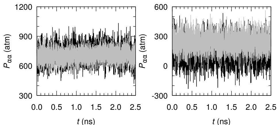
Figure 4.7 Normal (black line), P_N = P_{zz} , and parallel (gray line), P_T = \frac{1}{2} (P_{xx} + P_{yy}) , pressure components of methane hydrate ( left ) and liquid water ( right ) in a slit pore D_p = 9.9816 nm as a function of time, t , in canonical ensemble MD simulation at T = 290 K. The dimensions of the simulation box are: L_x = L_y = 2.3754 nm and L_z = 41.4932 nm.
