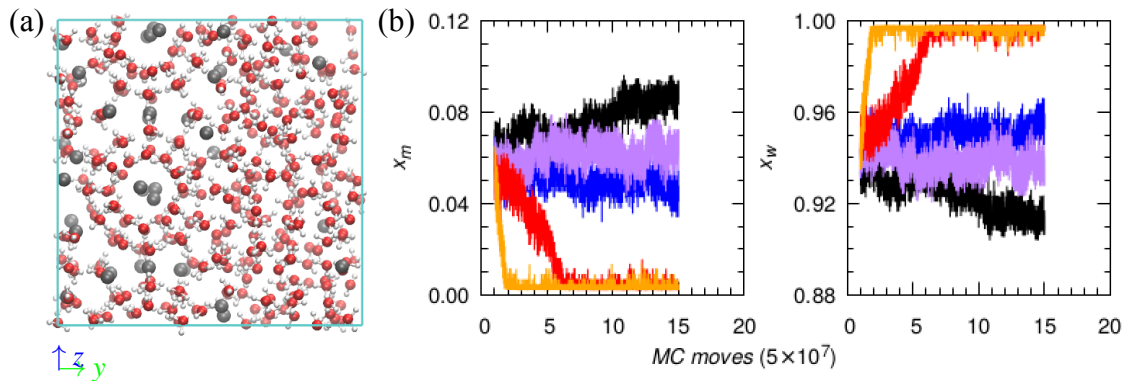
Figure 3.8 (color online) Determination of the phase transition temperature between methane hydrate and liquid phases using the direct coexistence method. (a) Starting from a methane hydrate coexisting with the liquid phase, several Monte Carlo simulations in the Grand Canonical ensemble ( \mu VT ) at different temperatures and chemical potentials are performed (chemical potentials are chosen so that the pressure is P = 100 atm). The red and white spheres are the oxygen and hydrogen atoms of water while the grey spheres are the methane molecules. The dimensions of the simulation box are: L_x = L_y = L_z = 2.3754 nm. Molecules with y < 0 (left region) and y > 0 (right region) belong to the methane hydrate and liquid phases, respectively. If the temperature is lower than the melting point T_m , the liquid disappears as methane hydrate forms. In contrast, if the temperature is larger than T_m , the methane hydrate melts and is replaced by the liquid. (b) Methane (left) and water (right) mole fractions during the different GCMC simulation runs: T = 260 K (black), 270 K (purple), 280 K (blue), 290 K (red), and 300 K (orange). The x -axis, which indicates progress along the GCMC simulation, is expressed as a number of attempted MC moves where one move is a molecule translation, rotation, insertion or deletion.
