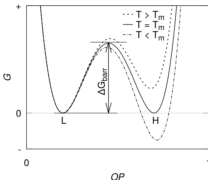
Figure 1.6 Free energy, G , as a function of the normalized order parameter, OP , using biased molecular simulations. Liquid water (L) exhibits a small order parameter, while methane hydrate (H) exhibits a large order parameter. At the melting temperature, T = T_m , methane hydrate coexists with liquid water (i.e., the free energies of liquid water and methane hydrate are equal). At high temperature, T > T_m , liquid water is stable (i.e., the free energy of liquid water is smaller than that of methane hydrate). At low temperature, T < T_m , methane hydrate is stable (i.e., the free energy of methane hydrate is smaller than that of methane hydrate). The free energy barrier between liquid water and methane hydrate, \Delta G_{barr} , upon formation is also shown.
