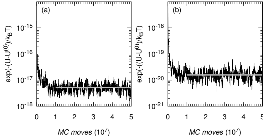
Figure A.2 Intermolecular potential energy U of the zero-occupancy methane hydrate along the canonical ensemble MC simulation at T = 250 K and P = 100 atm (black line) (only the harmonic potential U_{A^*} is considered in the acceptance probability): (a) TIP4P/2005 water model; (b) TIP4P/Ice water model. Note that the figure shows \exp\left(-\frac{(U - U^{(0)})}{k_B T}\right) where U^{(0)} is the potential energy of the reference lattice system. The gray horizontal line is the canonical ensemble averaged value, \left\langle \exp\left(-\frac{(U - U^{(0)})}{k_B T}\right) \right\rangle_{NVT} . All energies are normalized to the thermal energy k_B T .
