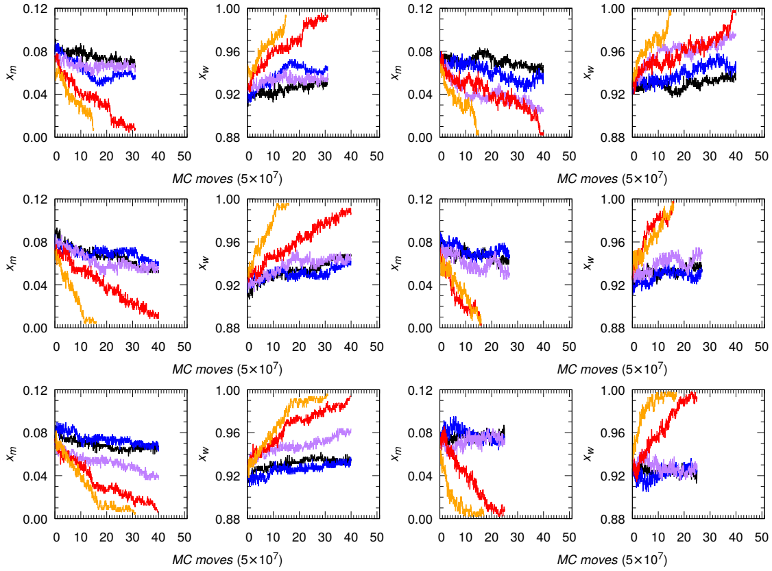
Figure B.6 Same as Figure 4.3 but for the decreased LJ energy parameter (two left panels: one for methane, x_m , and another one for water, x_w ): \epsilon' = 1/2\epsilon (top panels), 1/3\epsilon (center panels), and 1/4\epsilon (bottom panels); and for the increased LJ energy parameters (two right panels: one for methane, x_m , and another one for water, x_w ): \epsilon' = 2\epsilon (top panels), 3\epsilon (center panels), 4\epsilon (bottom panels). \epsilon' is for the pair of atoms between solid walls and hydrate/liquid phase.
