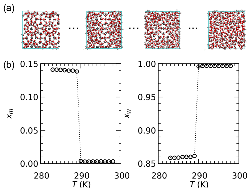
Figure 3.9 (color online) Determination of the phase transition temperature between the methane hydrate and liquid phases using hyper parallel tempering Monte Carlo simulations. (a) Several replicas M = 16 of the system are considered in parallel. Each replica is at different temperatures and chemical potentials (the latter are chosen so that the pressure of the system is P = 100 atm). The temperature ranges from 283 K to 298 K with a temperature difference \Delta T = 1 K. For each replica, a regular grand canonical Monte Carlo simulation consisting of molecule translation, rotation, insertion, and deletion moves are performed. In addition to these conventional moves, replicas at two different temperature/chemical potentials sets are swapped with a probability given from the ratio of the Boltzmann factors in the Grand Canonical ensemble ( see text ). The red and white spheres are the oxygen and hydrogen atoms of water while the grey spheres are the methane molecules. The dimensions of the simulation box are: L_x = L_y = L_z = 2.754 nm. (b) Average methane (left) and water (right) mole fraction as a function of temperature as estimated from the different replicas considered in the hyper parallel tempering simulation.
