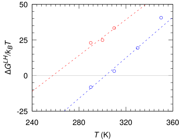
Figure 4.10 (color online) Free energy difference, \Delta G^{LH} , between methane hydrate and liquid water as a function of temperature, T . The blue circles are for bulk methane hydrate and the red circles are for confined methane hydrate in a pore D_p = 2.8554 nm. The blue dashed line is a linear fit for bulk methane hydrate while the red dashed line is a linear fit for confined methane. These fits lead to T_m^{bulk} = 302 K and T_m^{pore} = 257 K for D_p = 2.8554 nm. The free energy is normalized using the thermal energy, k_B T .
