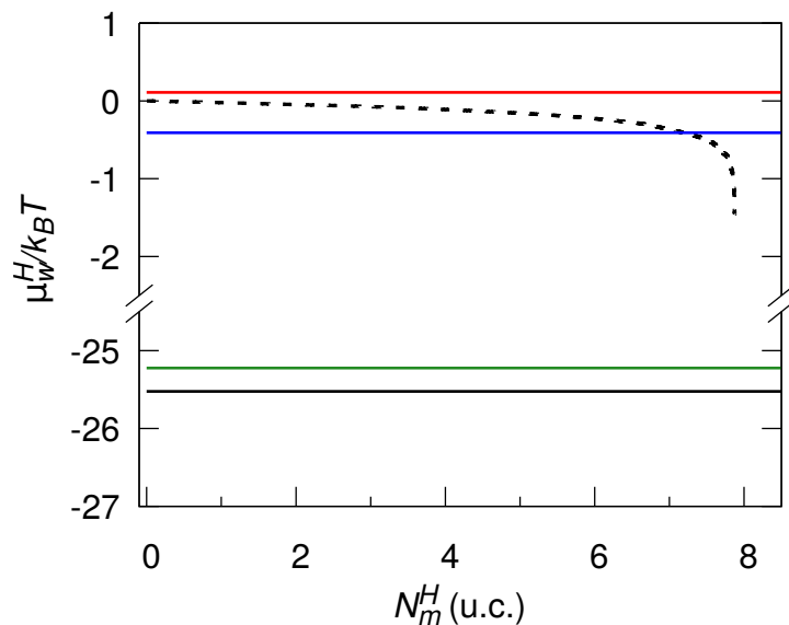
Figure A.6 Contributions to the chemical potential of water in methane hydrate \mu_w^H(x_m)/k_B T at T = 250 K and P = 100 atm. \mu_w^H(x_m)/k_B T = \mu_w^H(x_m = 0)/k_B T + \Delta\mu_w^H(x_m)/k_B T where \mu_w^H(x_m = 0)/k_B T (black solid line) is the chemical potential of water in zero-occupancy methane hydrate and \Delta\mu_w^H(x_m)/k_B T (black dashed line) is the contribution due to the methane occupancy. \mu_w^H(x_m = 0)/k_B T = A_w(x_m = 0)/N_w k_B T + A_{disorder}/N_w k_B T + PV/N_w k_B T where A_w(x_m = 0)/k_B T is the contribution from the Helmholtz free energy of zero-occupancy methane hydrate using Einstein molecule approach (green solid line), A_{disorder} is the proton disorder correction (blue solid line), and PV/N_w k_B T term (red solid line). The data shown here are for the TIP4P/Ice water model (similar qualitative results were obtained for the TIP4P/2005 water model). Note the use of a broken axis along the y-axis.
