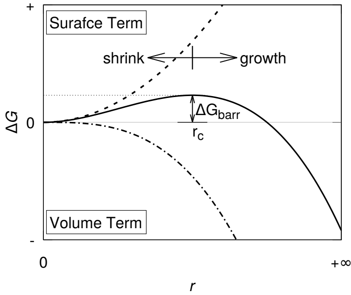
Figure 1.4 Free energy (solid line), \Delta G , as a function of nucleus radius, r , in the formation process of methane hydrate. Formation can be described as the interplay between the hydrate–liquid surface free energy (surface term corresponding to the dashed line), \Delta G_S , and the free energy difference between liquid water and methane hydrate (volume term corresponding to the dot dashed line), \Delta G_V . The critical radius, r_c , and the corresponding free energy barrier, \Delta G_{barr} , are also shown in this figure. If the nucleus radius is larger than the critical radius, i.e., r > r_c , the nucleus keeps growing to form methane hydrate (“growth”). For r < r_c , the nucleus melts into liquid water (“shrink”).
