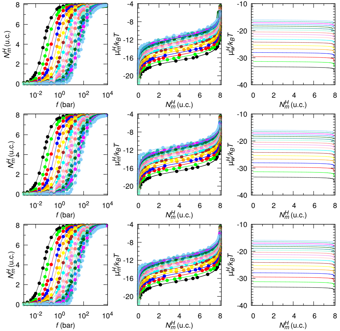
Figure A.4 Determination of the chemical potential of methane and water in methane hydrate using TIP4P/2005 water in combination with OPLS-UA methane model: (1) methane occupancy N_m^H (the number of molecules per unit cell) versus fugacity f (left panel), (2) chemical potential of methane \mu_m^H/k_B T = \ln \frac{f \Lambda^3}{k_B T} (center panel) and water \mu_w^H/k_B T = \mu_w^{(0)}/k_B T - \frac{1}{N_w k_B T} \int_{-\infty}^{\mu_m} N_m d\mu_m (right panel) versus N_m^H . In the left panel, the temperature increases from 180 to 350 K ( \Delta T = 10 K) (from left to right); In the center and right panels, temperature increases from 180 to 350 K ( \Delta T = 10 K) (from top to bottom). The pressures are P = 1 atm (top), 10 atm (middle), and 100 atm (bottom). All chemical potentials are normalized to the thermal energy, k_B T .
