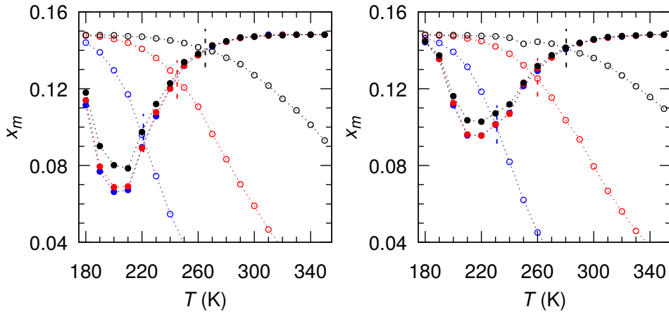
Figure 3.6 (color online) Equilibrium number of methane, x_m(\mu_m^V = \mu_m^H) (empty circles) and x_m(\mu_w^L = \mu_w^H) (filled circles), as a function of temperature, T , at P = 1 (blue), 10 (red), 100 (black) atm. The corresponding interpolation cross point, x_m(\mu_m^V = \mu_m^H) = x_m(\mu_w^L = \mu_w^H) , indicating the liquid water-methane hydrate-methane vapor (L–H–V) equilibrium temperature and methane composition at the given pressure. The left and right panels are for TI4P/2005 and TIP4P/Ice water models, respectively.
