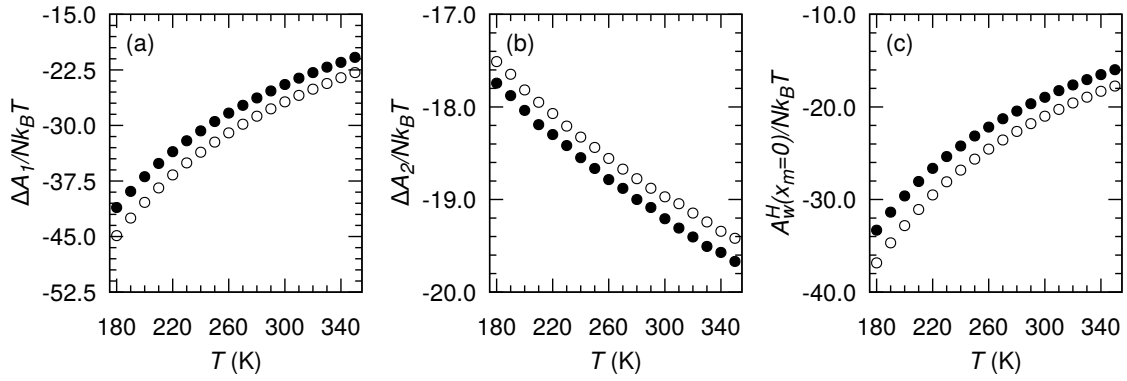
Figure 3.4 Free energy changes \Delta A_1 (a) and \Delta A_2 (b) and free energy A_w^H(x_m = 0) of the zero-occupancy methane hydrate (c) as a function of temperature T (all data reported here are for P = 100 atm). The empty and closed circles are for the TIP4P/Ice and TIP4P/2005 water models, respectively. Free energies are normalized to the total thermal energy Nk_B T . \Delta A_1 = A_{B^*} - A_{A^*} is the free energy difference between the non-interacting and interacting Einstein molecules (corresponding to the zero-occupancy methane hydrate). \Delta A_2 = A_{C^*} - A_{B^*} is the free energy difference between the interacting Einstein molecule and the zero-occupancy methane hydrate. Except for the zero-occupancy methane hydrate in (c), all systems are constrained with one of their molecules having a fixed reference position.
