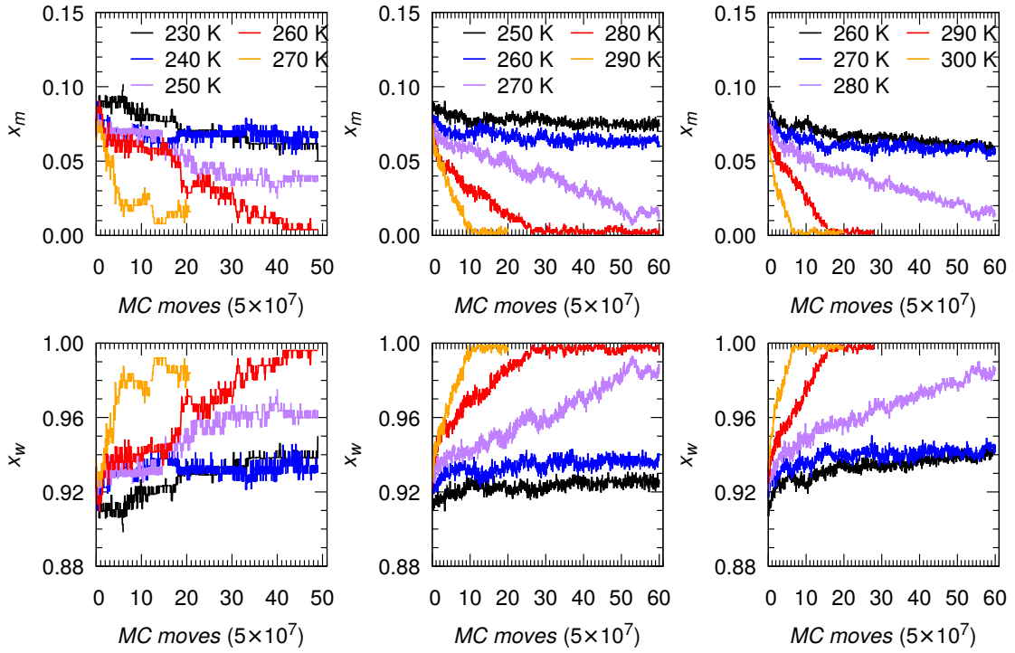
Figure 4.4 (color online) Melting temperature, T_m^{pore} , of confined methane hydrate/liquid water for different pore widths: D_p = 1.6677 nm ( left panels ), 5.2308 nm ( center panels ), and 7.6062 nm ( right panels ) as obtained using the direct coexistence method. The methane ( x_m , top panels ) and water ( x_w , bottom panels ) mole fractions during the different GCMC simulation runs are shown: T for each pore size is indicated using different colors (see figure legend). The x -axis, which indicates progress along the GCMC simulation, is expressed as a number of attempted MC moves where one move is a molecule translation, rotation, insertion or deletion. T_m^{pore} of confined methane hydrate for different D_p are summarized in Table 4.1. For bulk methane hydrate, we reported T_m^{bulk} = 285 \pm 5 K at P = 100 atm using the direct coexistence method in Chapter 3.
