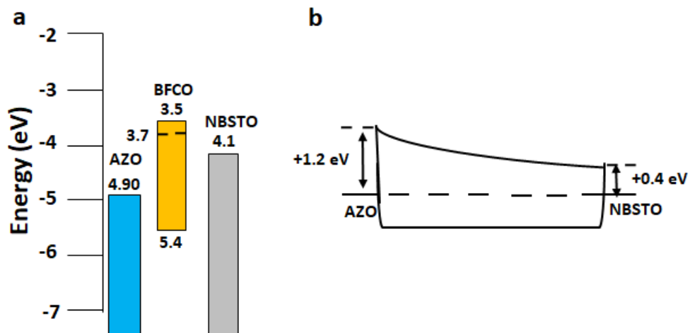
Fig.4.44 Schema of the energy levels of the device AZO/BFCO/NBSTO
