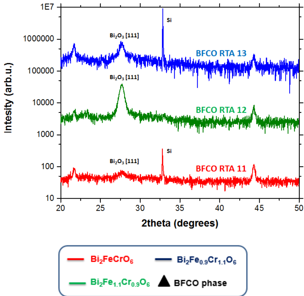
Fig.3.13: XRD spectra taken for BFCO films with different stoichiometry and annealed by RTA under N_2/O_2 : 70/30
