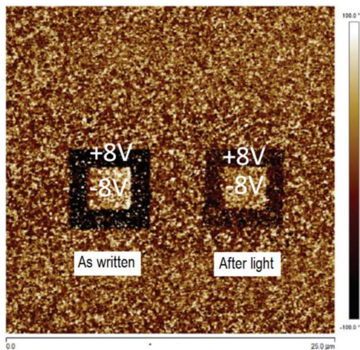
Figure 4.31. PFM poling images before and after exposure to 365 nm light
