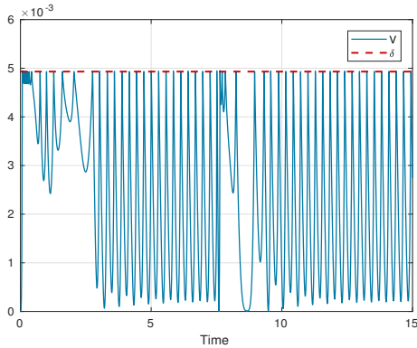
(a) The PLF of the SISO system and the threshold \delta .
